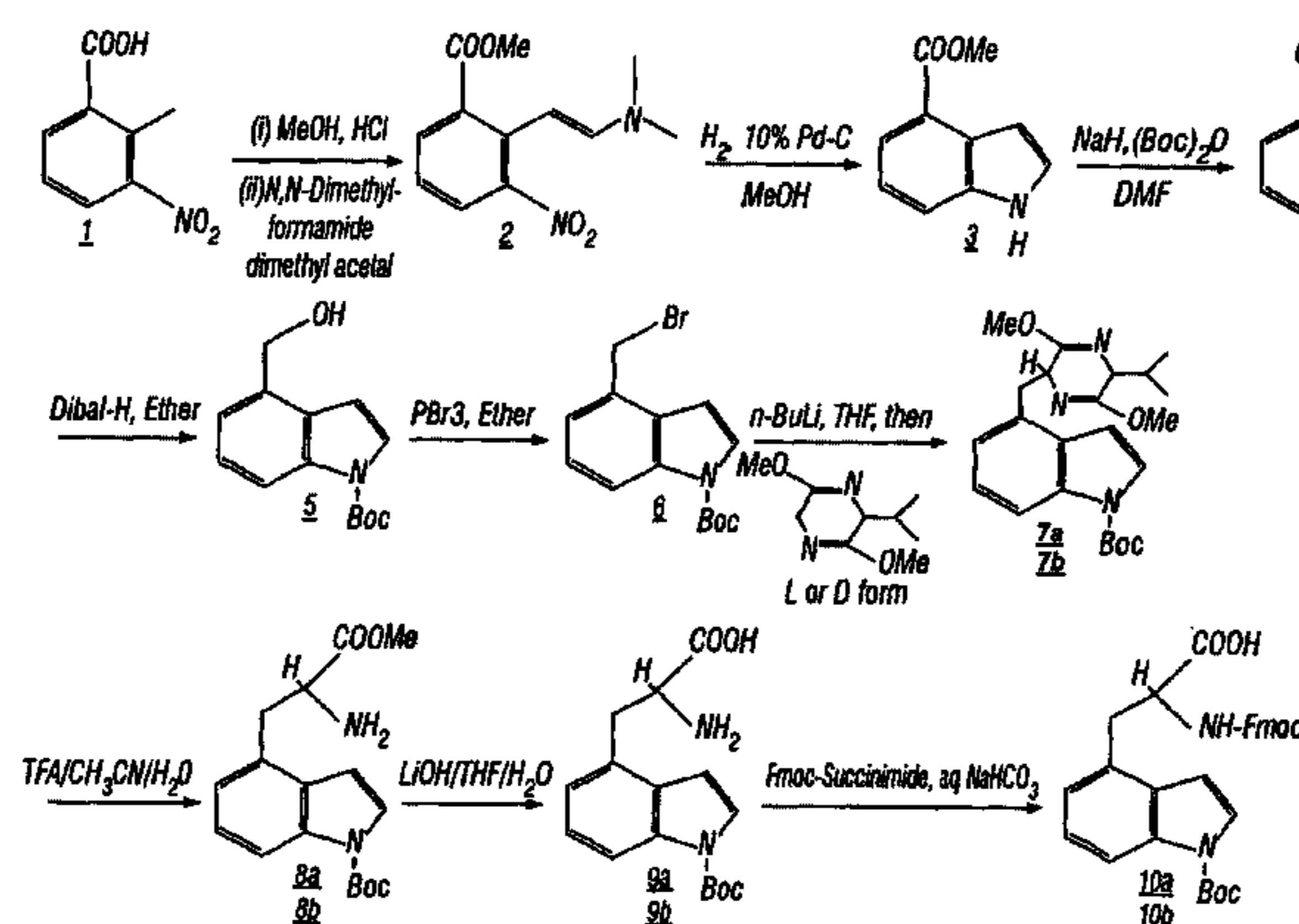
Synthesis of (DL)-Neo-Tryptophan
