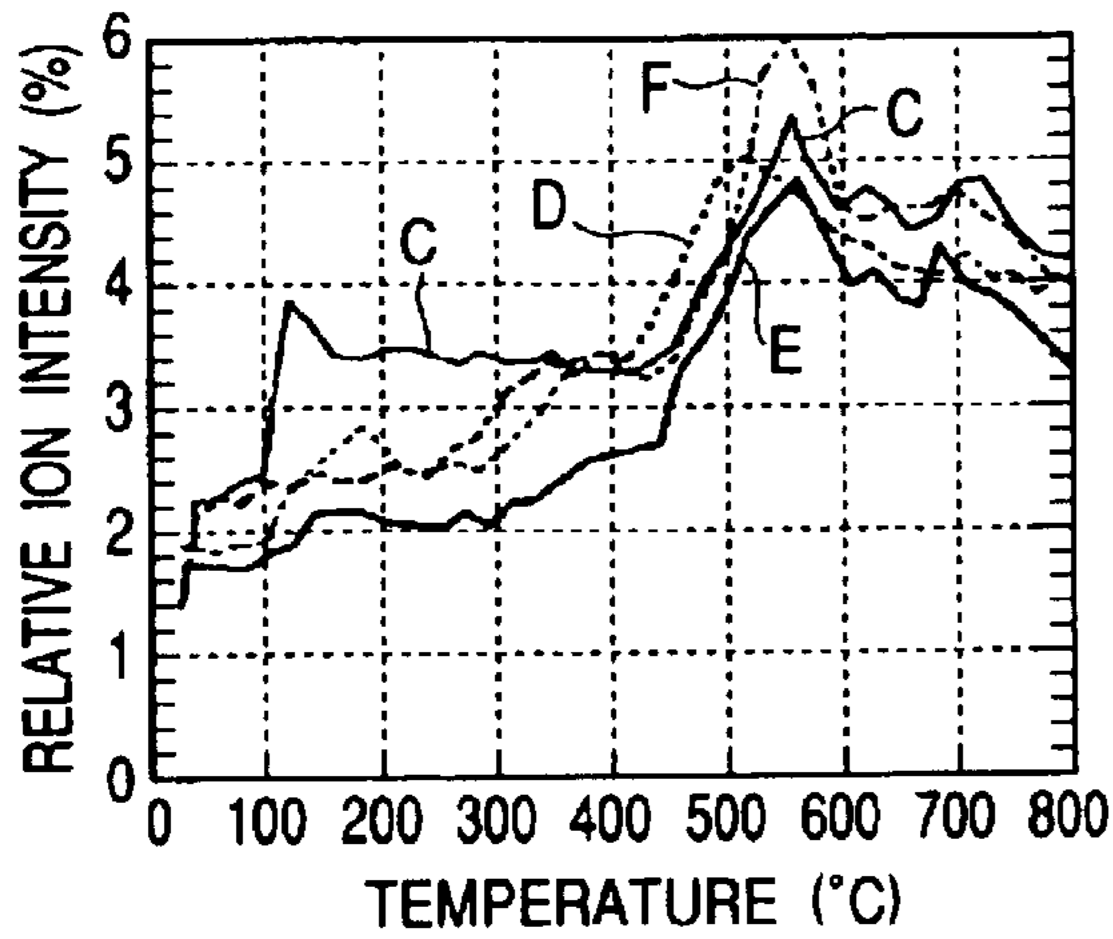
THERMAL DISSOCIATION OF HYDROGEN, Ar-H m/z=41
