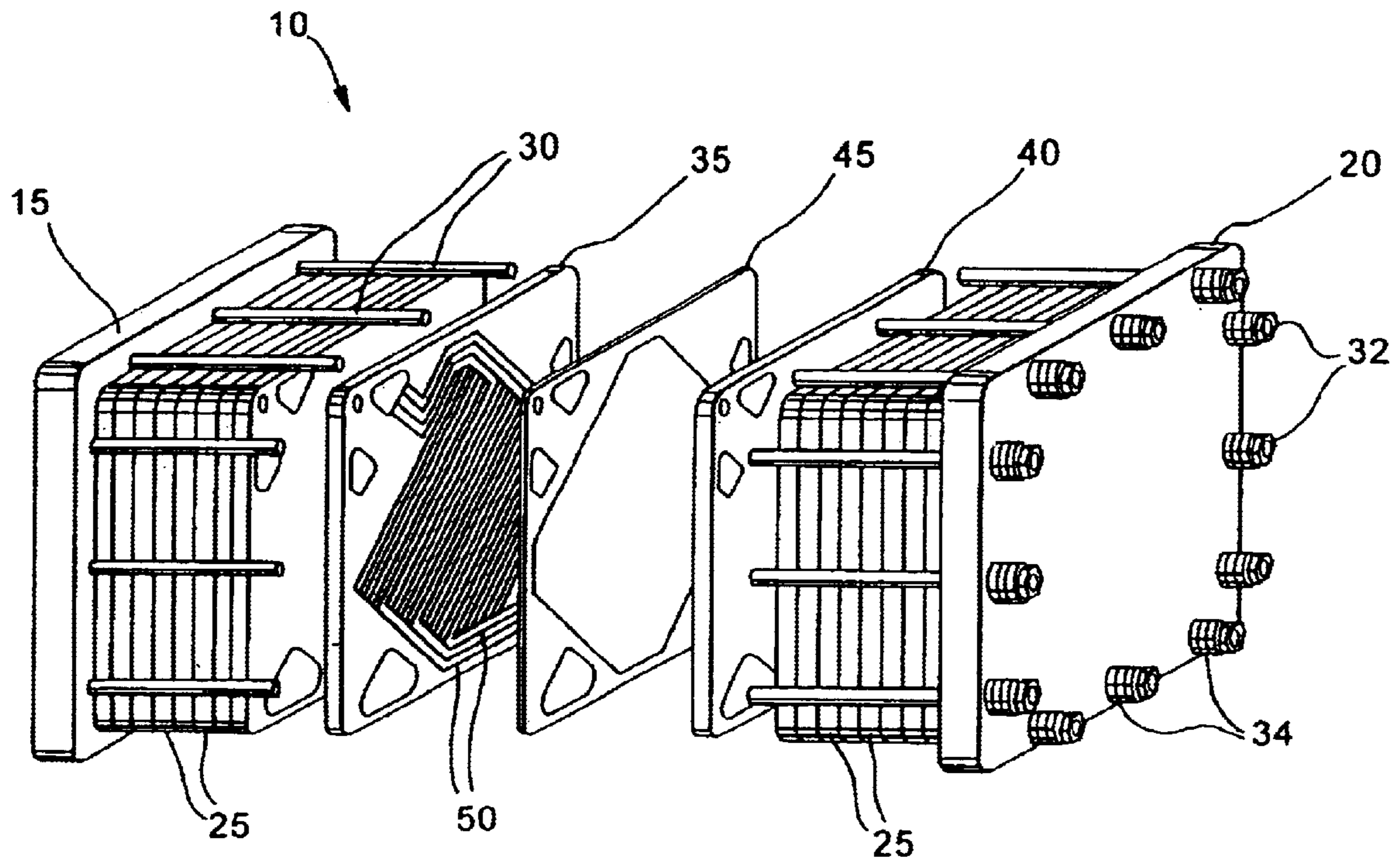
FIG. 1 PRIOR ART
