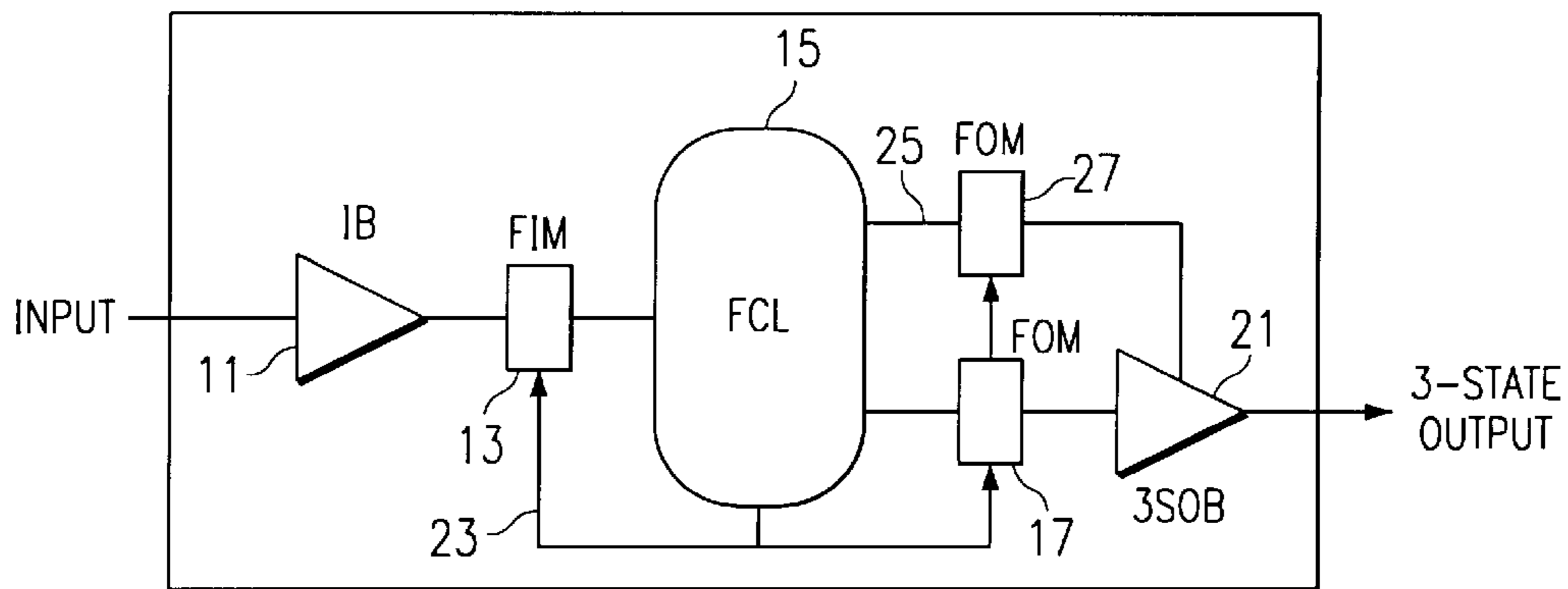
FIG. 2 (PRIOR ART)
