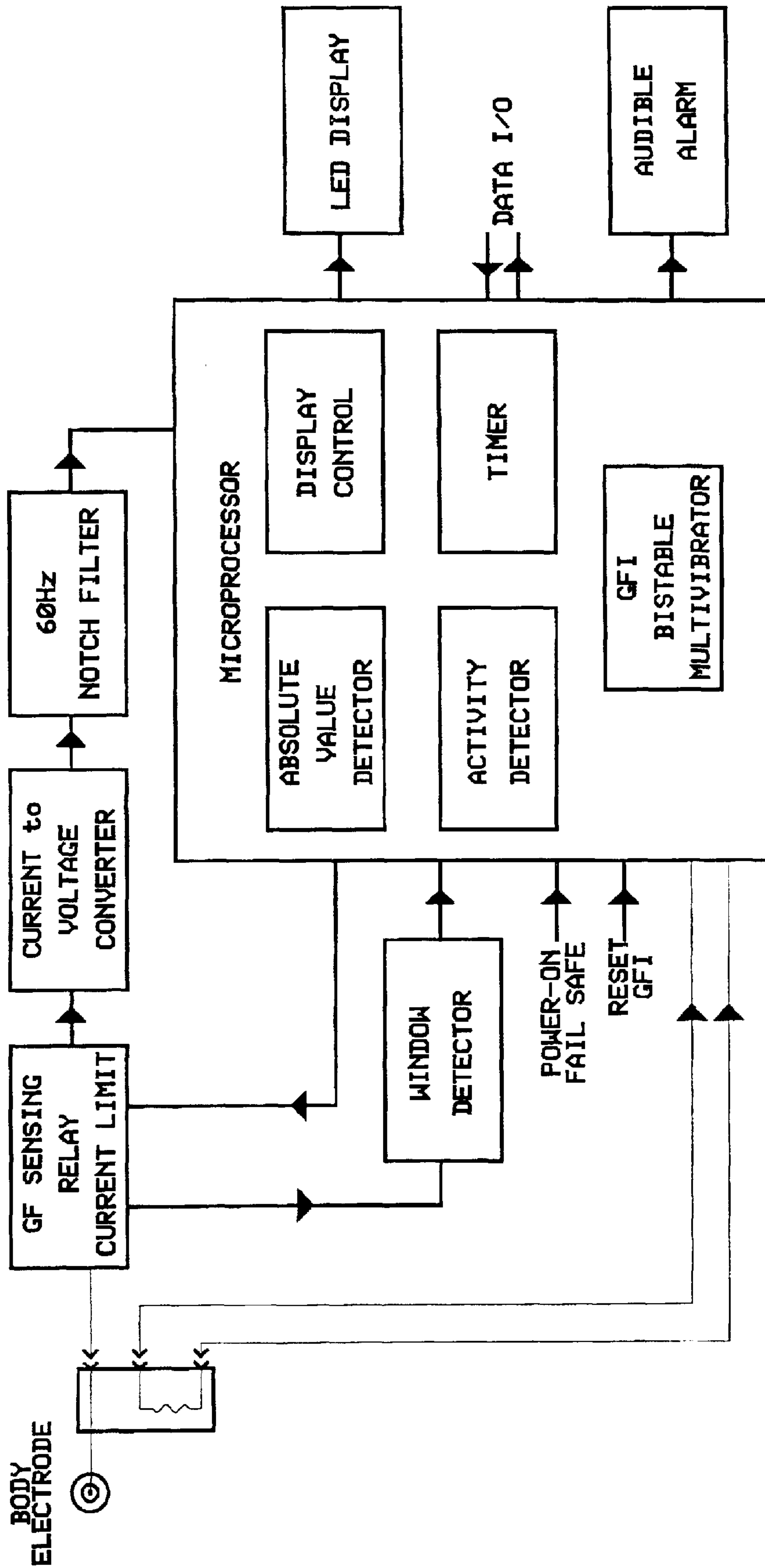
FIGURE 4 BLOCK DIAGRAM
