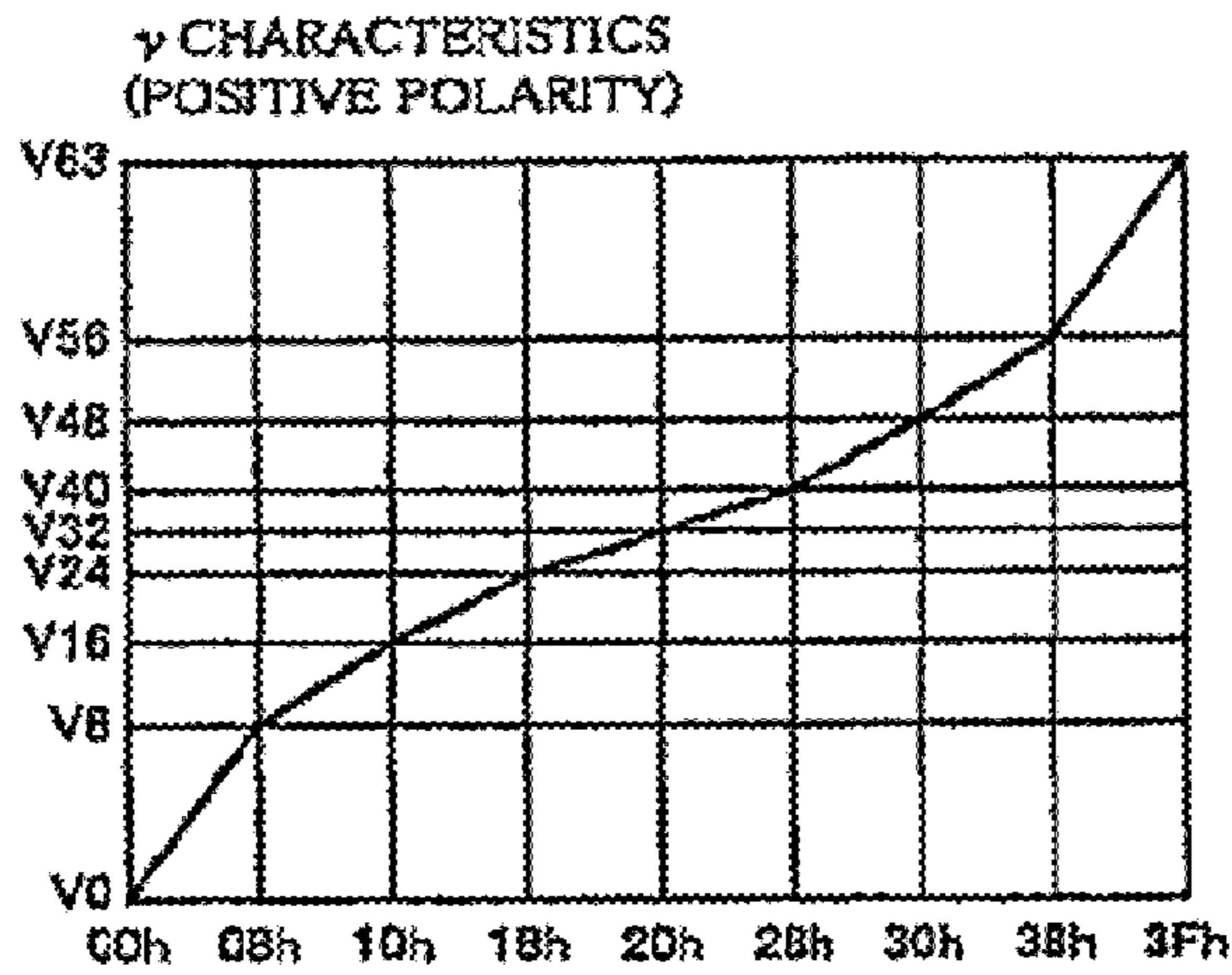
FIG. 26 (a) CONVENTIONAL ART
