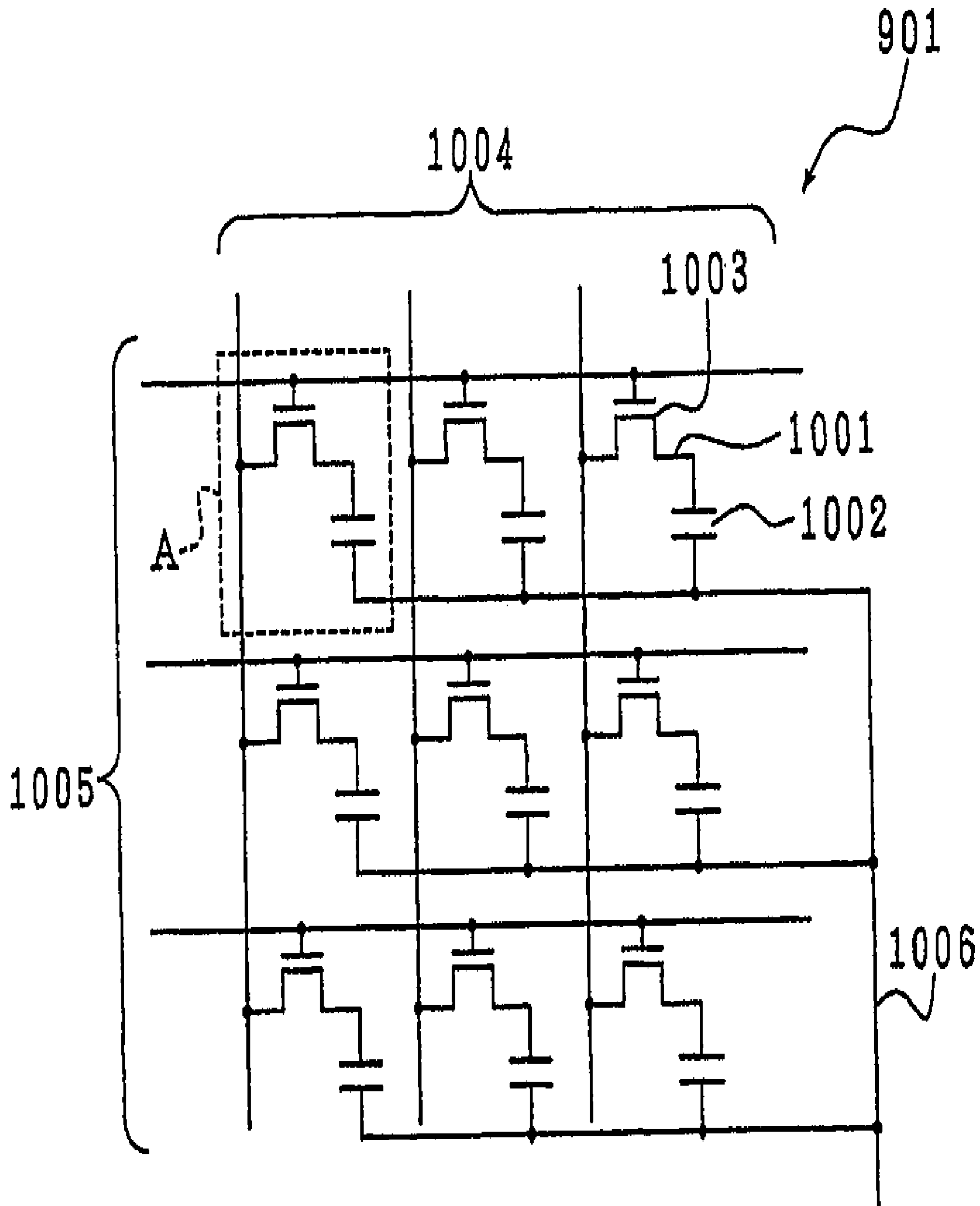
FIG. 14 CONVENTIONAL ART
