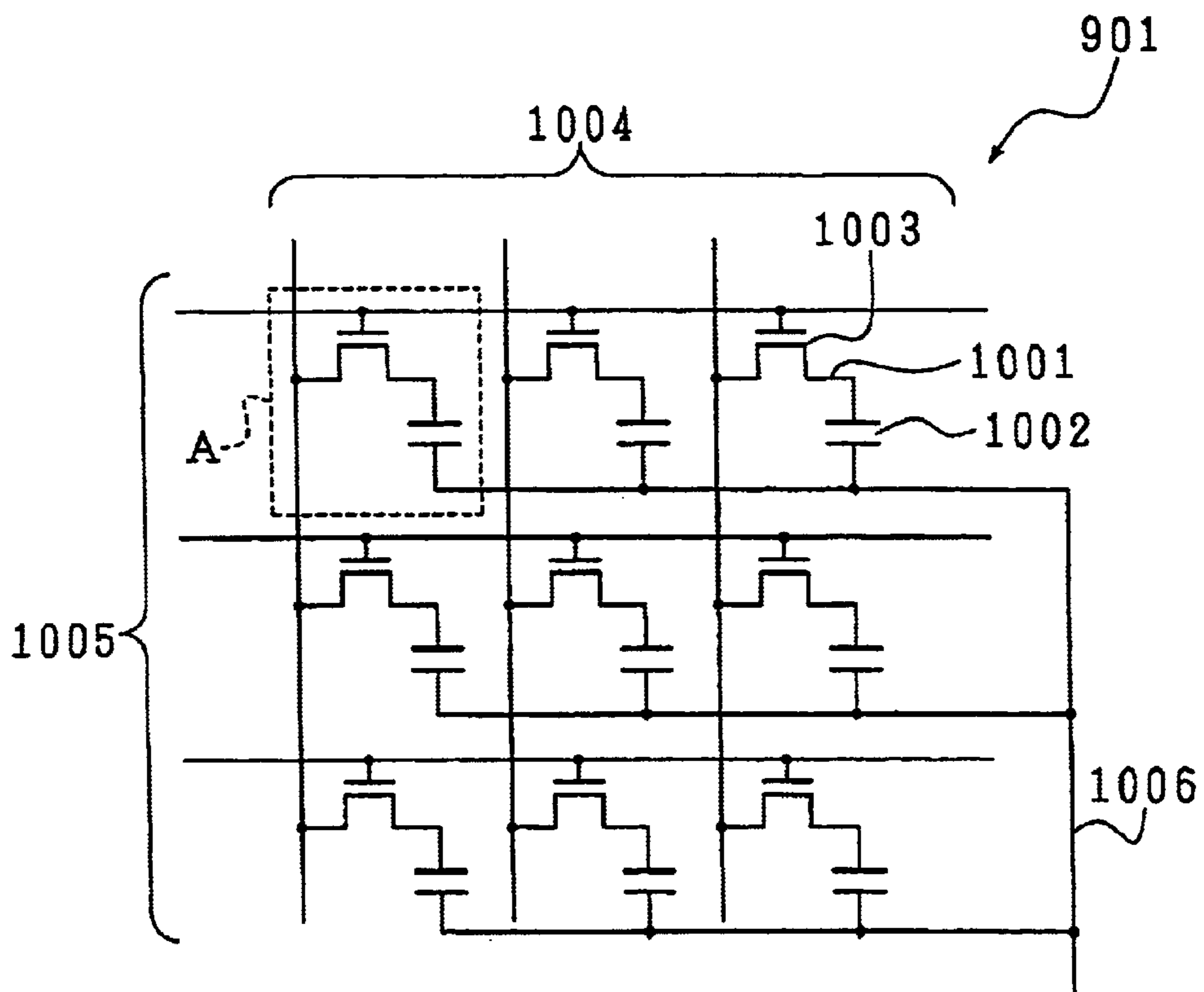
FIG. 14 CONVENTIONAL ART
