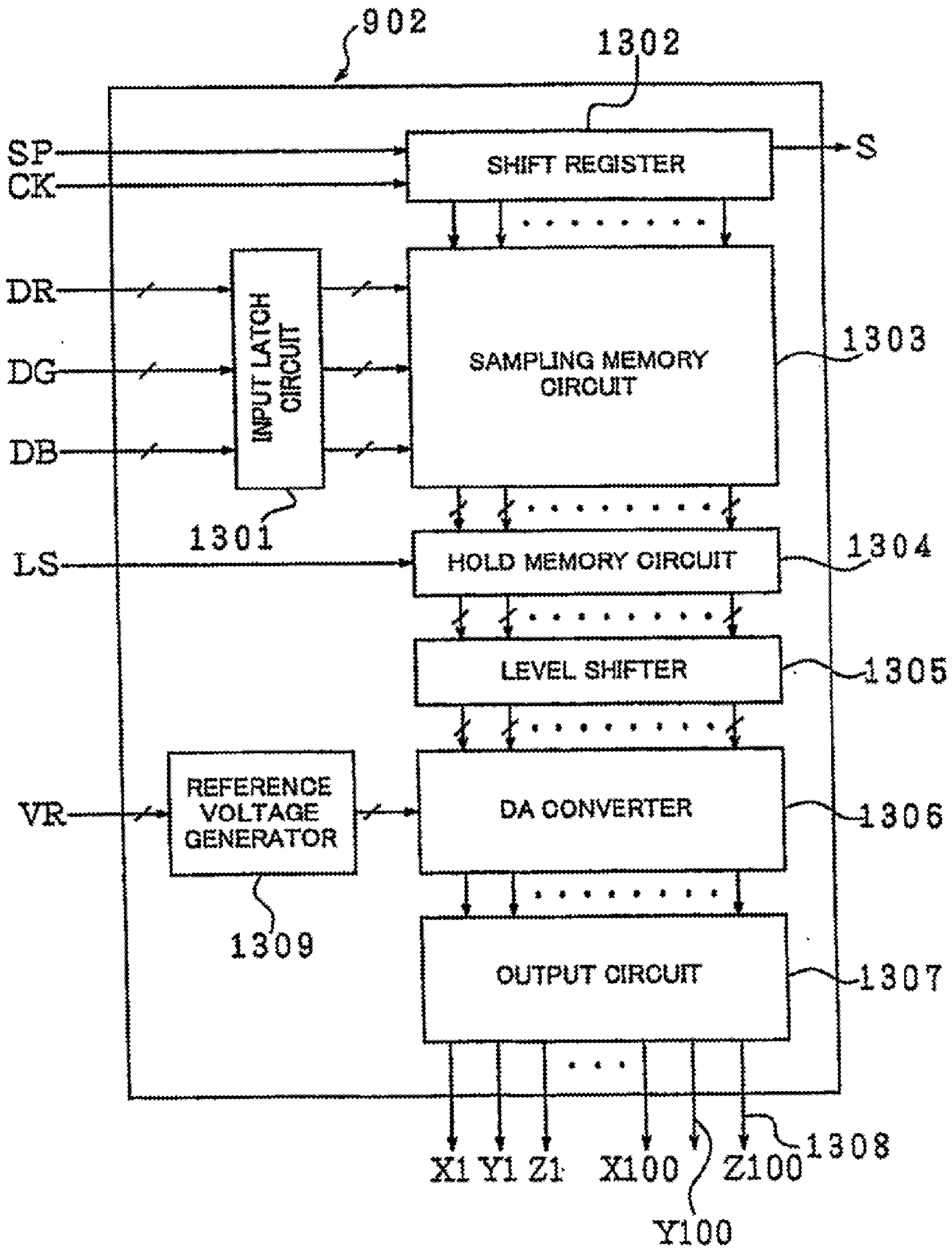
FIG. 17 CONVENTIONAL ART
