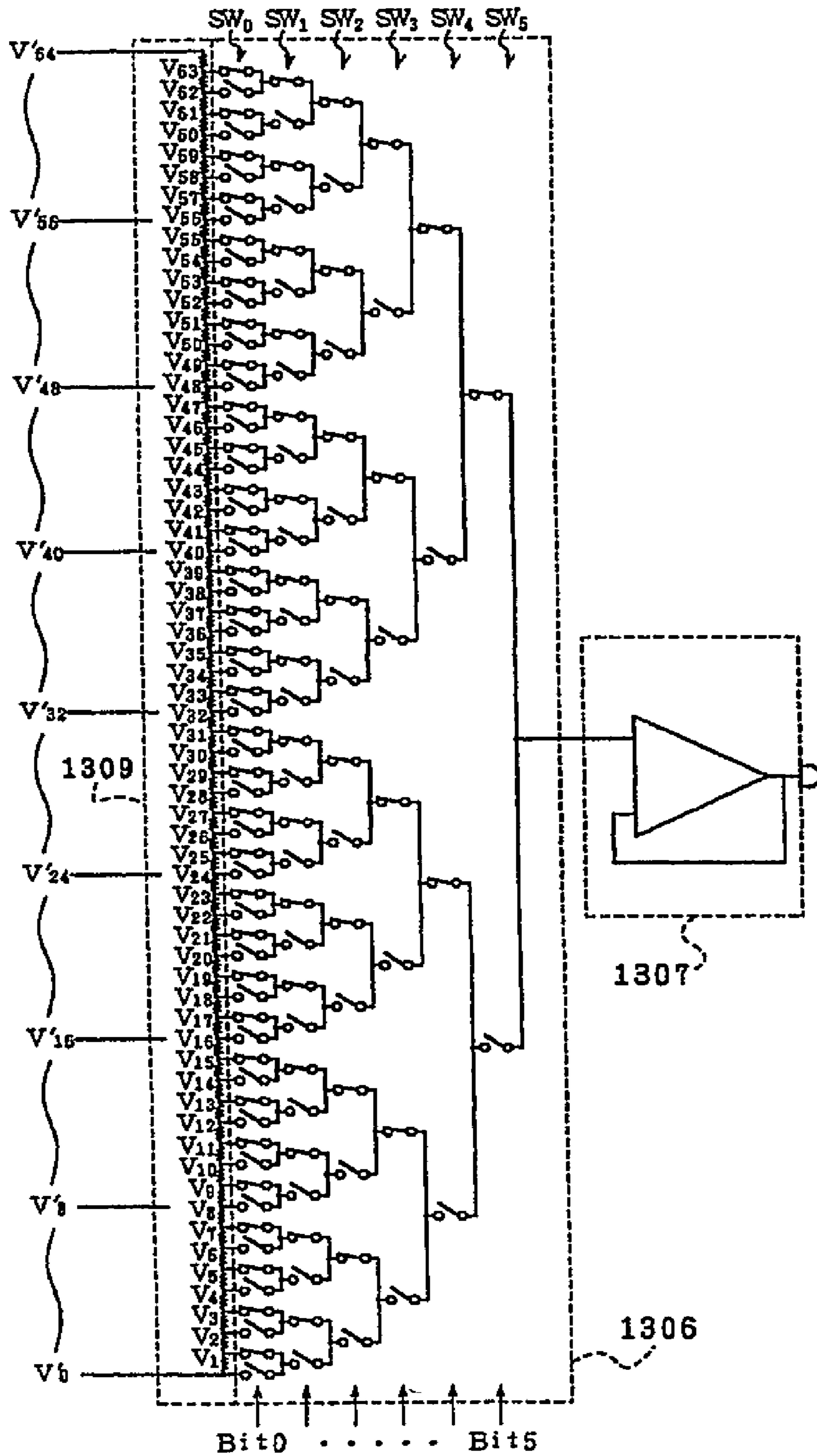
FIG. 22 CONVENTIONAL ART
