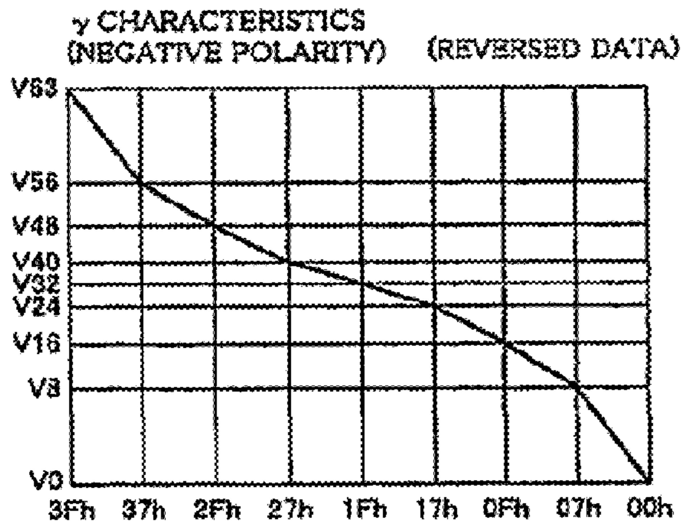
FIG. 26 (c) CONVENTIONAL ART
