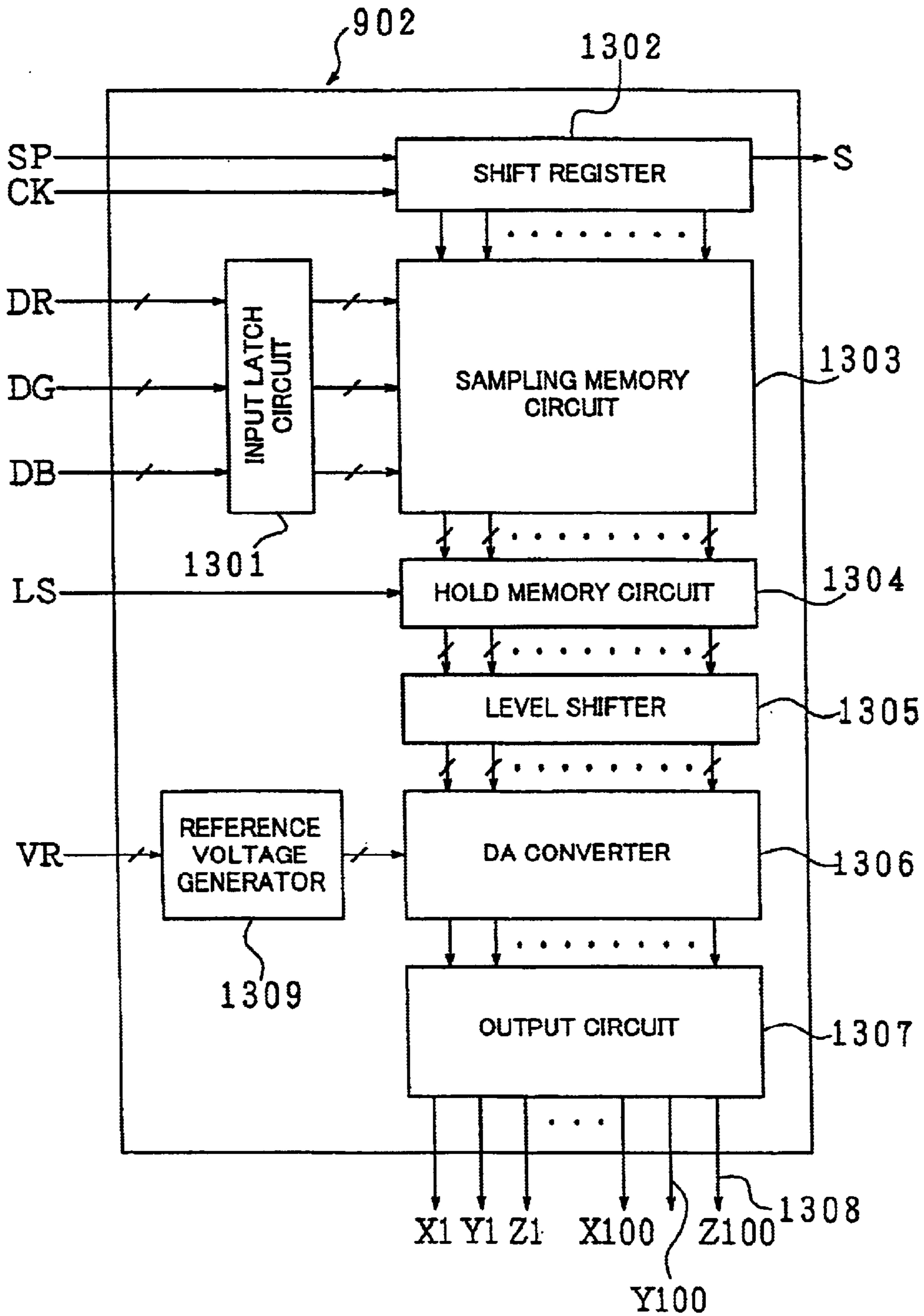
FIG. 17 CONVENTIONAL ART
