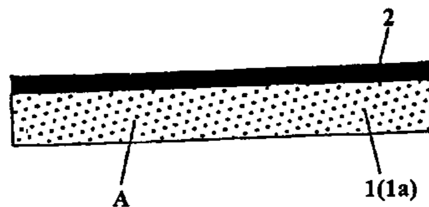
1... low refractive index member 1a... silica aerogel 2... electrically conductive transparent film
