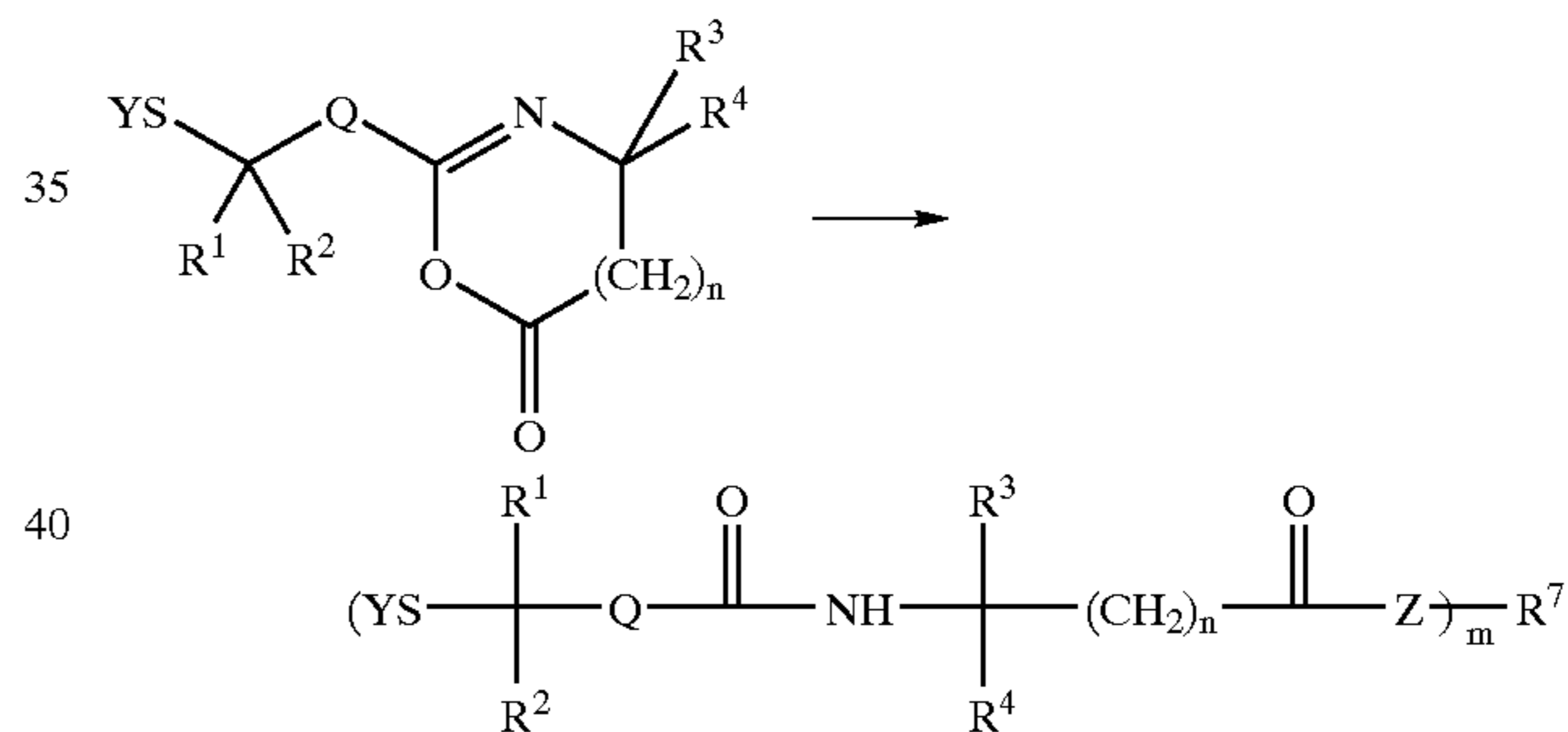
Scheme II
