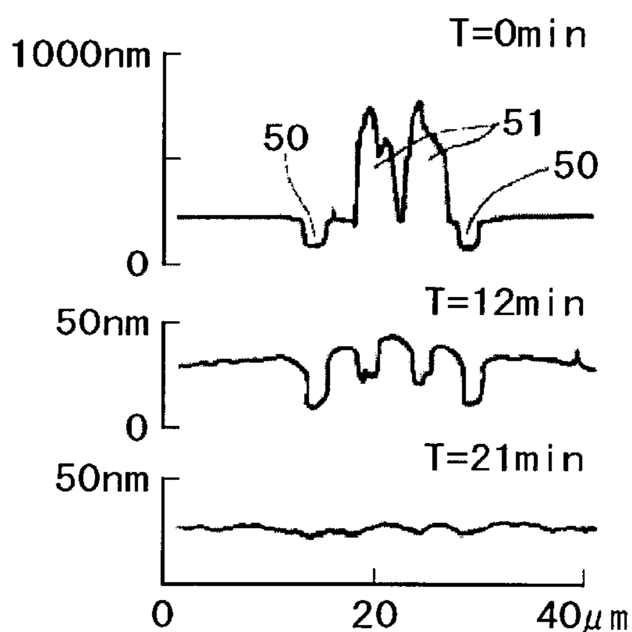
POLISHING ON FILLED-UP SURFACE
