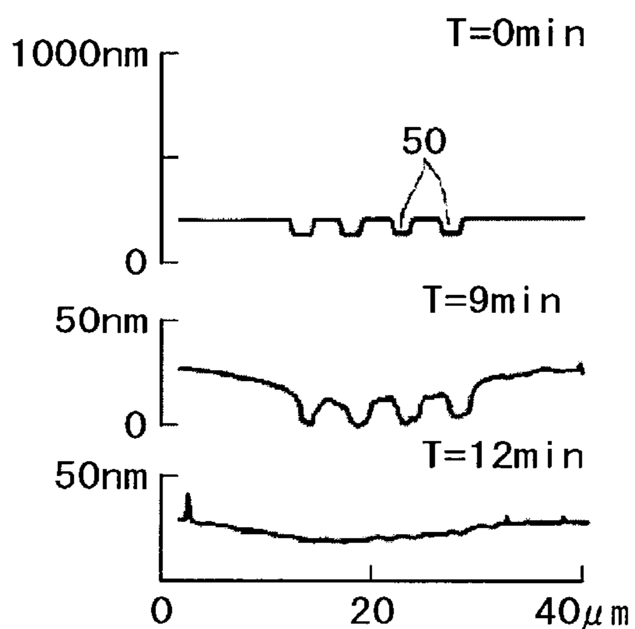
POLISHING ON SURFACE HAVING DEPRESSIONS
