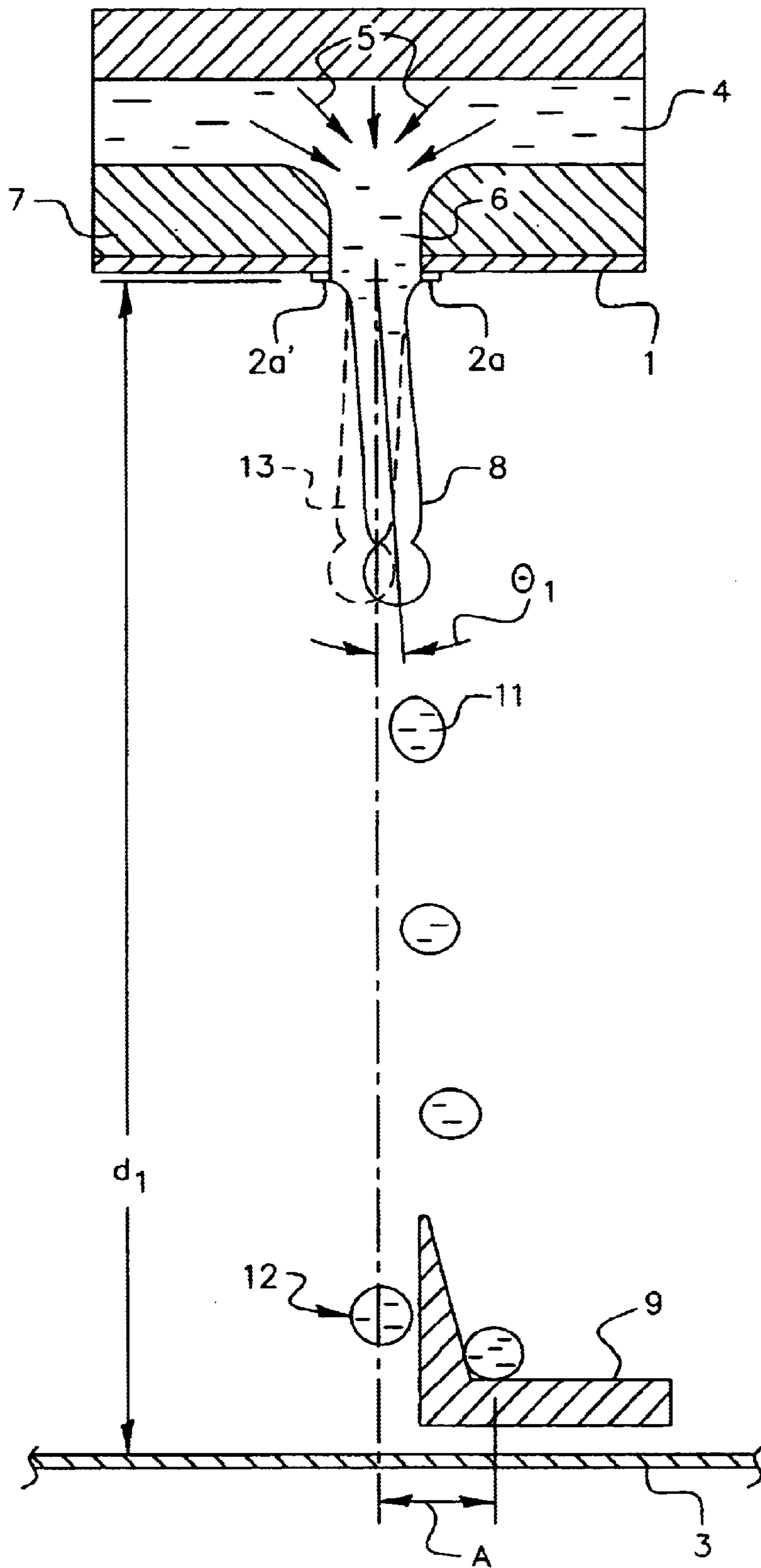
FIG. 2 (PRIOR ART)
