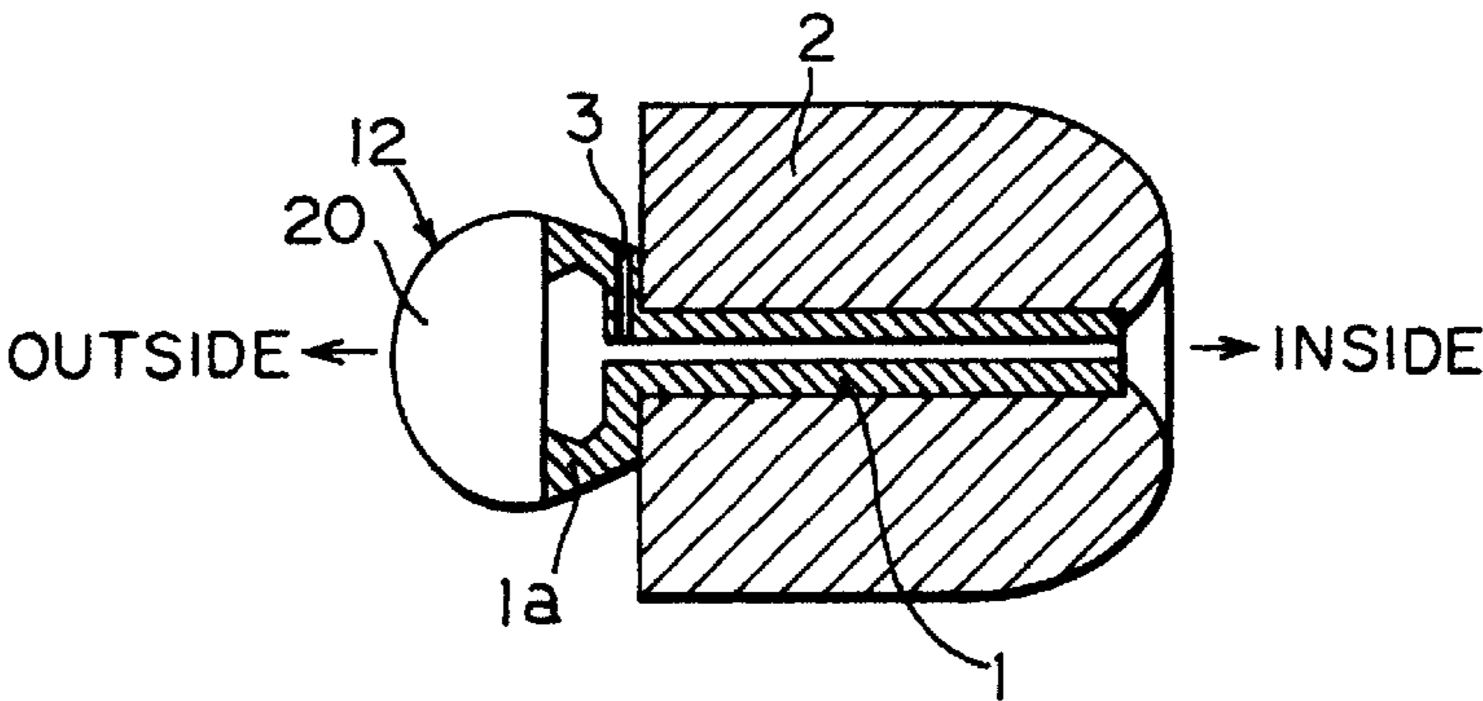
FIG. 1 PRIOR ART
