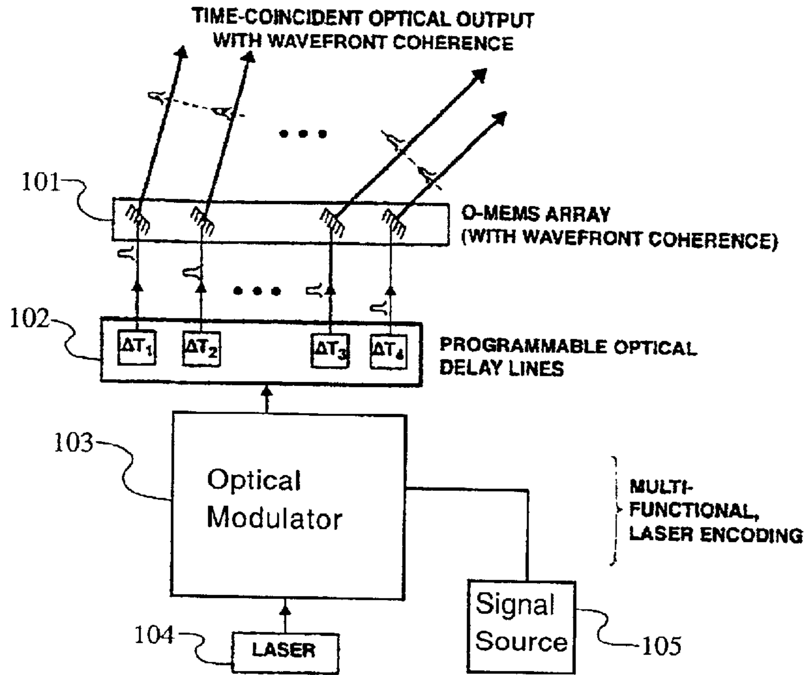
FIG. 1 (prior art)
