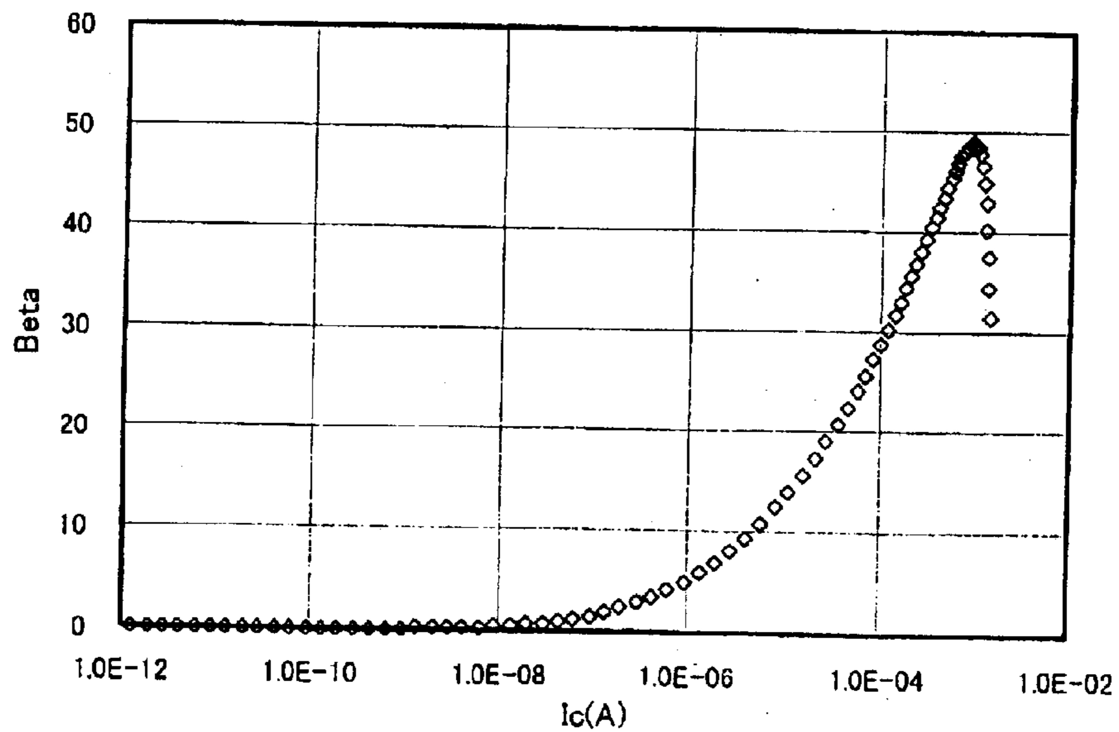
Current multiplication factor of SiGe 0.268 C 0.0091 HBT
