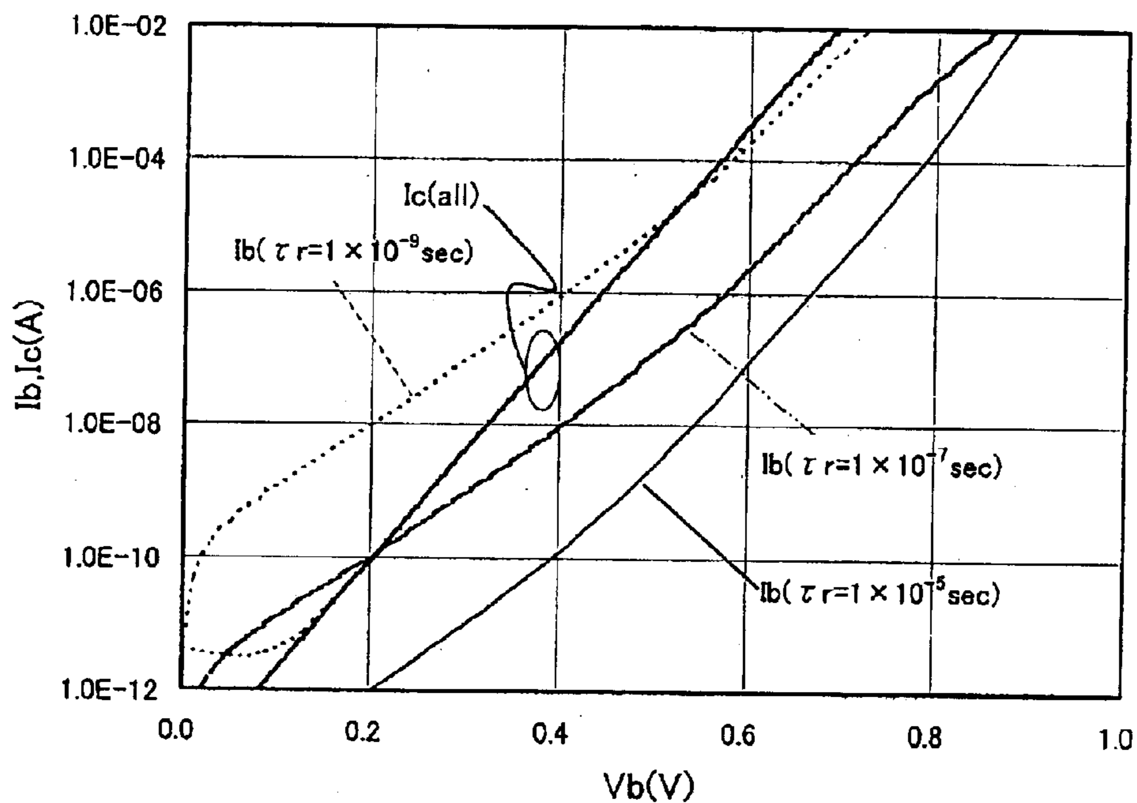
Gummel plot
