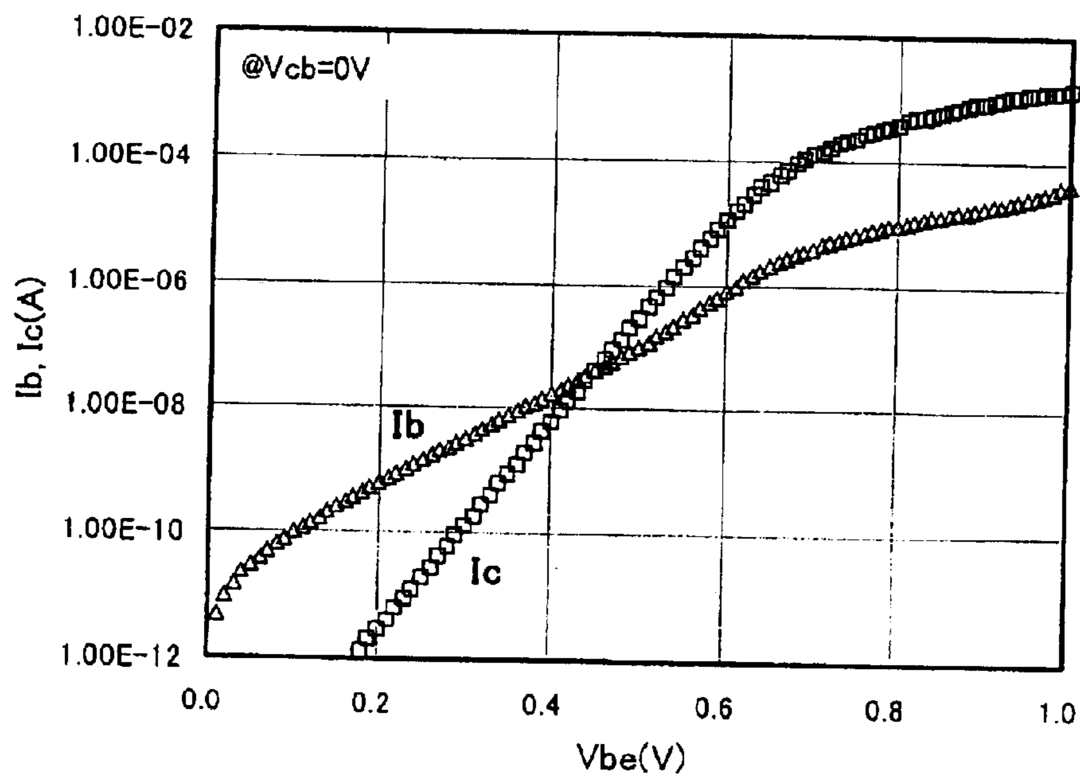
SiGe 0.268 C 0.0091 HBT Gummel plot
