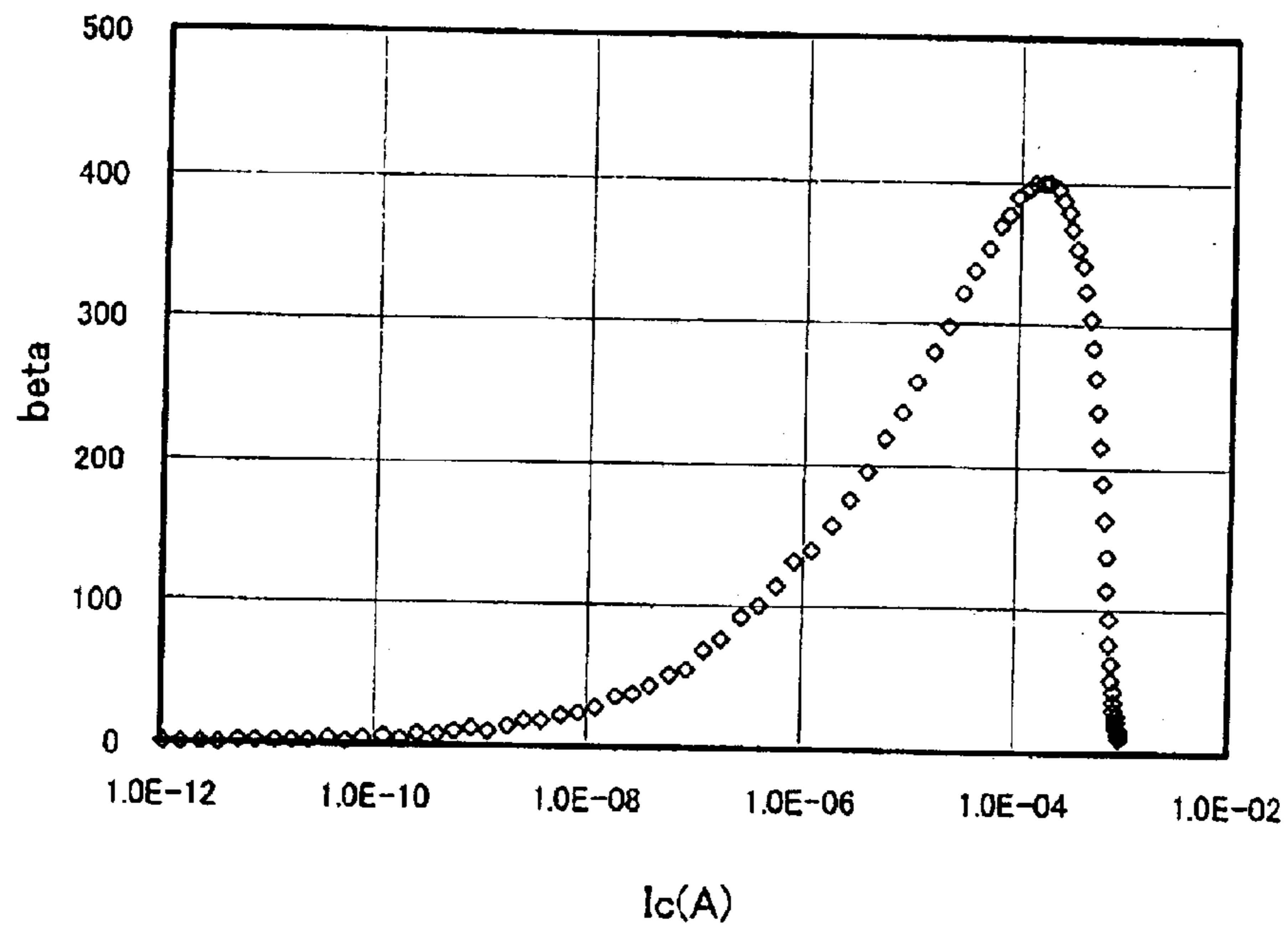
Current multiplication factor of SiGe 0.268 HBT
