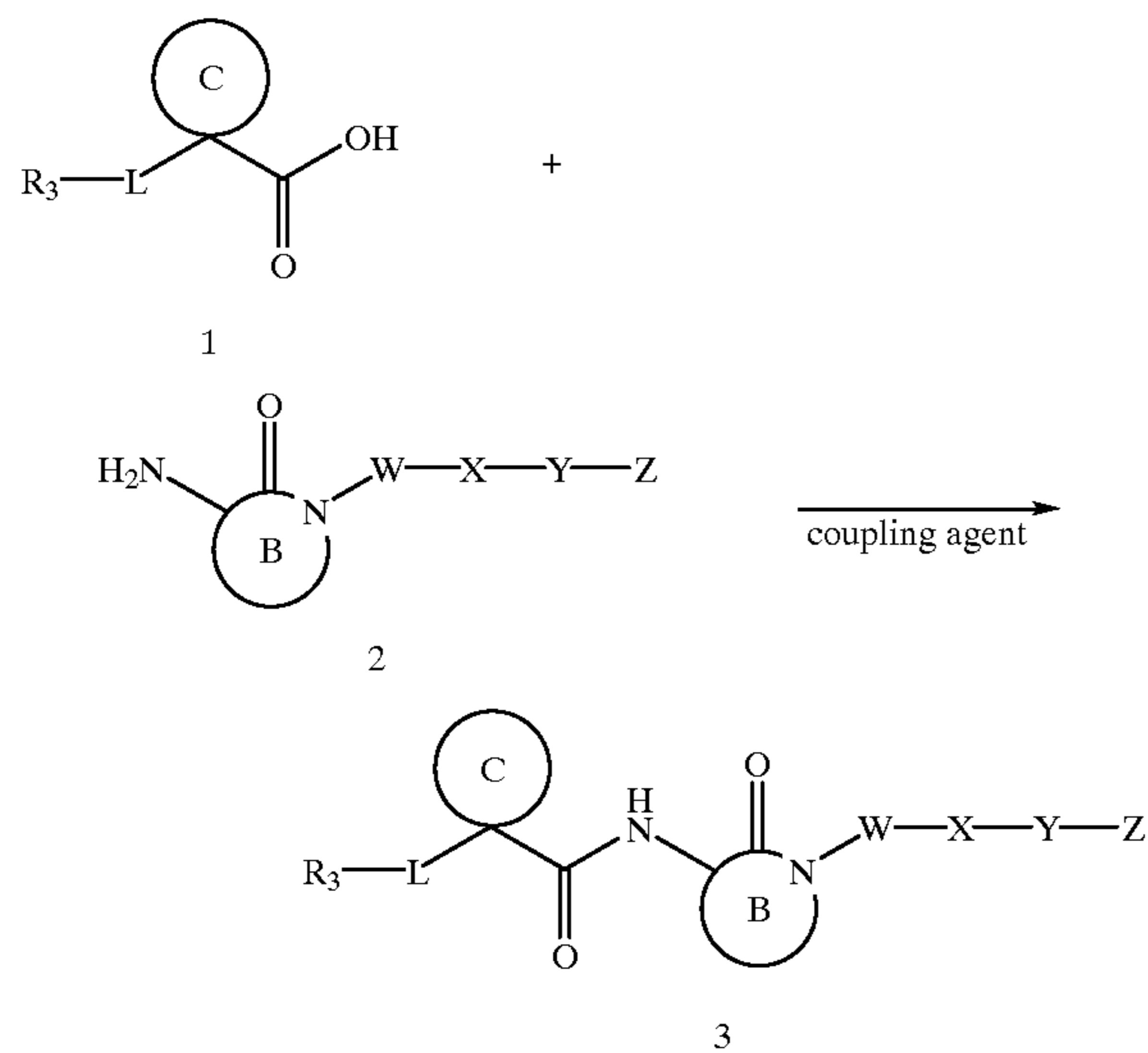
Scheme 1
