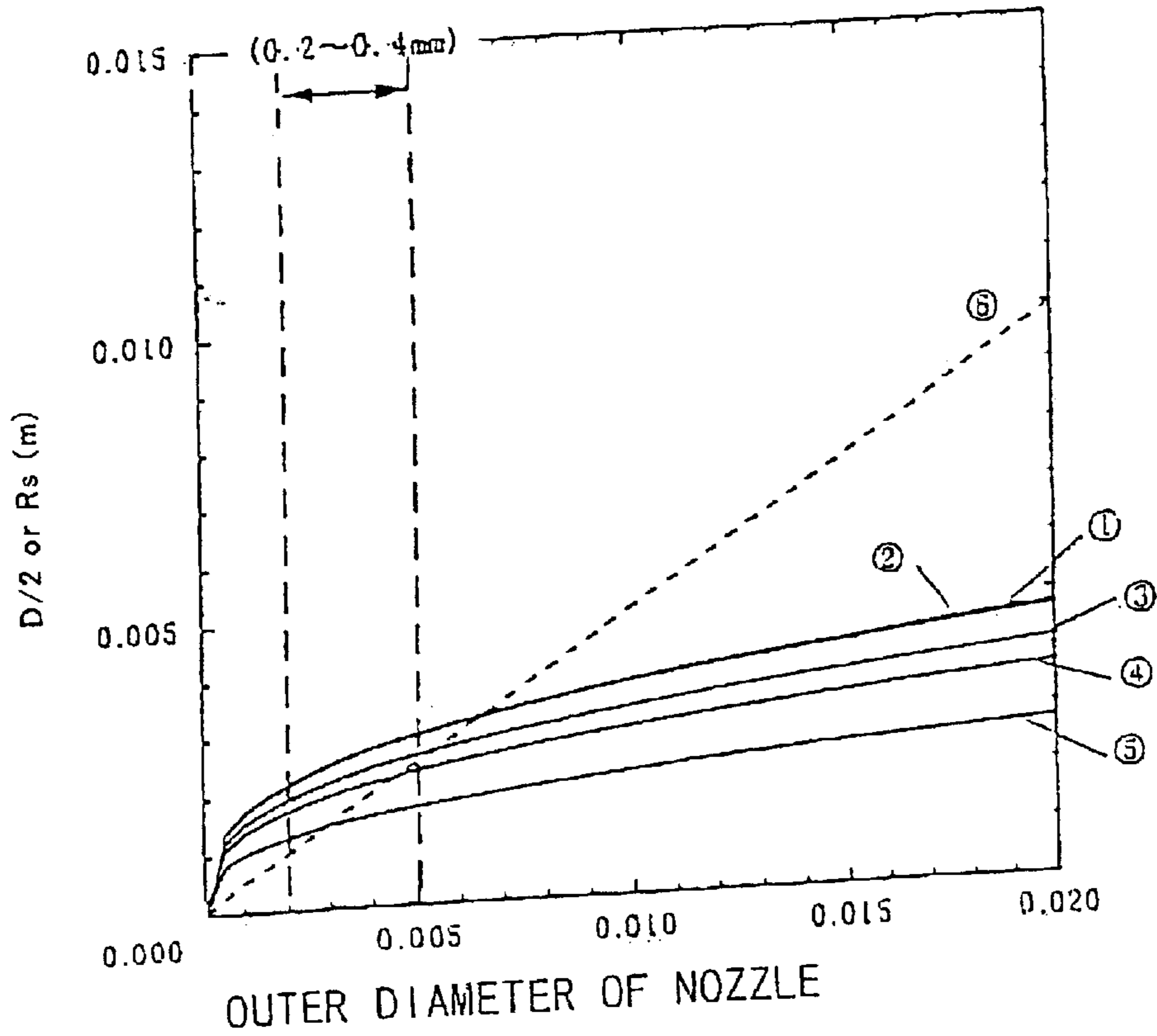
FIG. 5 (C) OUTER DIAMETER OF ORDINARY NOZZLE
