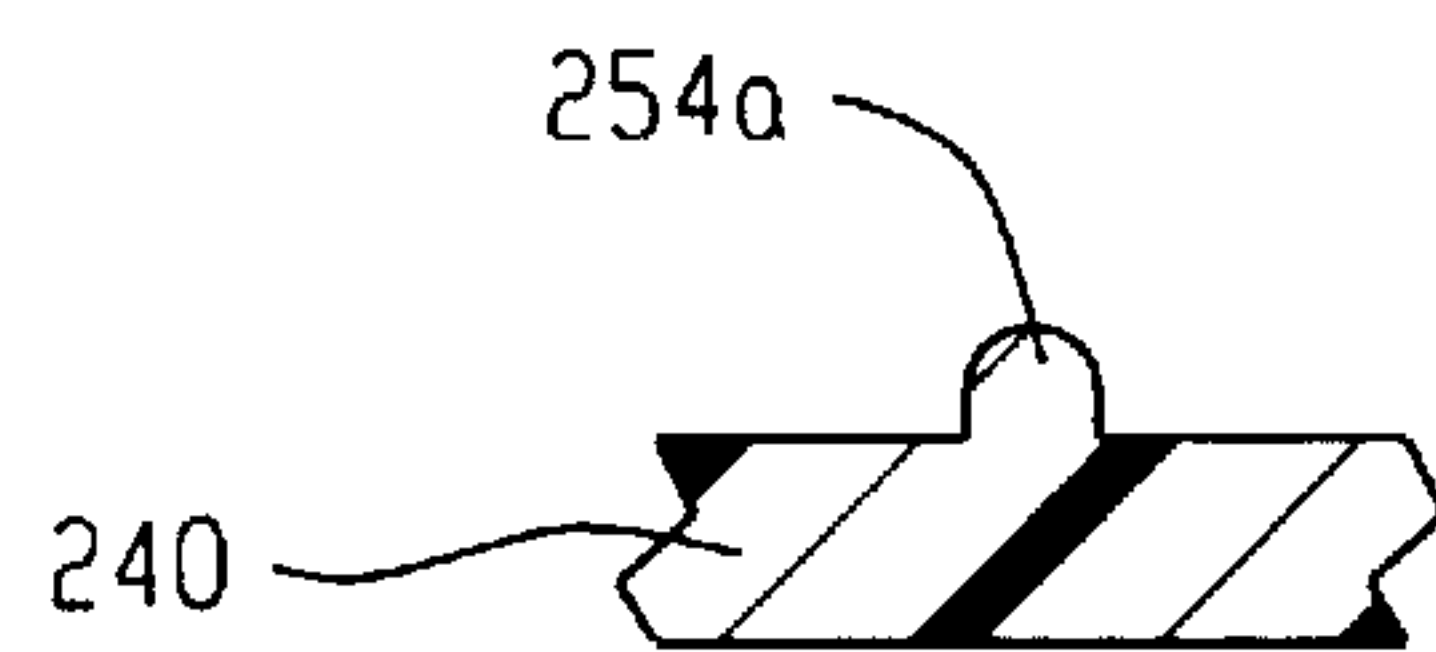
SECTION C-C
