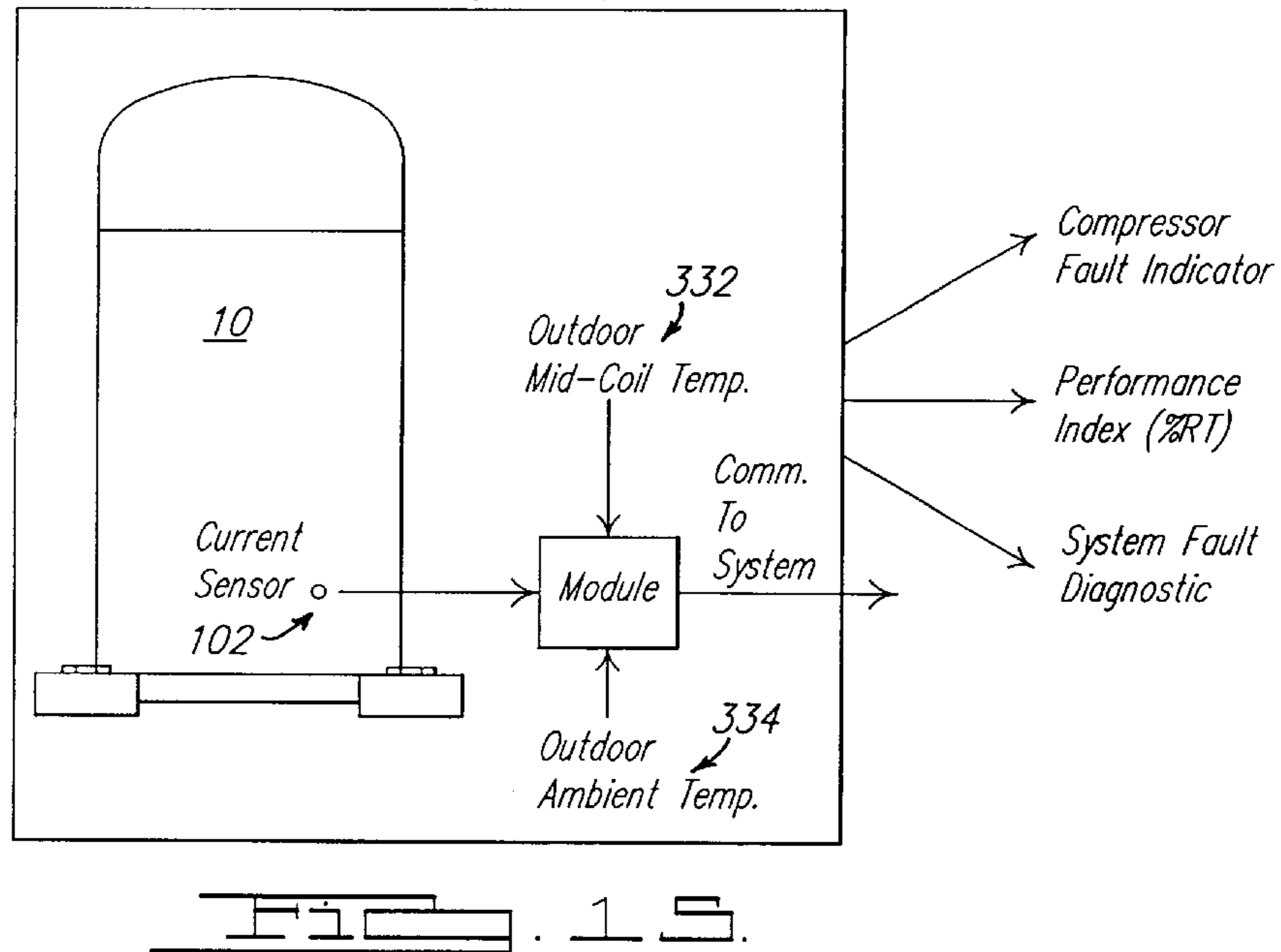
Integrated Protection/Diagnostic/Defrost Control
