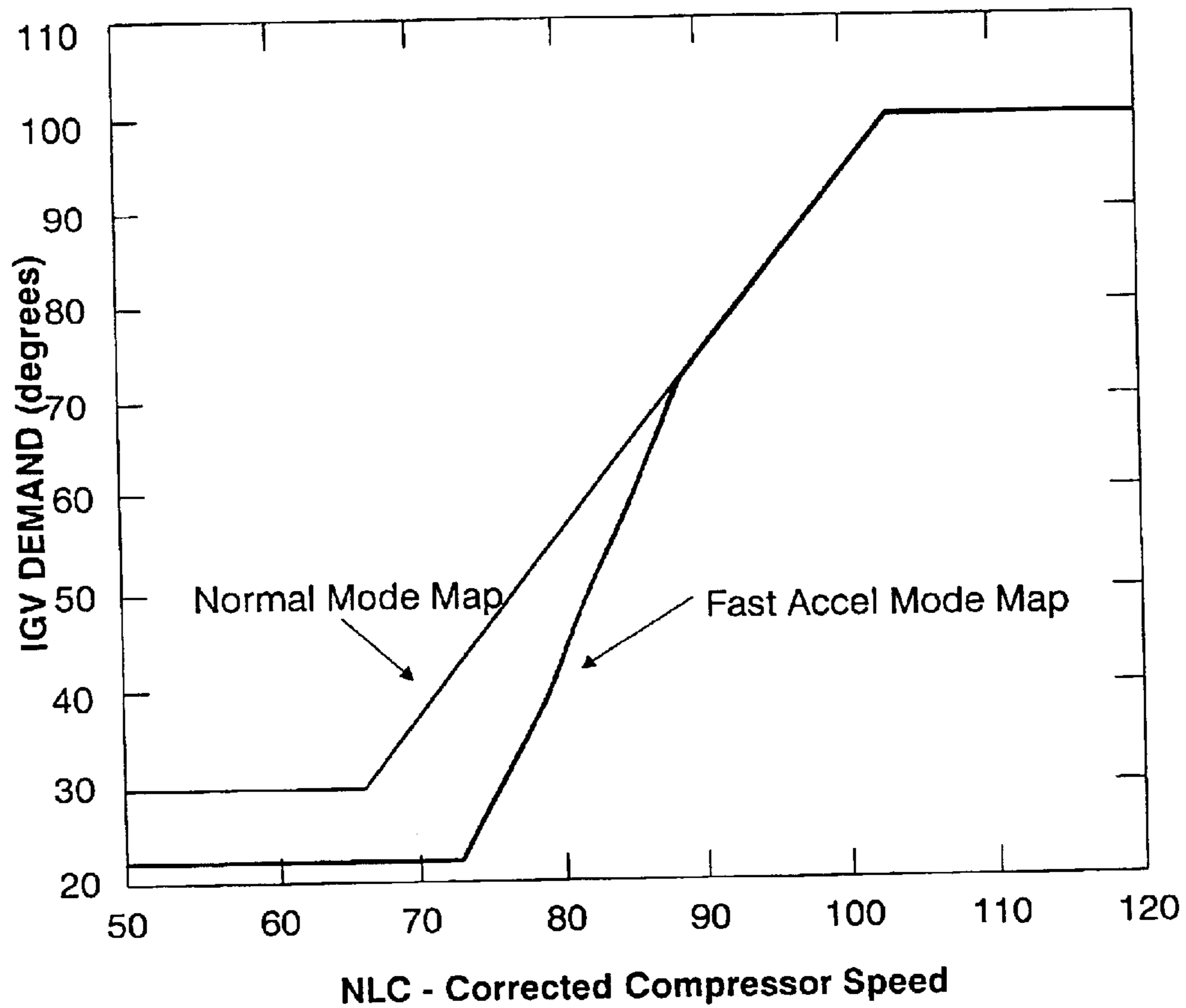
Steady-State IGV Schedules
