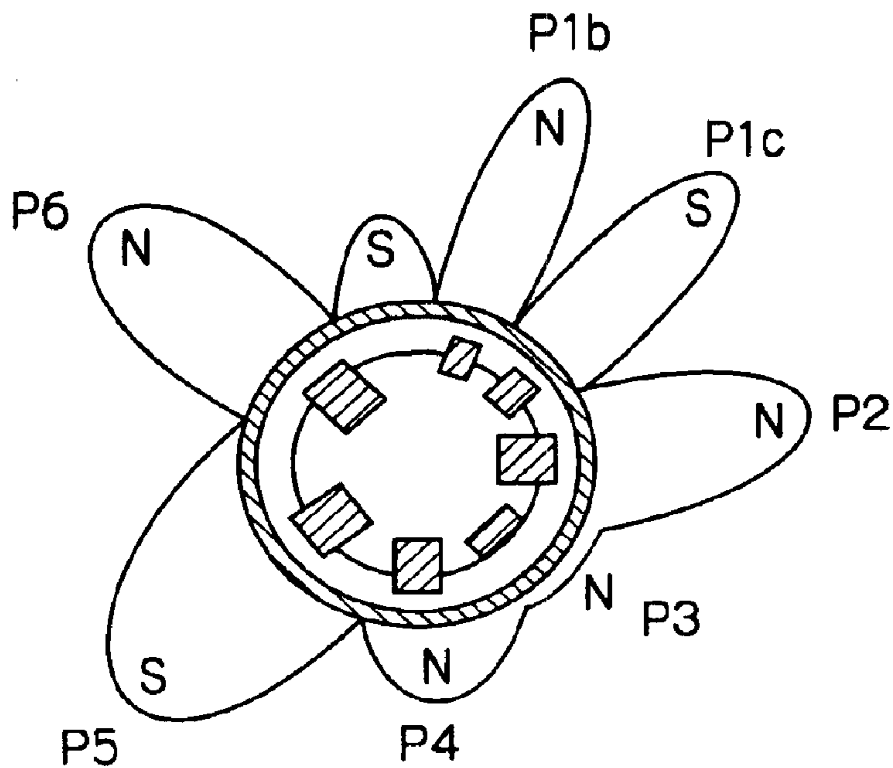
Fig. 42 PRIOR ART
