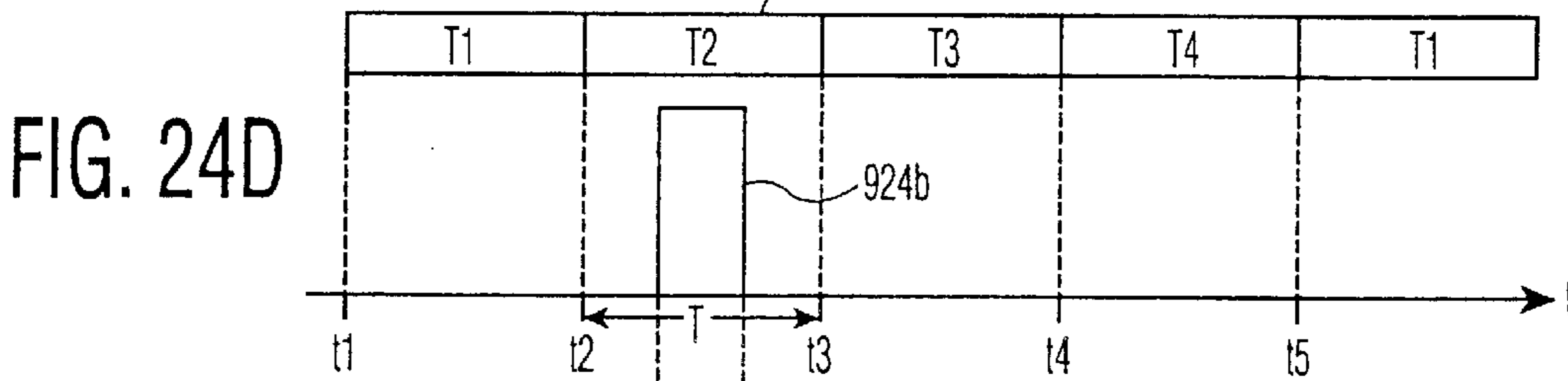
FIG. 24D (3) RECORDED SIGNAL OF "01"
