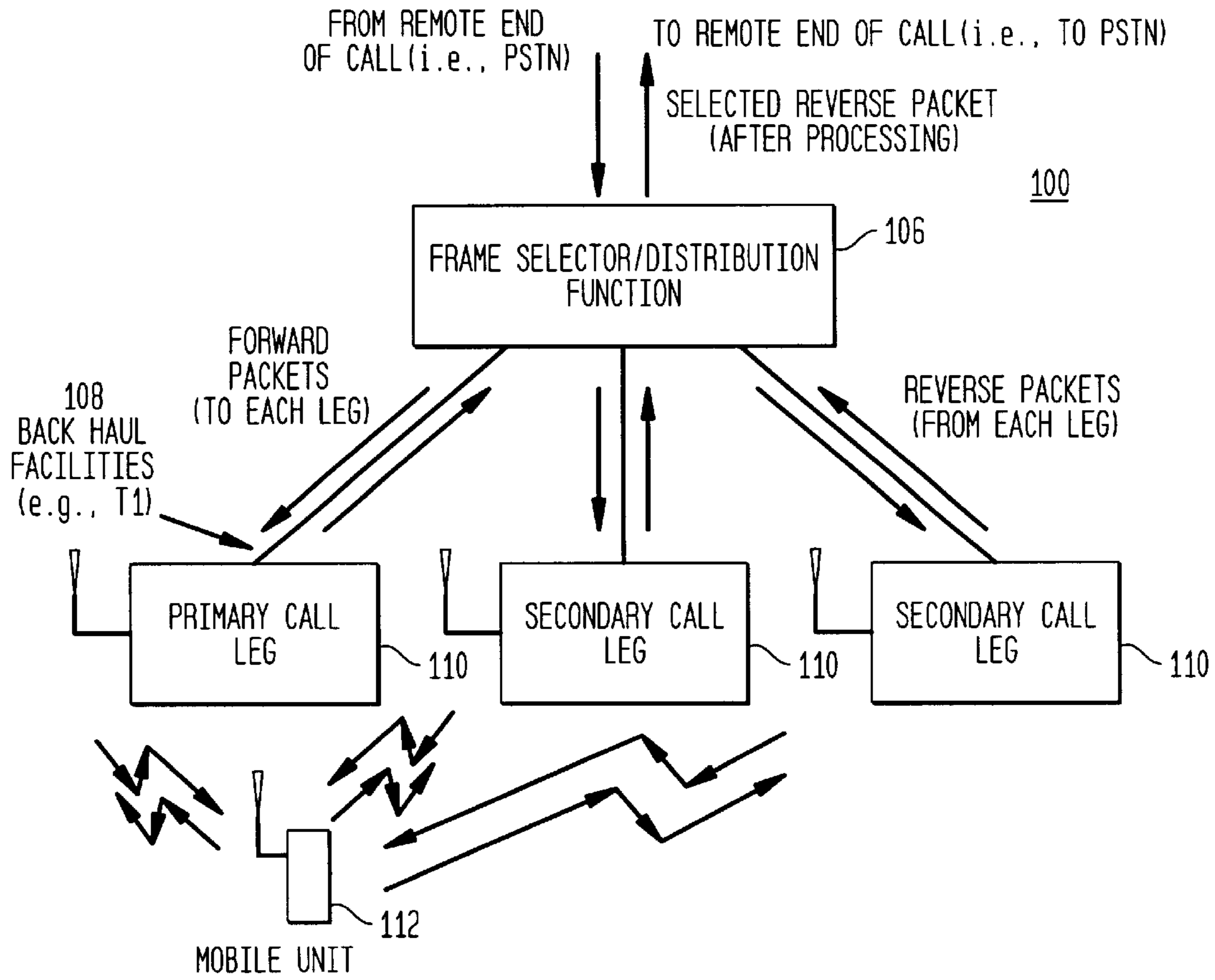
FIG. 2 (PRIOR ART)
