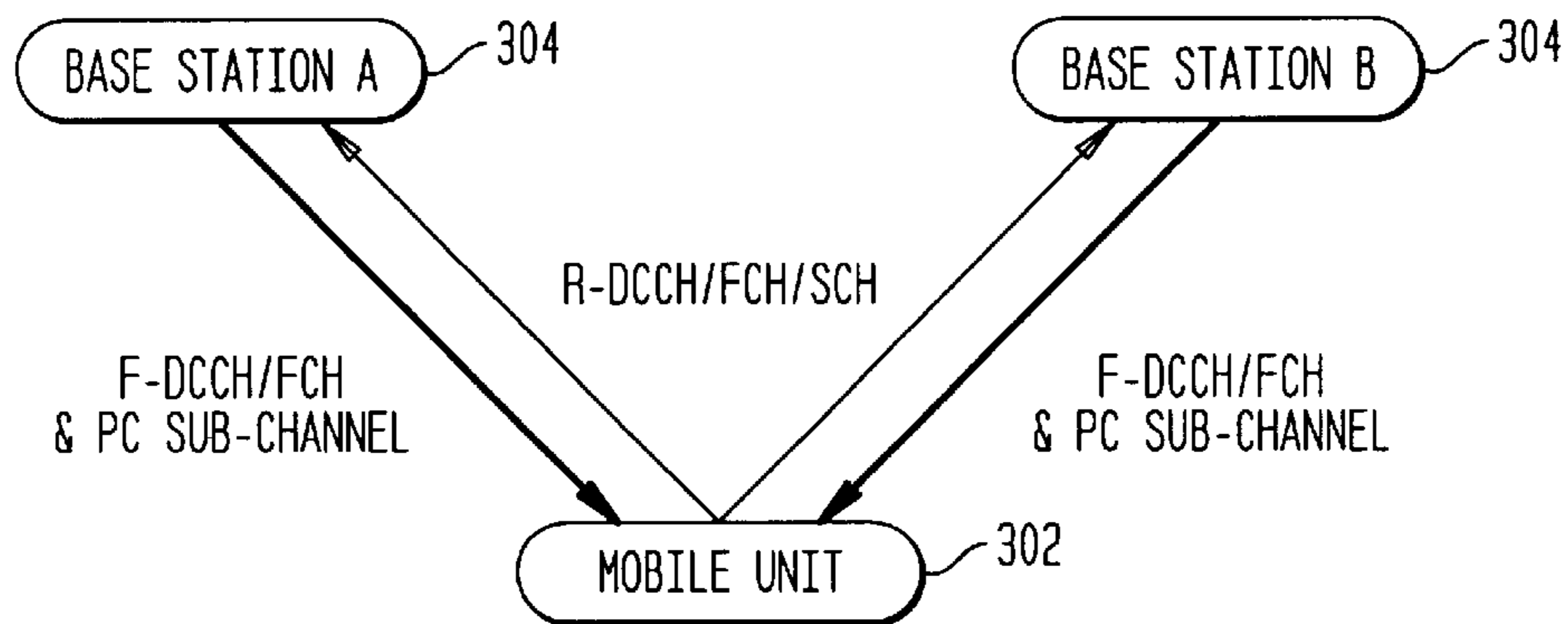
FIG. 3 (PRIOR ART)
