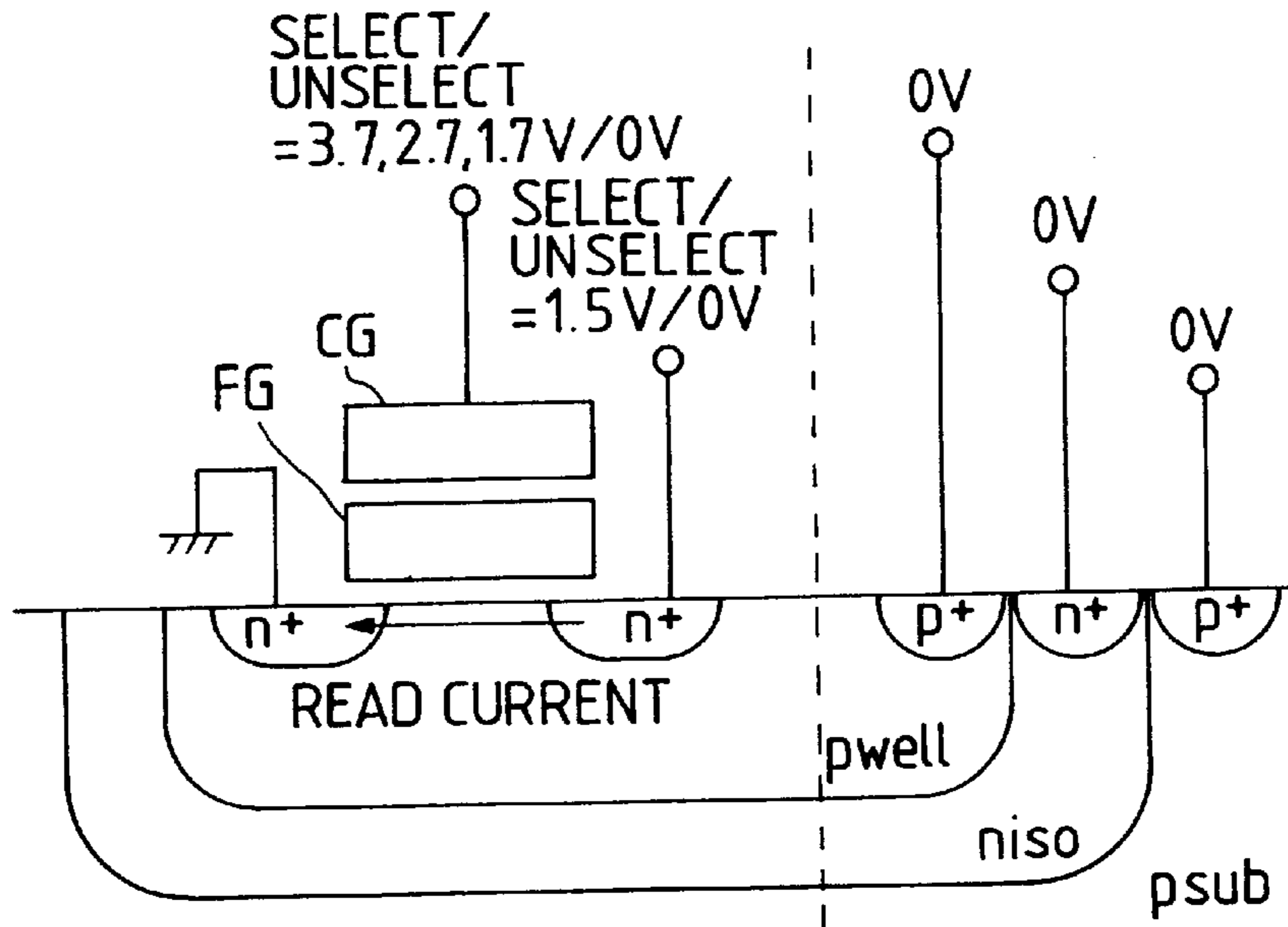
EXAMPLE OF APPLIED VOLTAGES AT READING TIME
