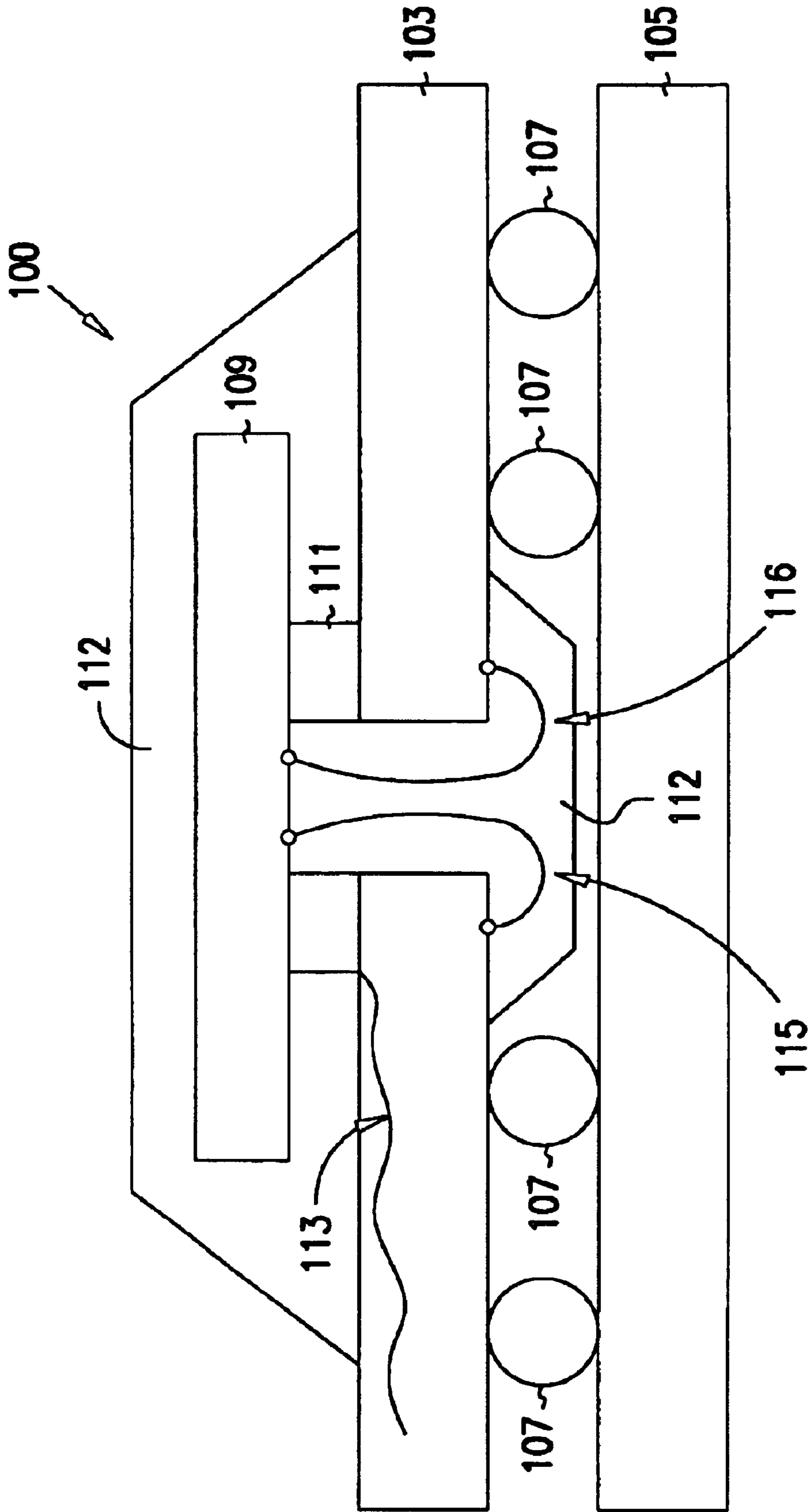
Figure 1 (PRIOR ART)
