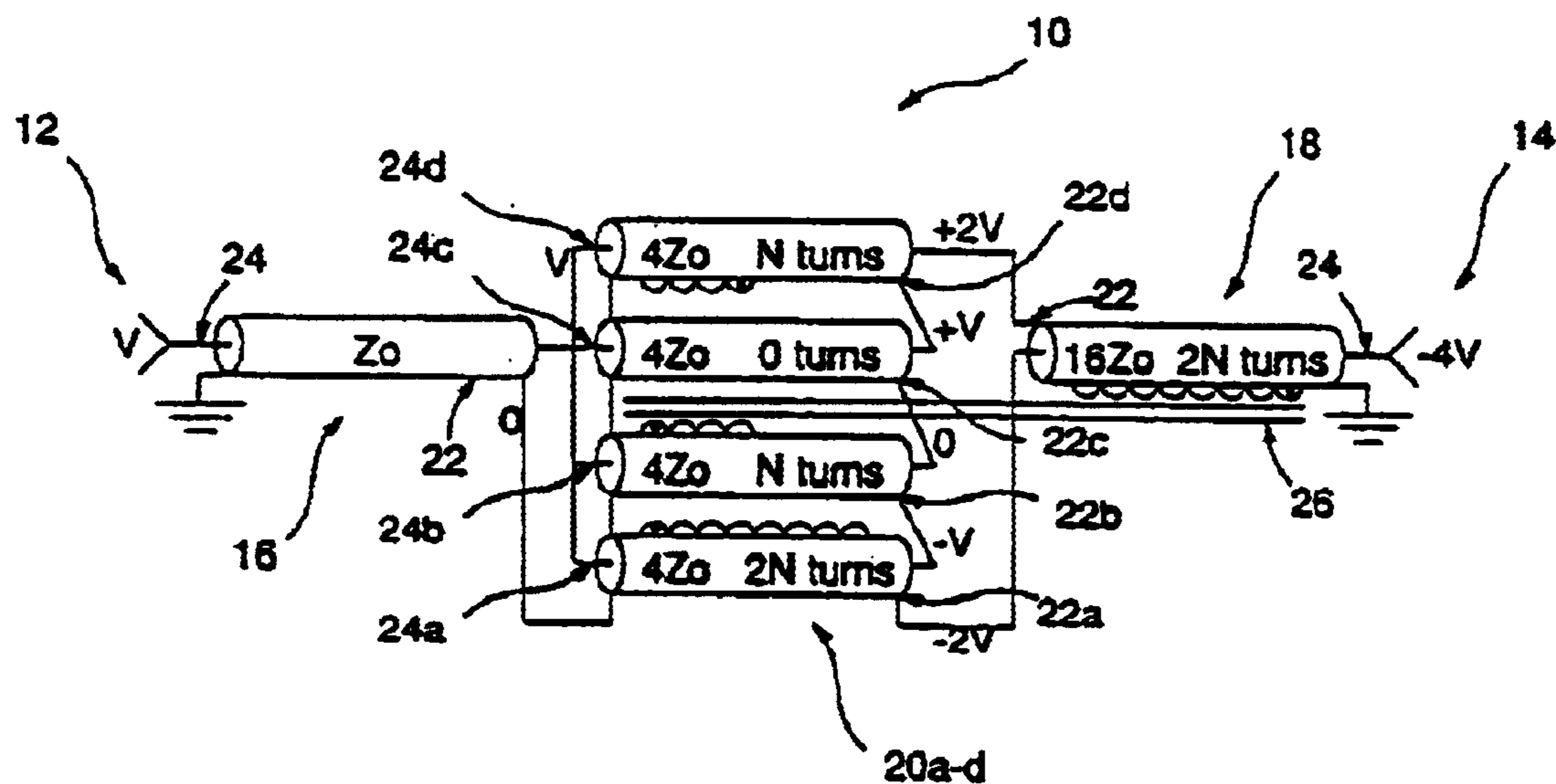
Figure 2. 16:1 Inverting Balanced TLT of prior art.
