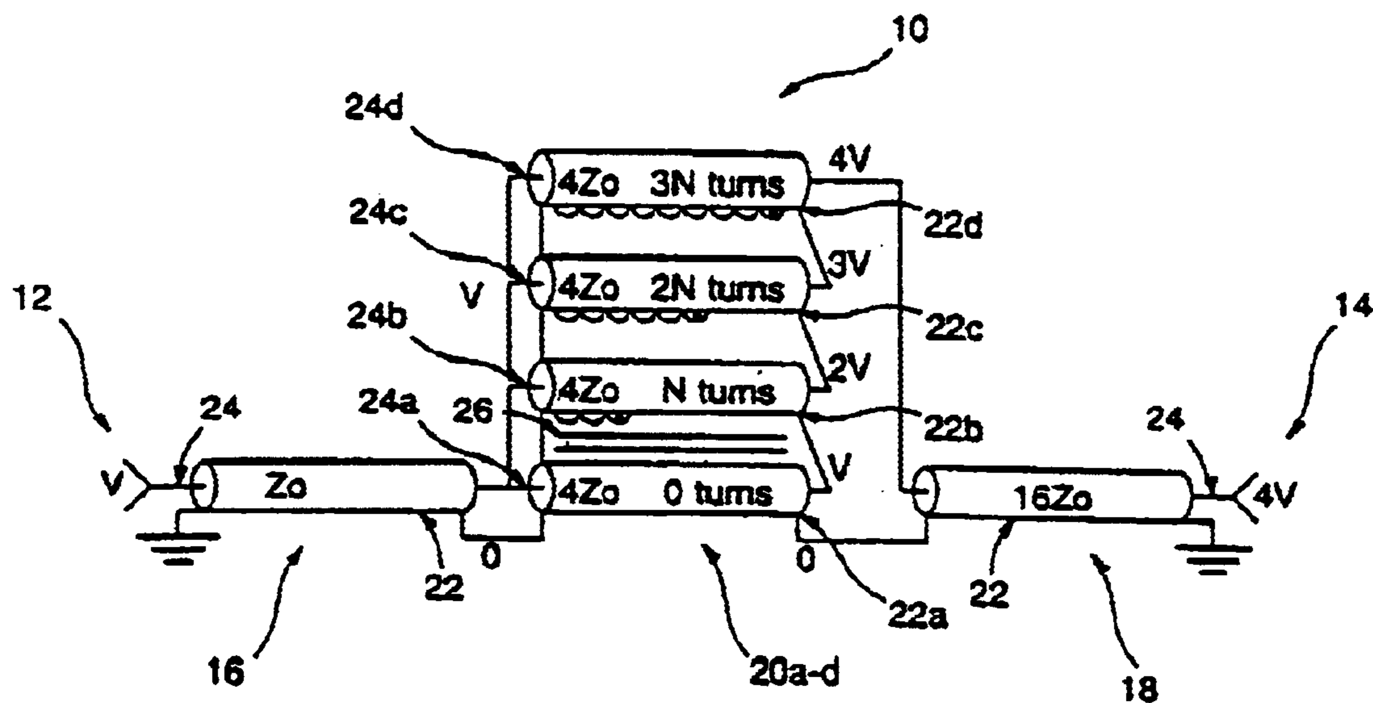
Figure 1. 16:1 TLT of the prior art
