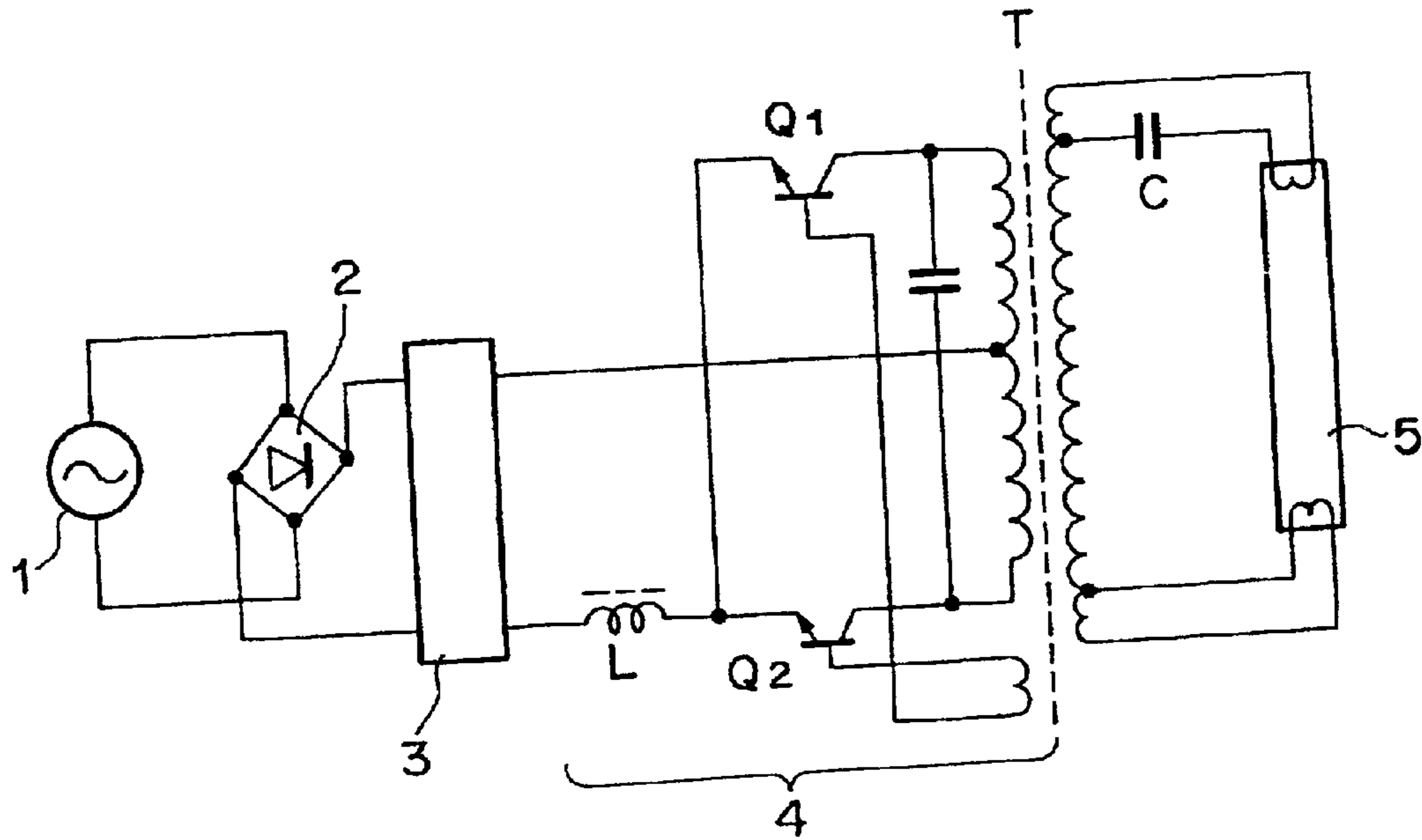
FIG. 21 PRIOR ART
