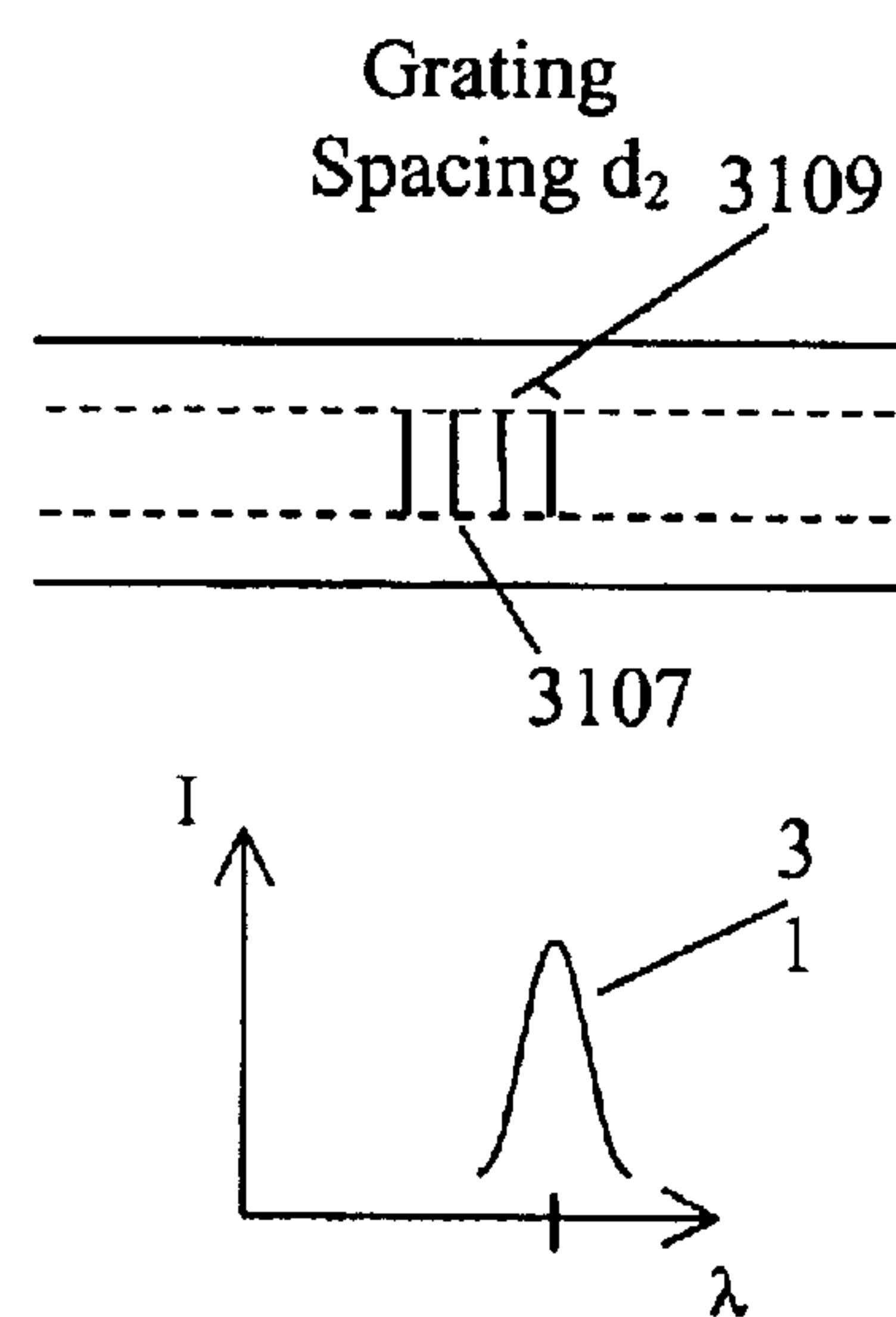
Reflected Peak at Higher Center Wavelength
