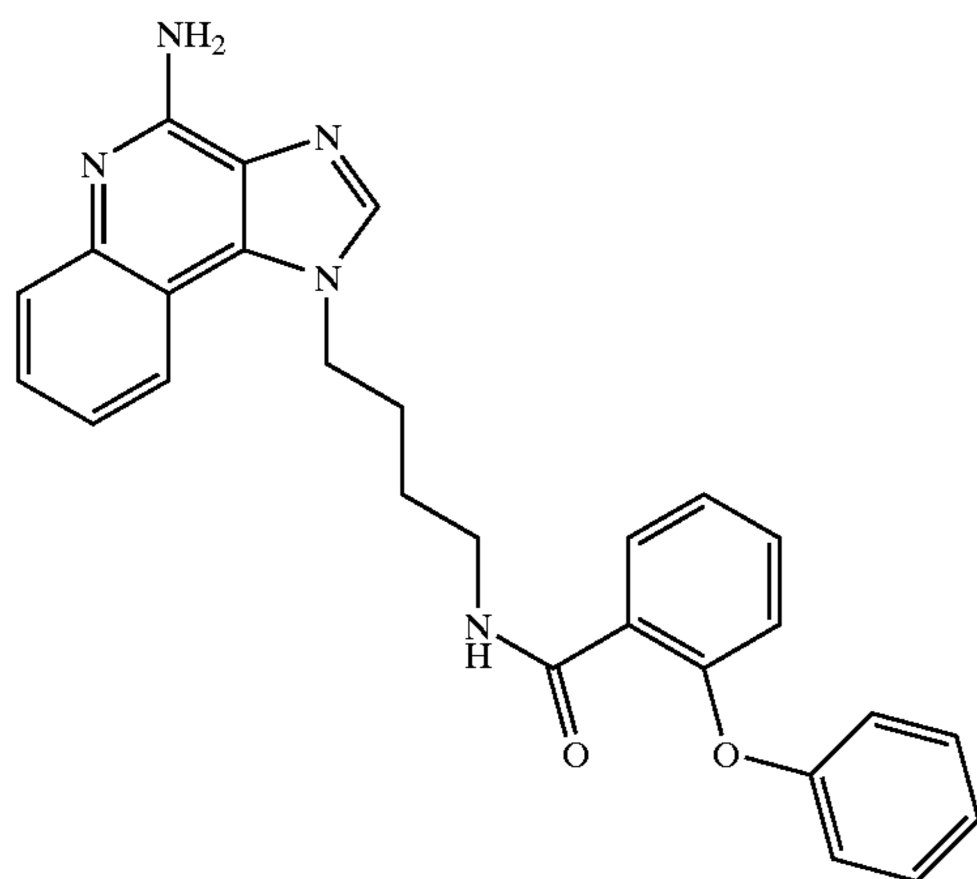
N 1 -[4-(4-Amino-1H-imidazo[4,5-c]quinolin-1-yl)butyl]-2-phenoxybenzamide
