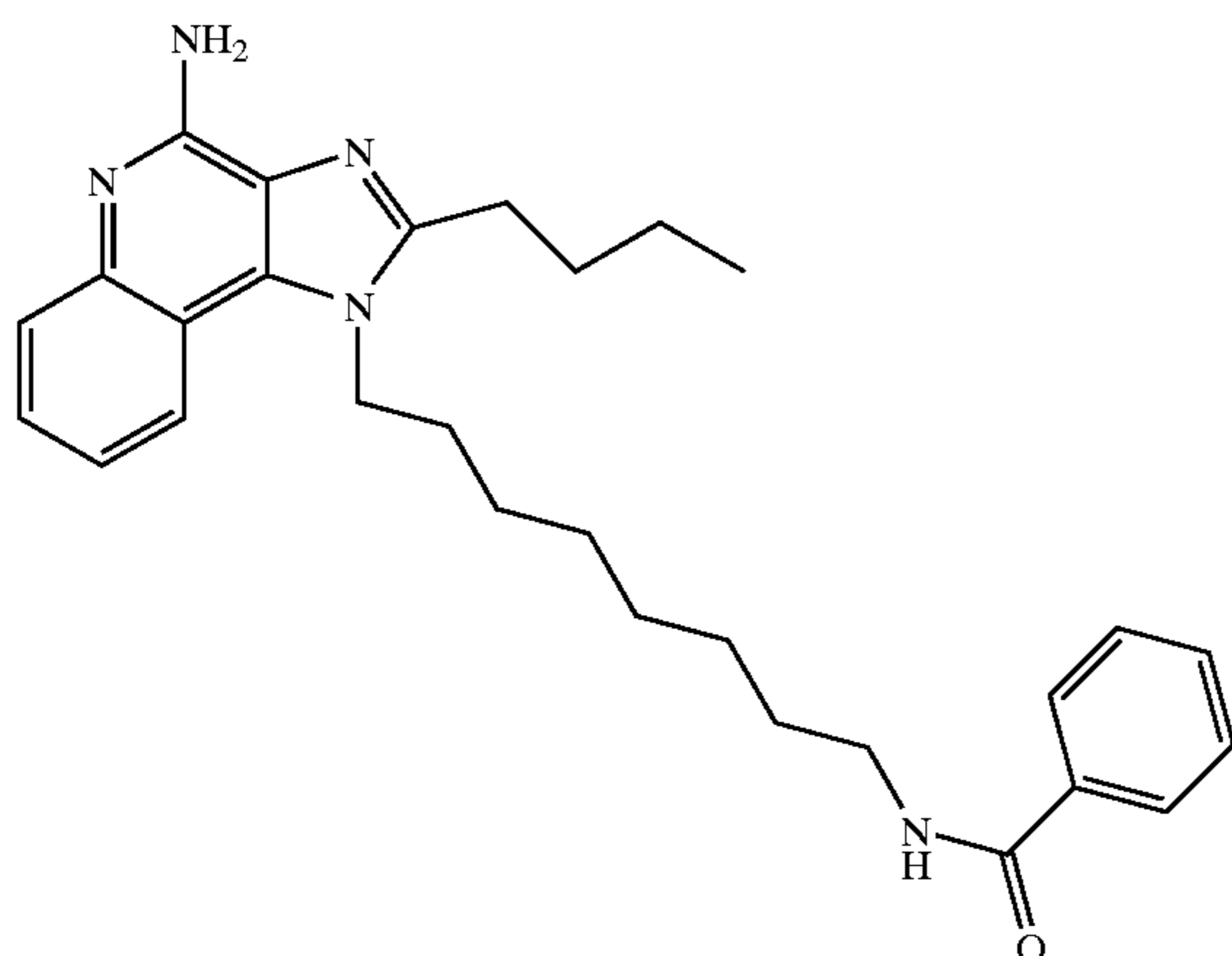
N-[8-(4-amino-2-butyl-1H-imidazo[4,5-c]quinolin-1-yl)octyl]benzamide
