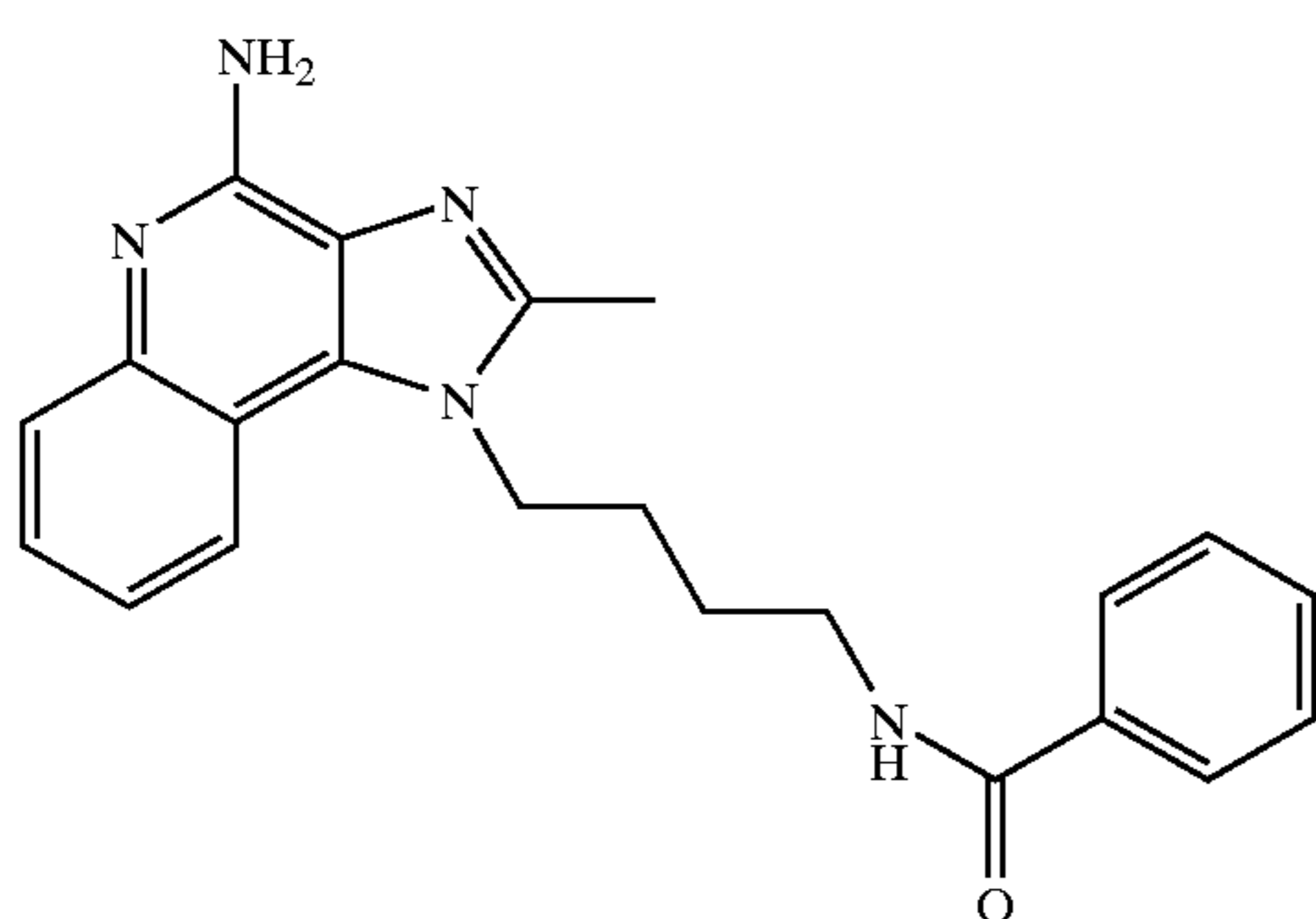
N 1 -[4-(4-Amino-2-methyl-1H-imidazo[4,5-c]quinolin-1-yl)butyl]benzamide
