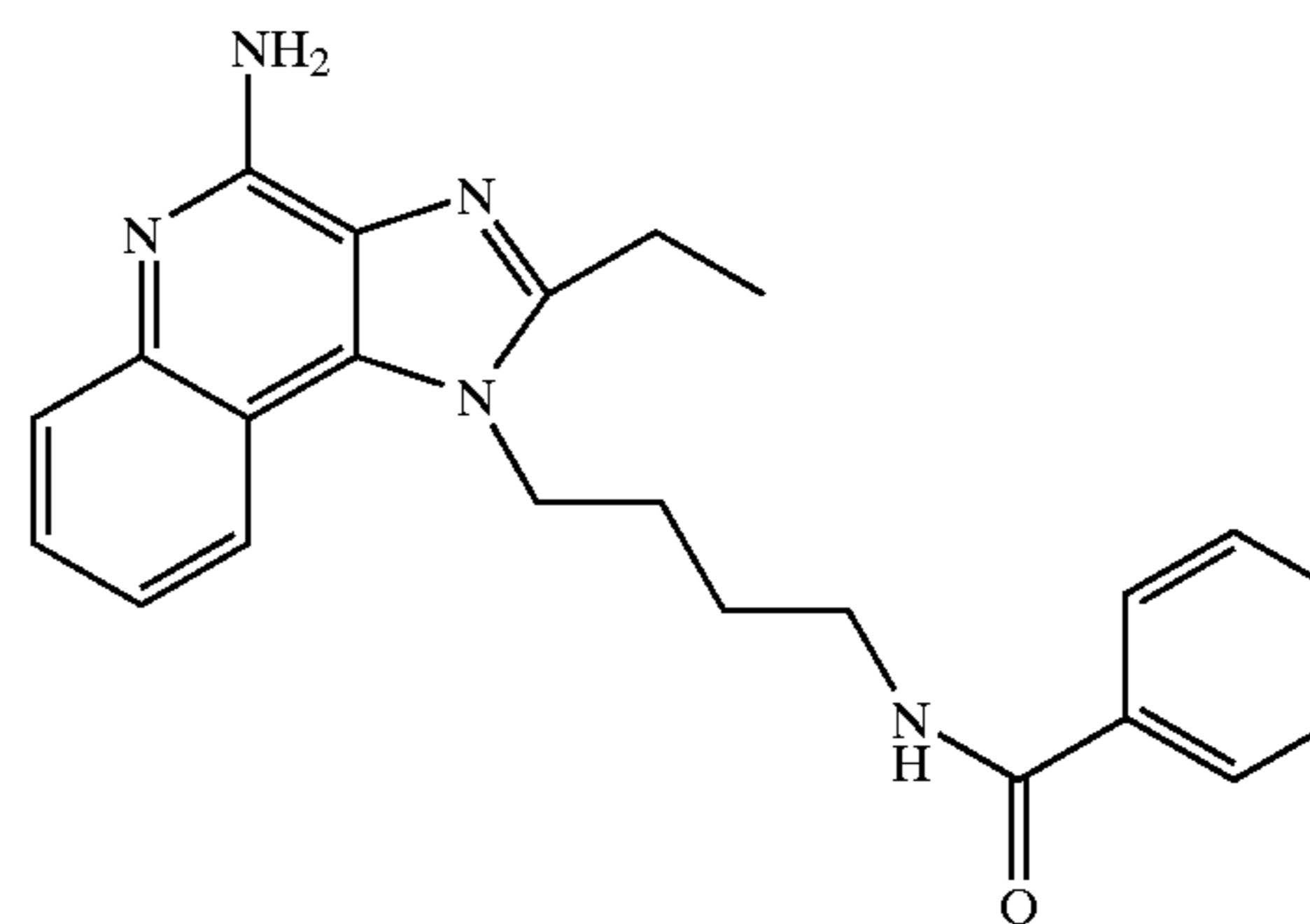
N 1 -[4-(4-Amino-2-ethyl-1H-imidazo[4,5-c]quinolin-1-yl)butyl]benzamide
