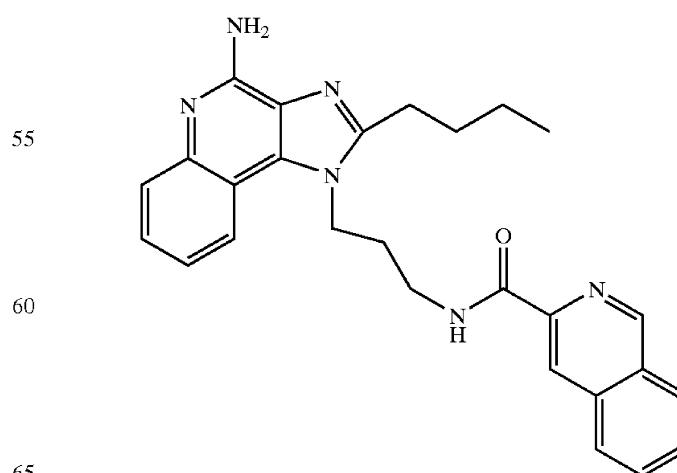
N-[3-(4-amino-2-butyl-1H-imidazo[4,5-c]quinolin-1-yl)propyl]isoquinoline-3-carboxamide
