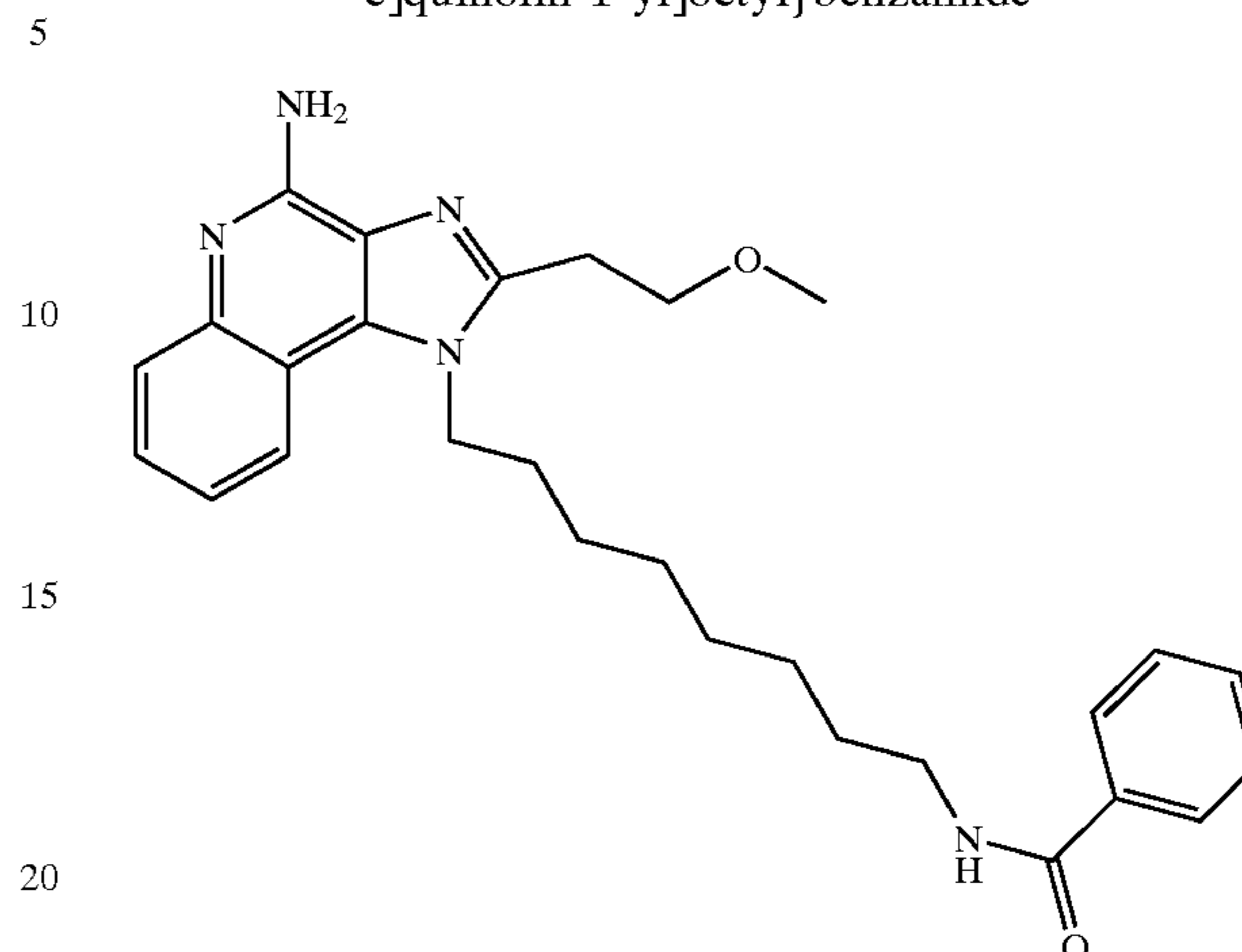
N-{8-[4-amino-2-(2-methoxyethyl)-1H-imidazo[4,5-c]quinolin-1-yl]octyl}benzamide
