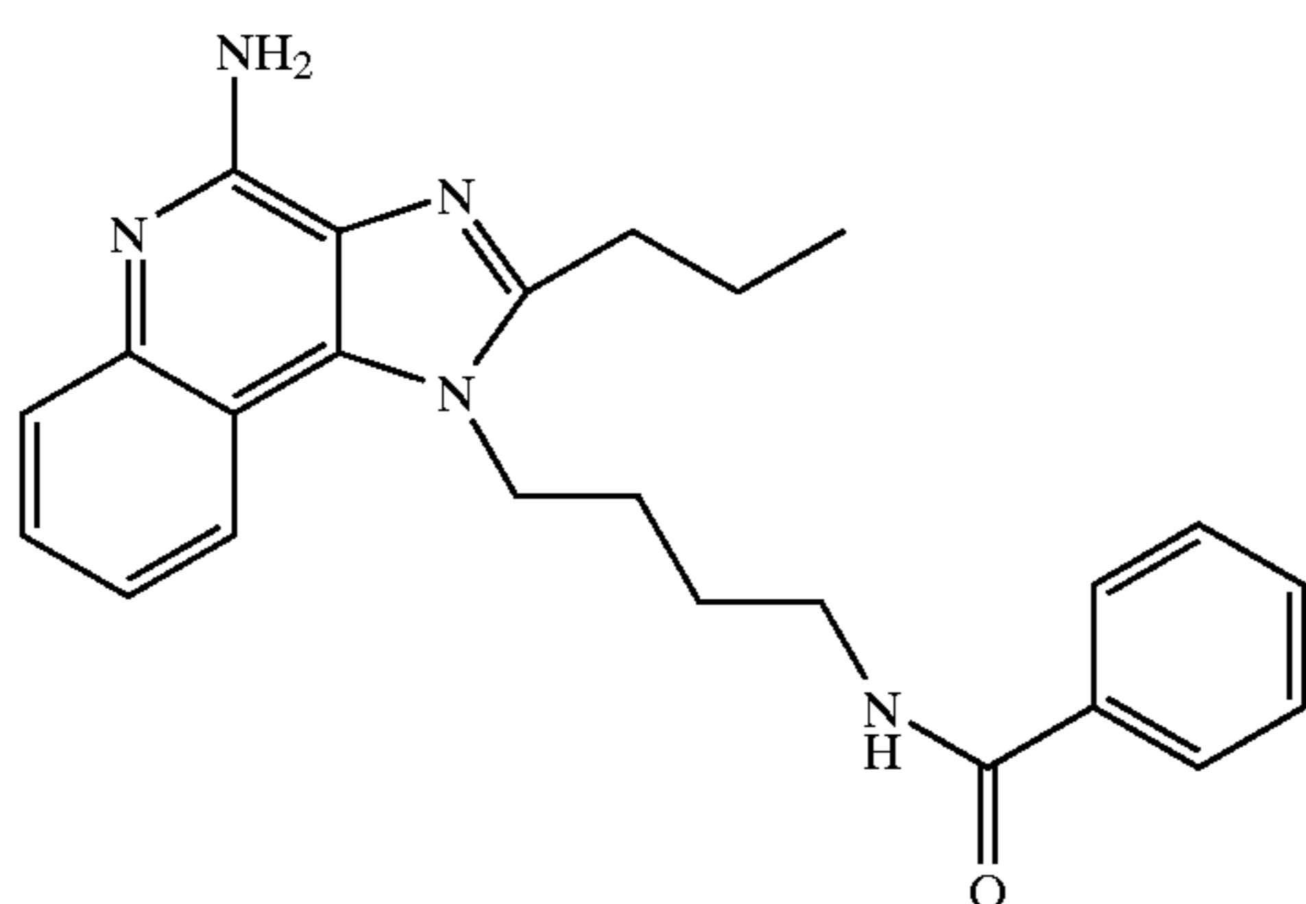
N 1 -[4-(4-Amino-2-propyl-1H-imidazo[4,5-c]quinolin-1-yl)butyl]benzamide
