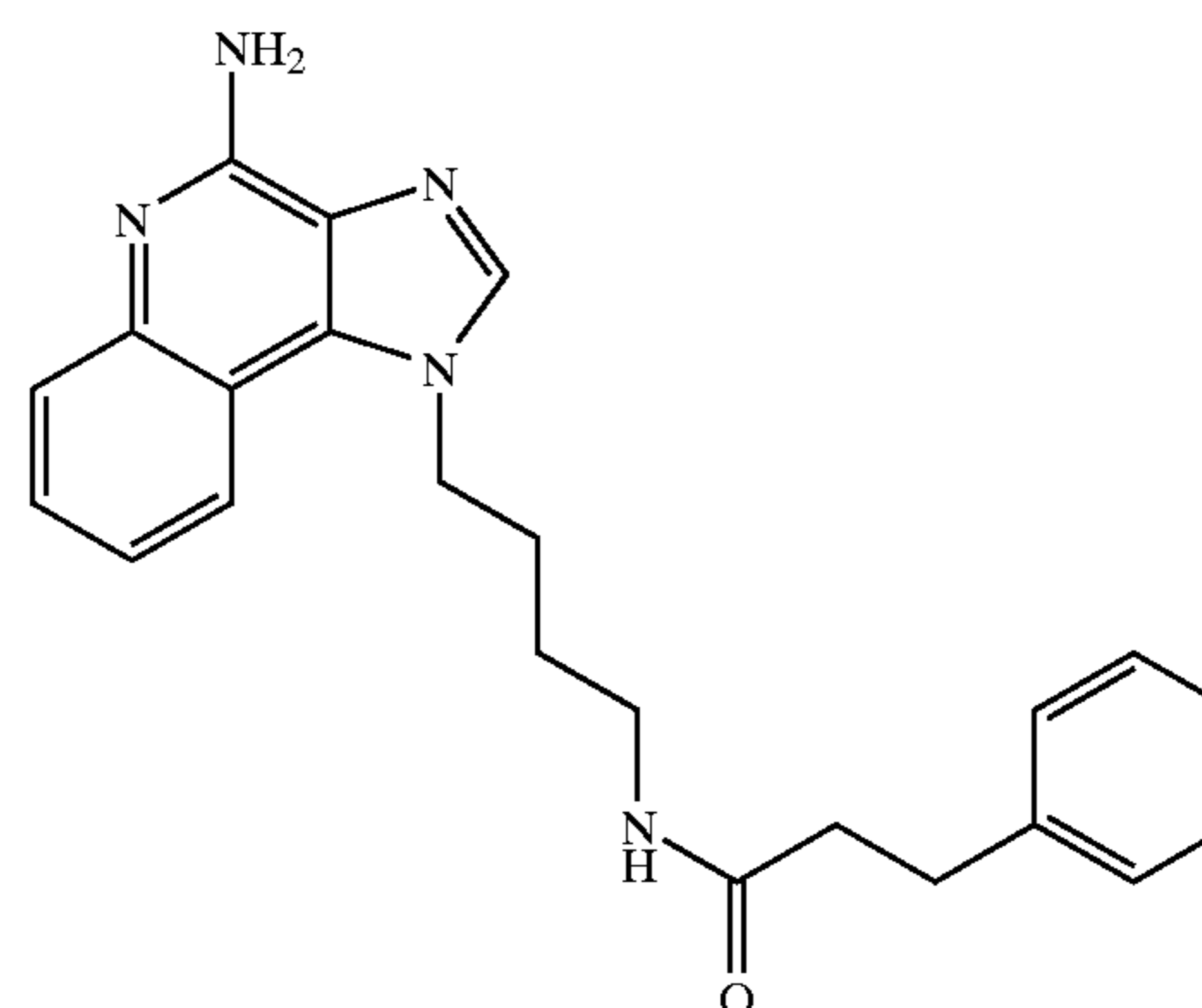
N 1 -[4-(4-Amino-1H-imidazo[4,5-c]quinolin-1-yl)butyl]-3-phenylpropanamide
