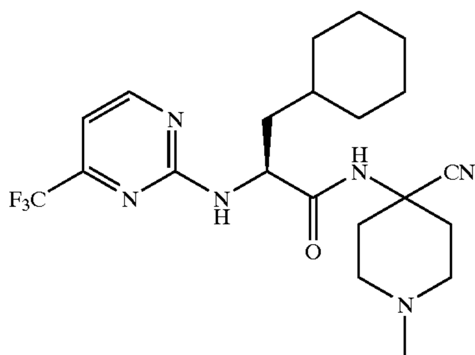
N-(4-cyano-1-methyl-piperidin-4-yl)-2-(4-trifluoromethyl-pyrimidin-2-ylamino)-3-cyclohexyl-propionamide
