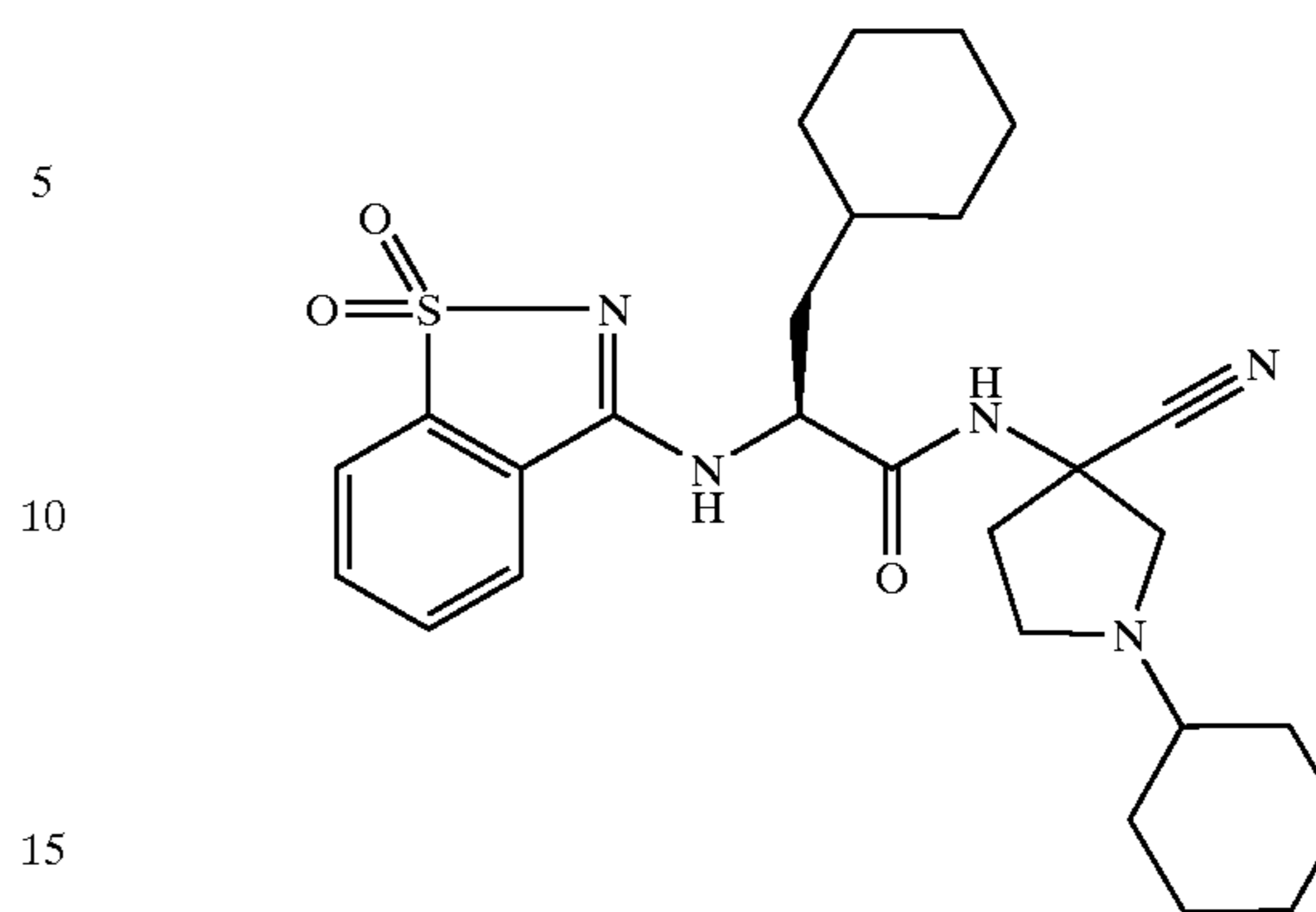
N-(3-Cyano-1-cyclohexyl-pyrrolidin-3-yl)-3- cyclohexyl-2-(1,1-dioxo-1H-1λ 6 -benzo[d]isothiazol- 3-ylamino)-propionamide
