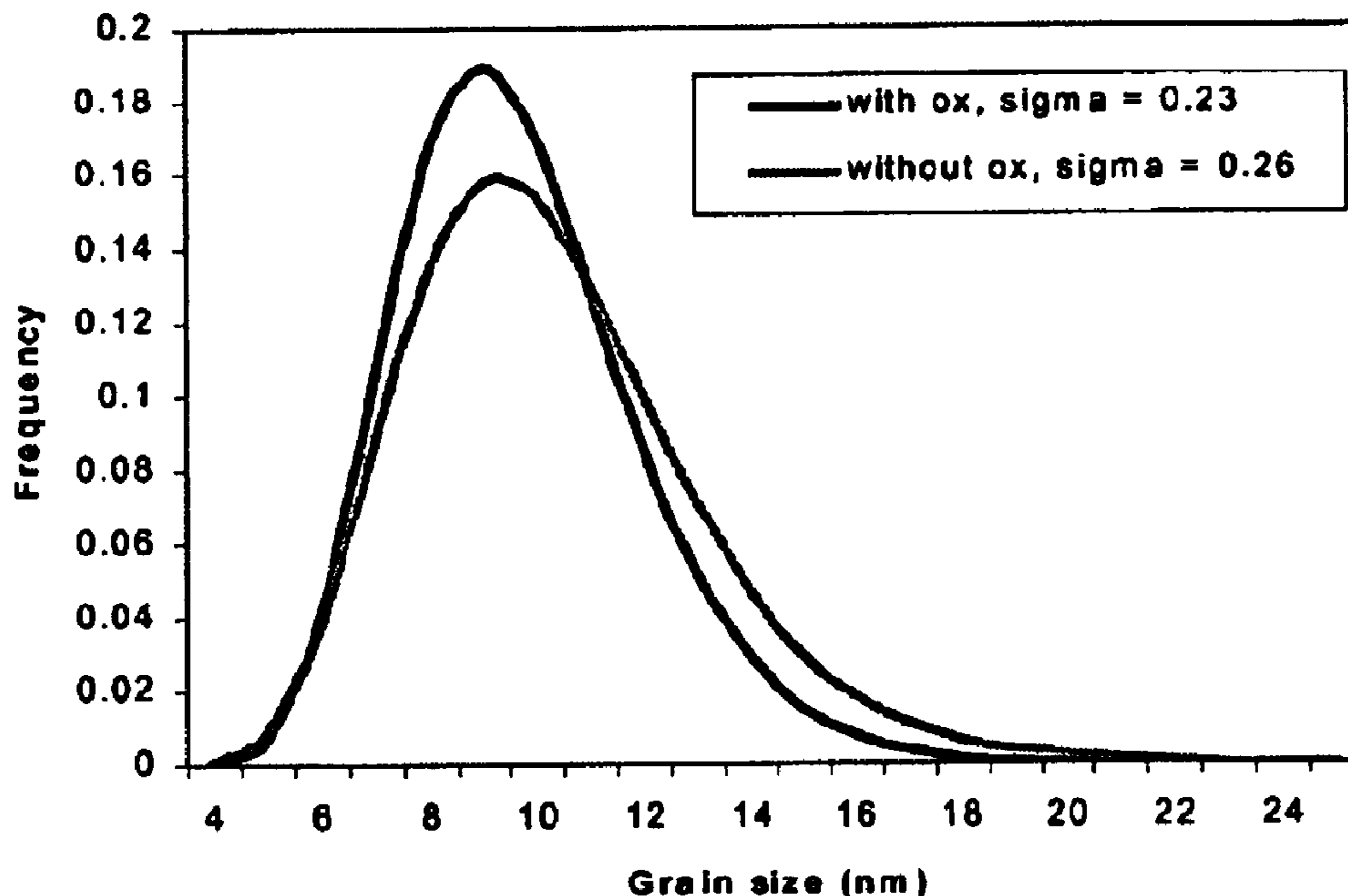
Comparison of Grain Size Distributions x1994 with and without Oxygen
