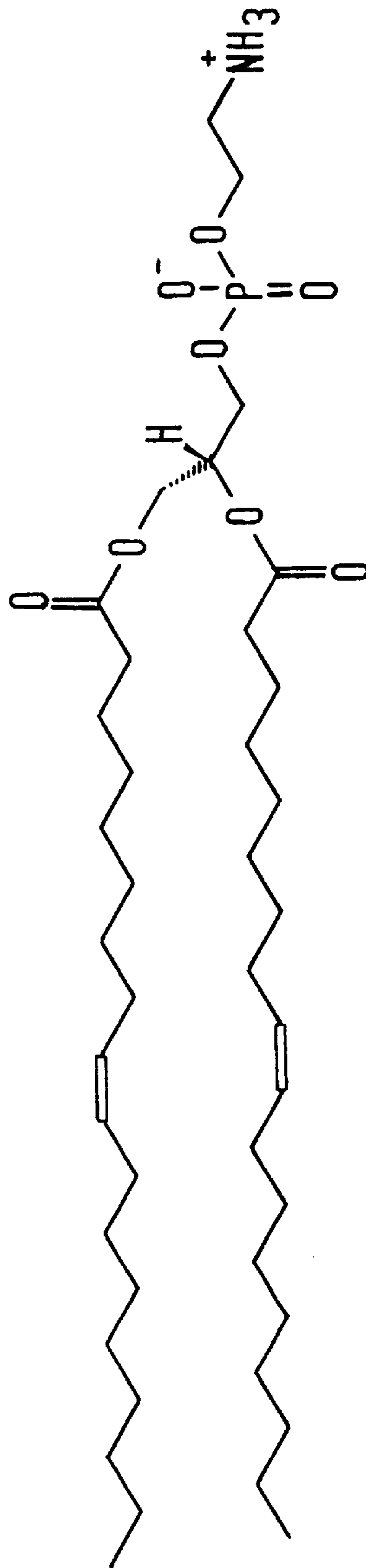
DOPE Dioleoylphosphatidyl ethanolamine
