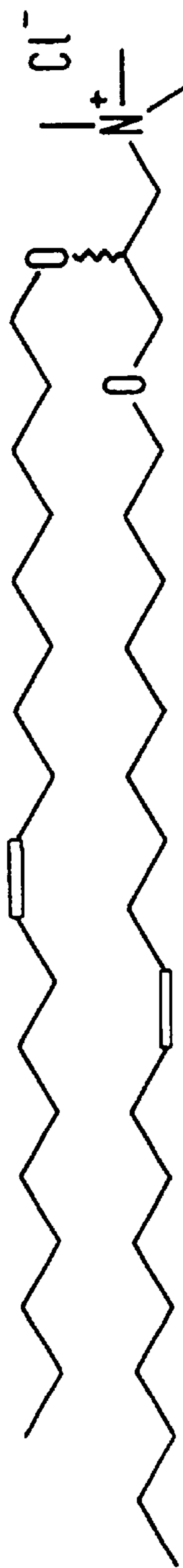
DOTMA N -[1-(2,3-dioleoyloxy)propyl]- N,N,N -trimethyl ammonium chloride
