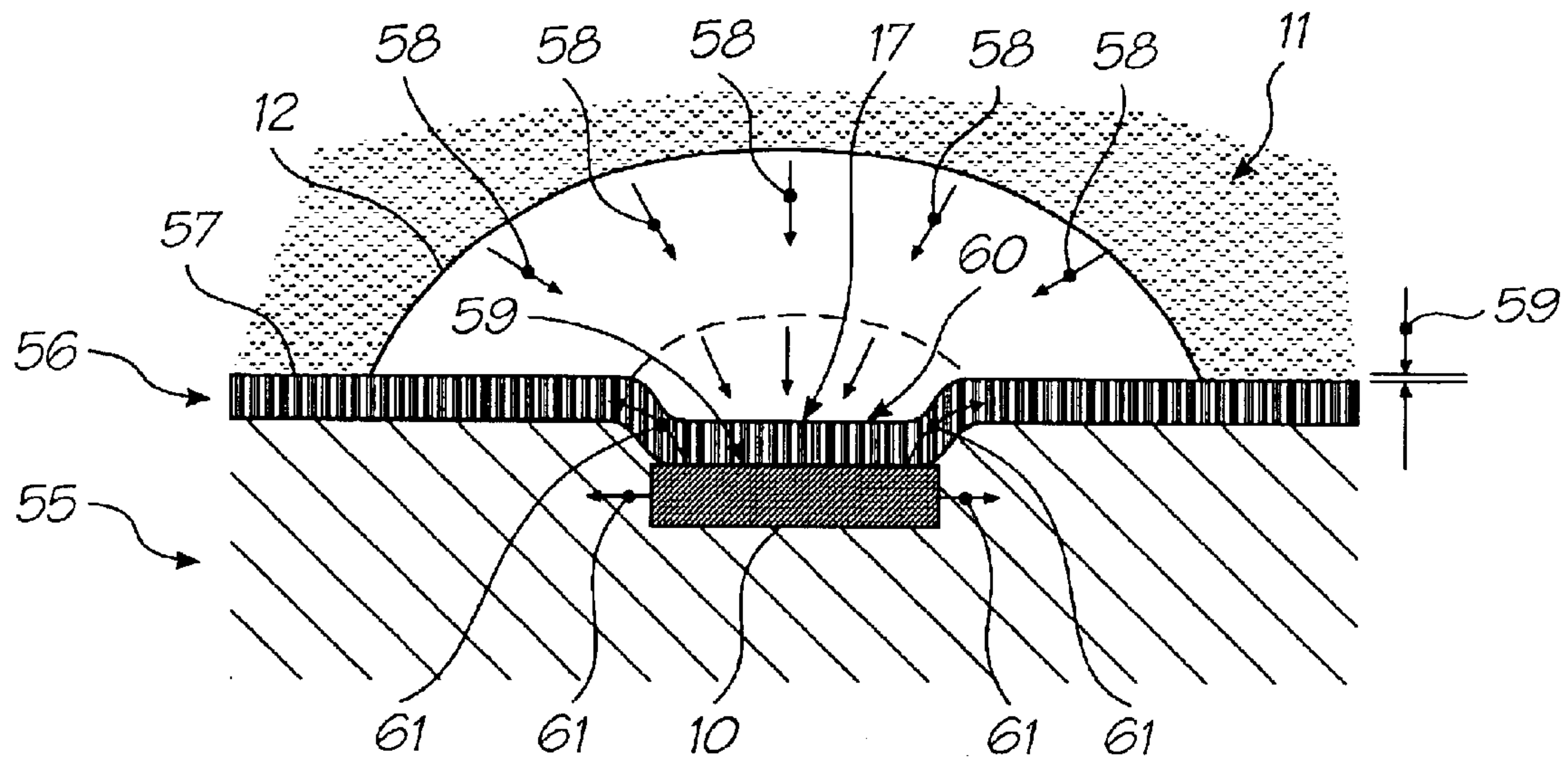
FIG. 47 (PRIOR ART)
