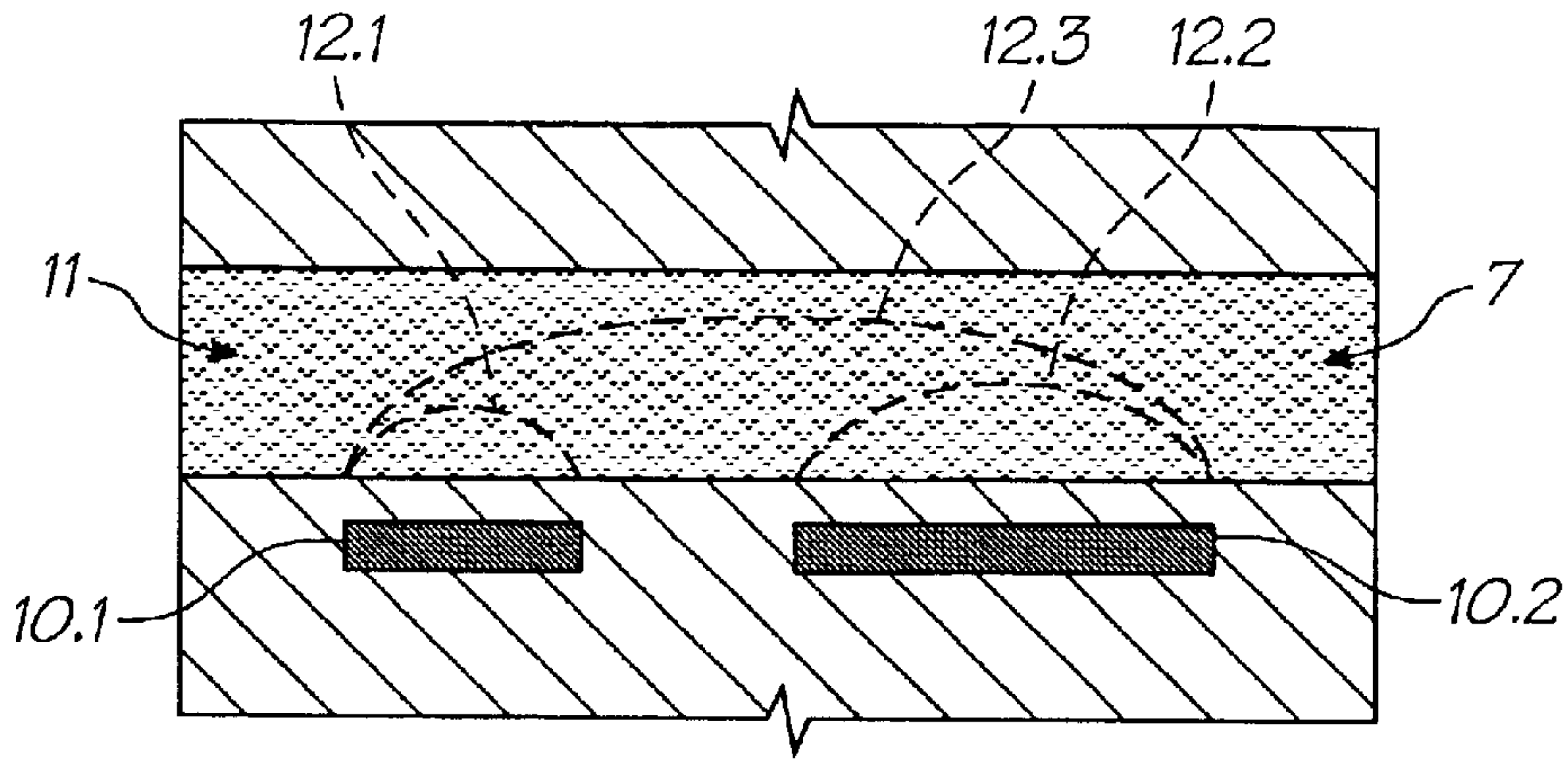
FIG. 52 (PRIOR ART)
