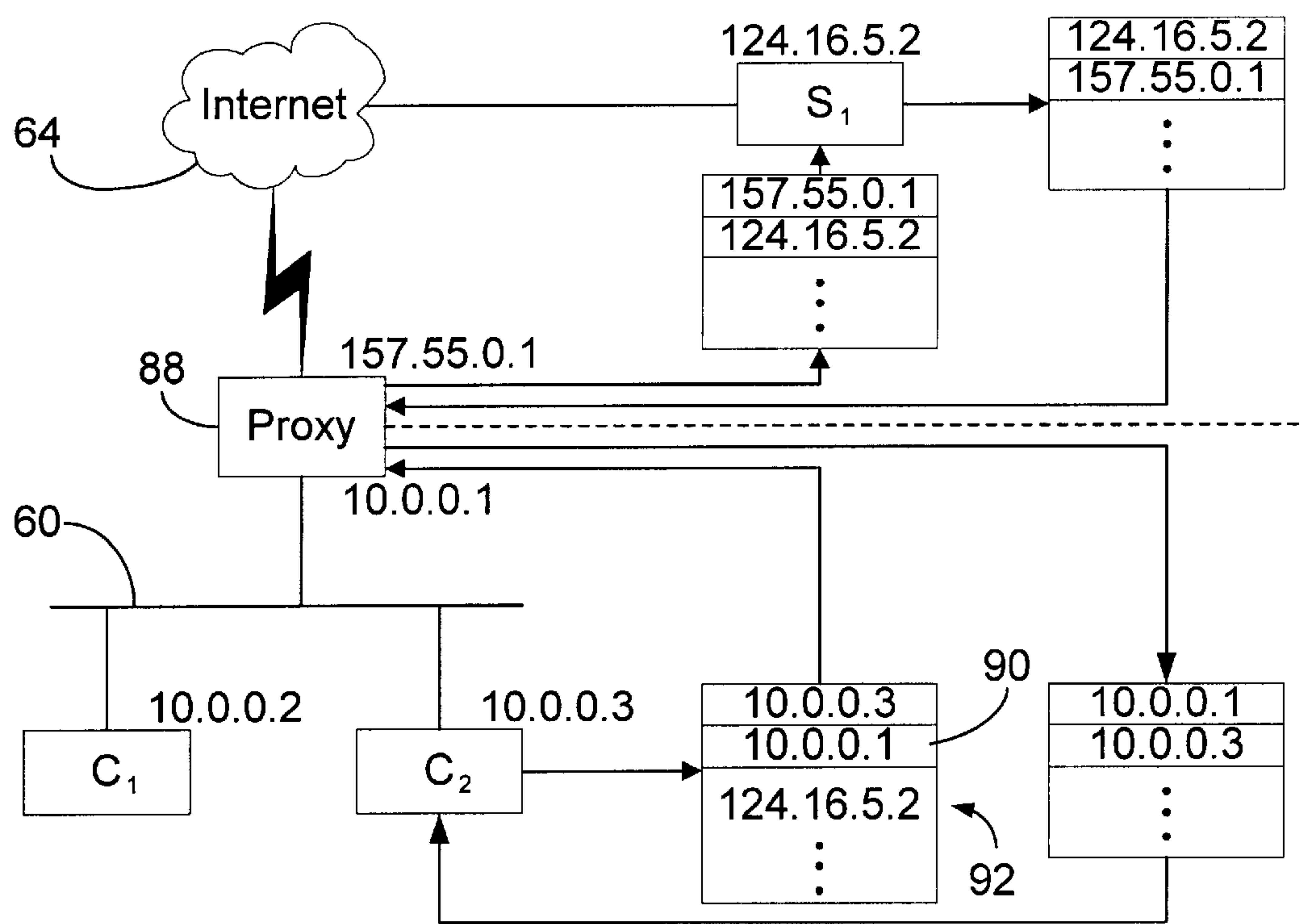
FIG. 6 (PRIOR ART)
