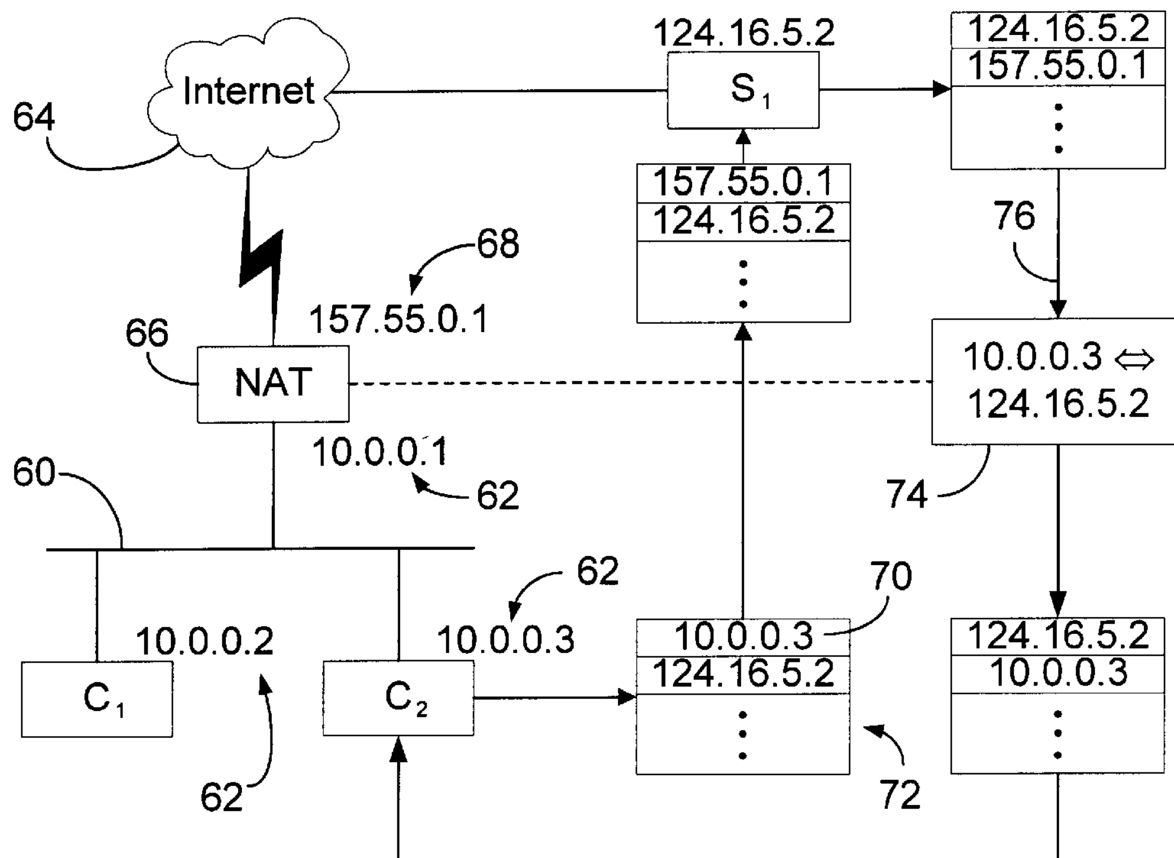
FIG. 2 (PRIOR ART)
