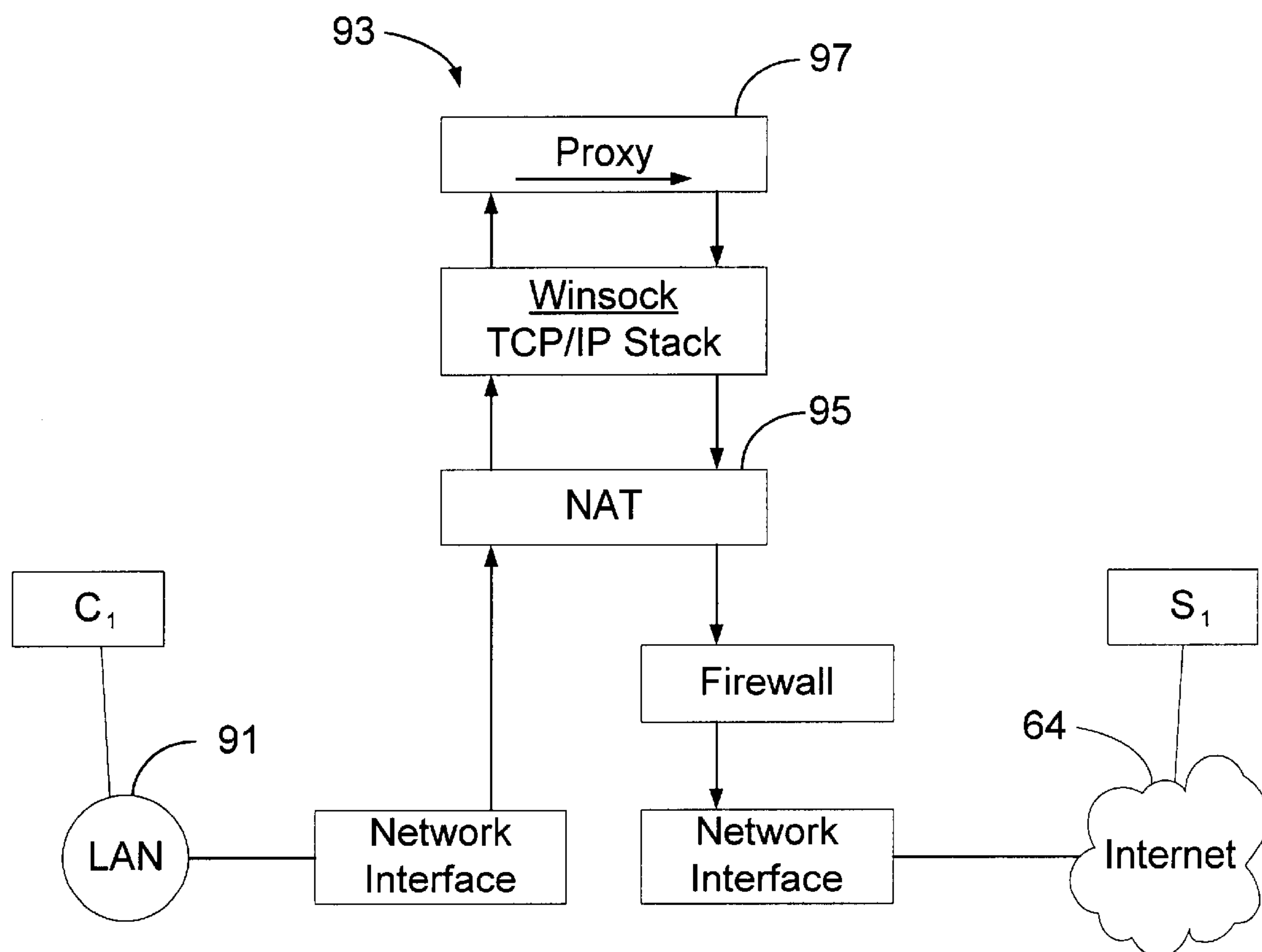
FIG. 7 (PRIOR ART)
