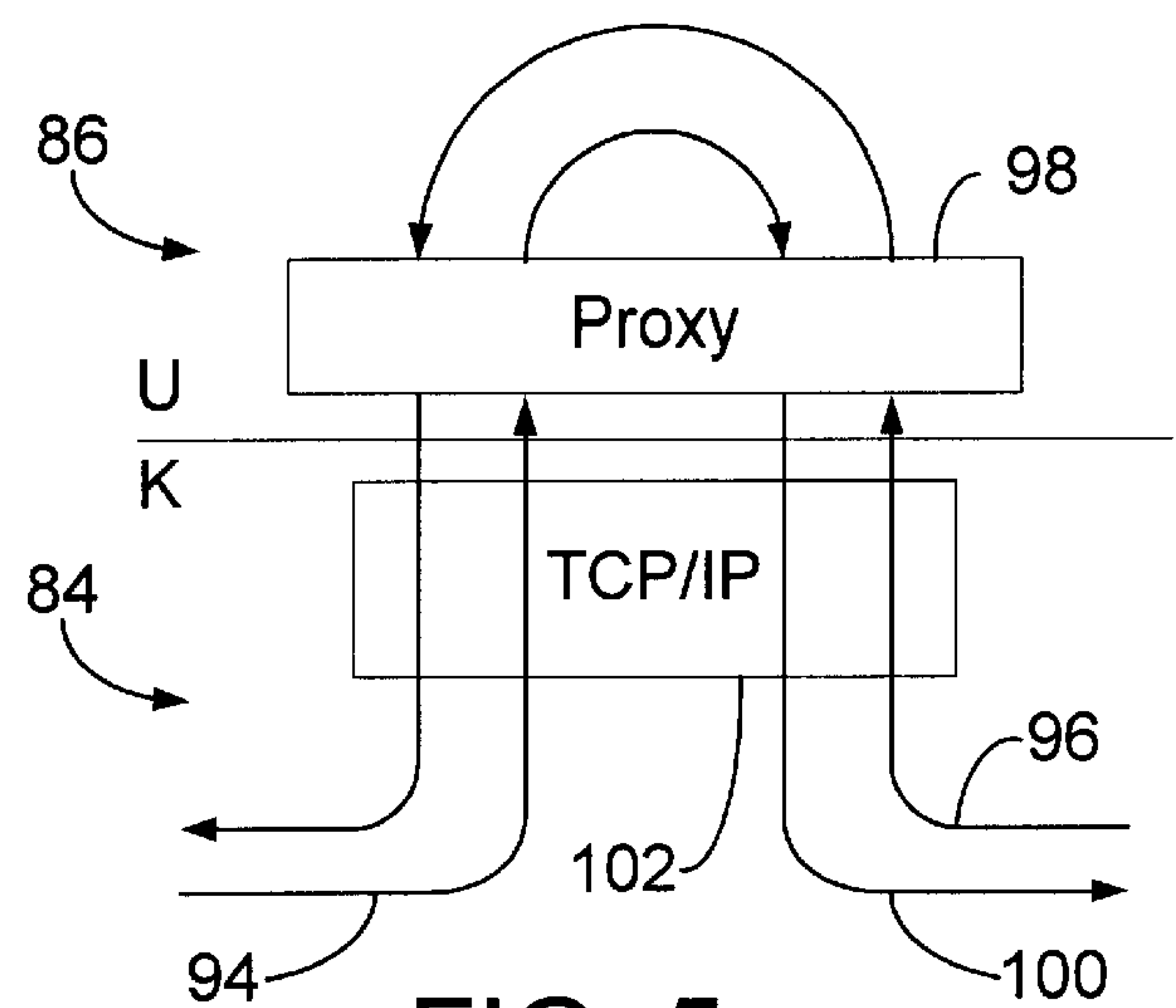
FIG. 5 (PRIOR ART)
