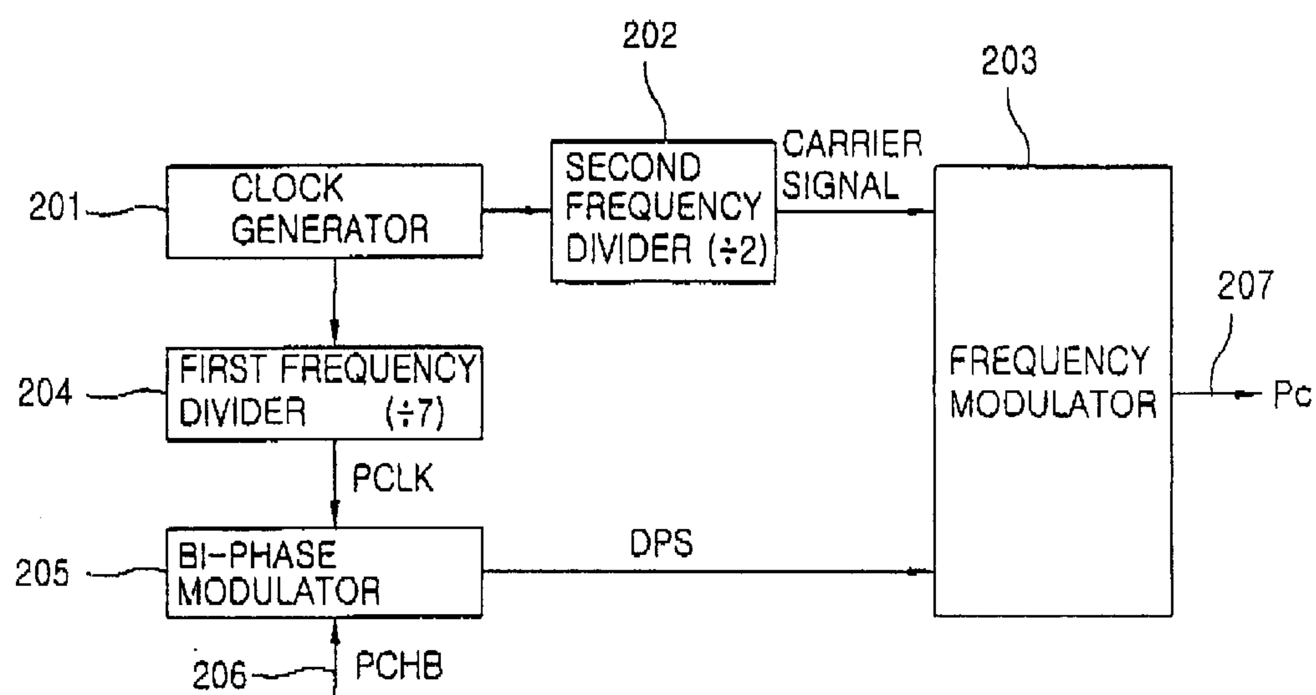
FIG. 2 CONVENTIONAL ART
