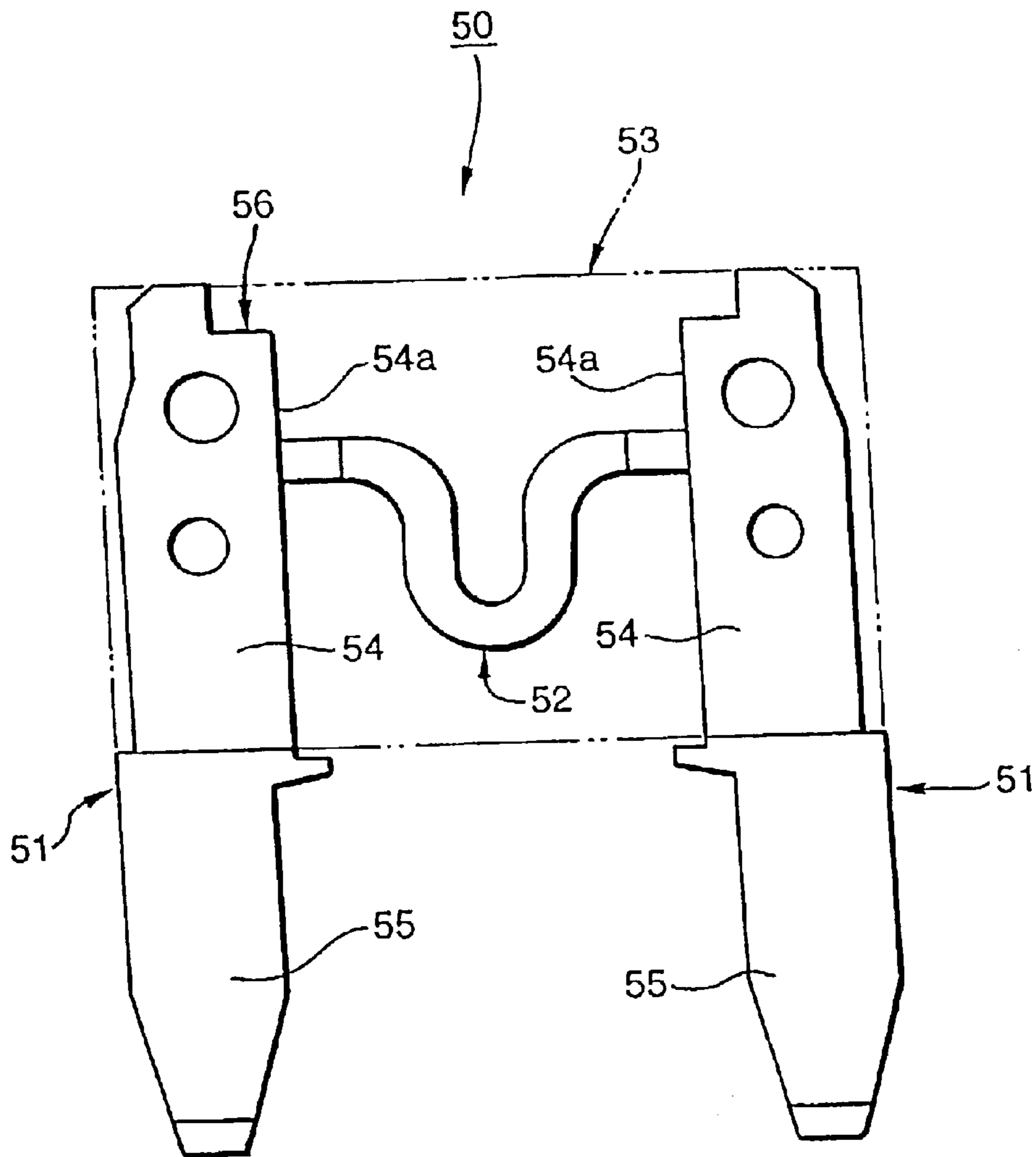
FIG. 7 PRIOR ART
