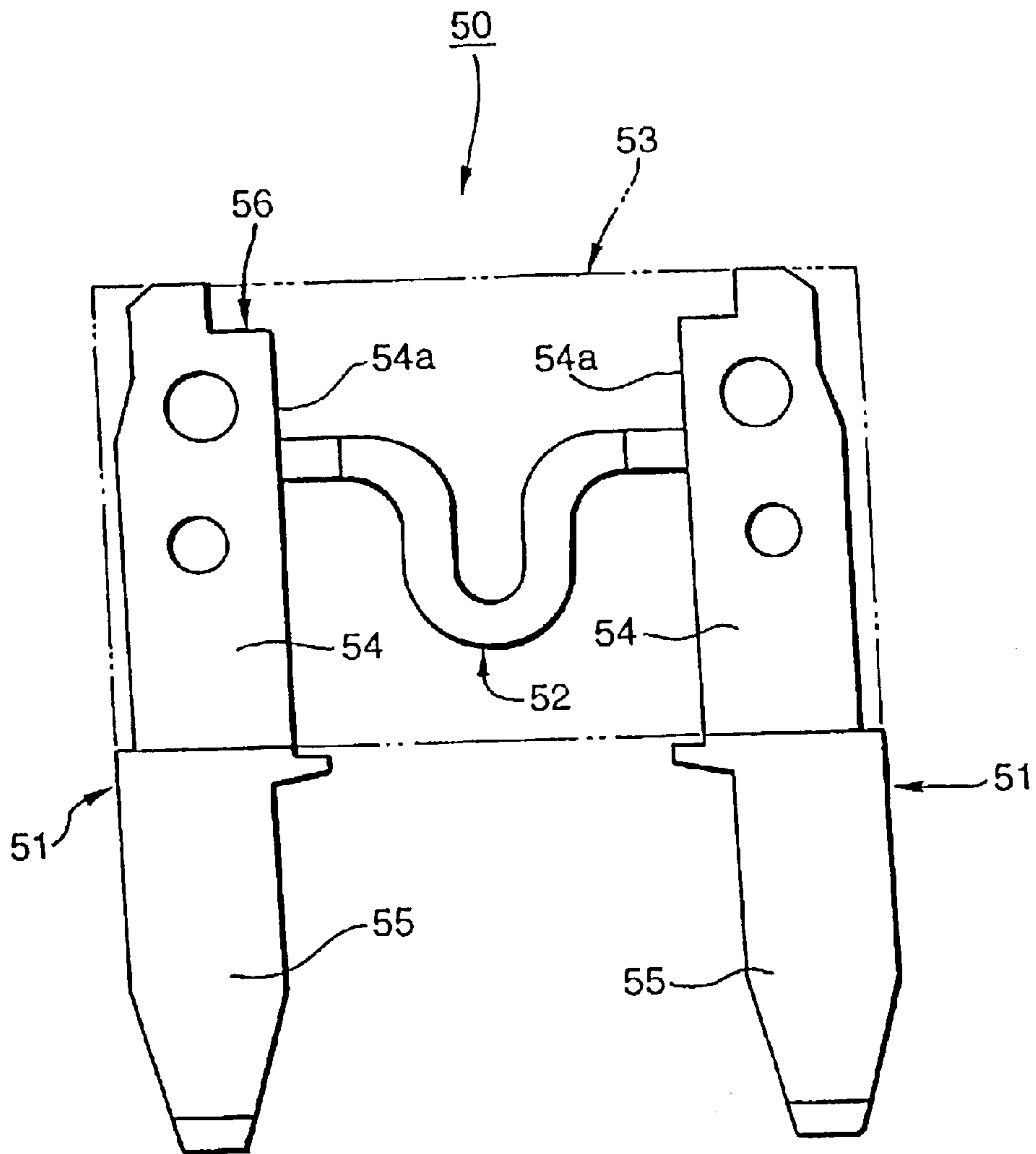
FIG. 7 PRIOR ART
