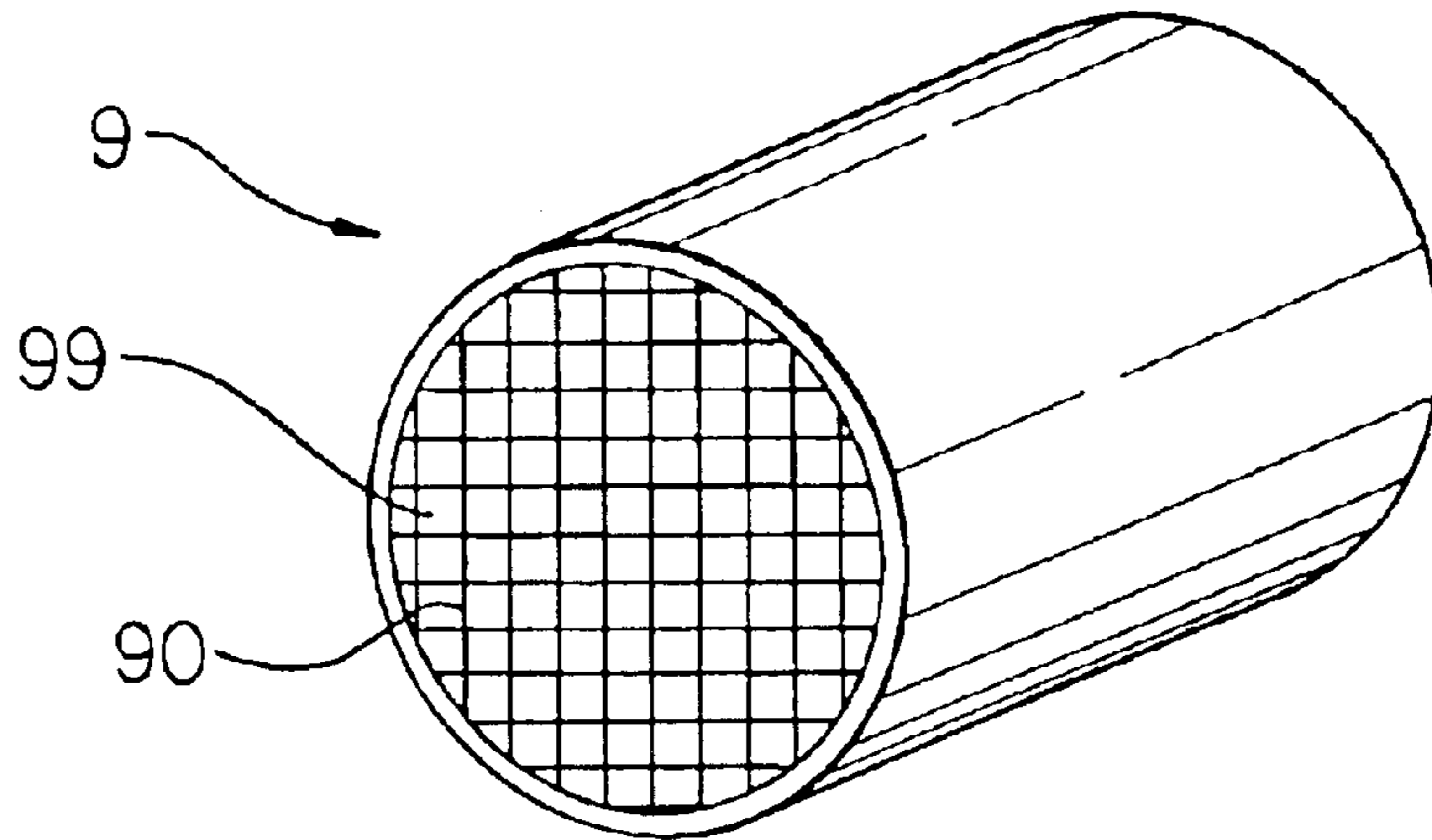
Fig. 6 (PRIOR ART)
