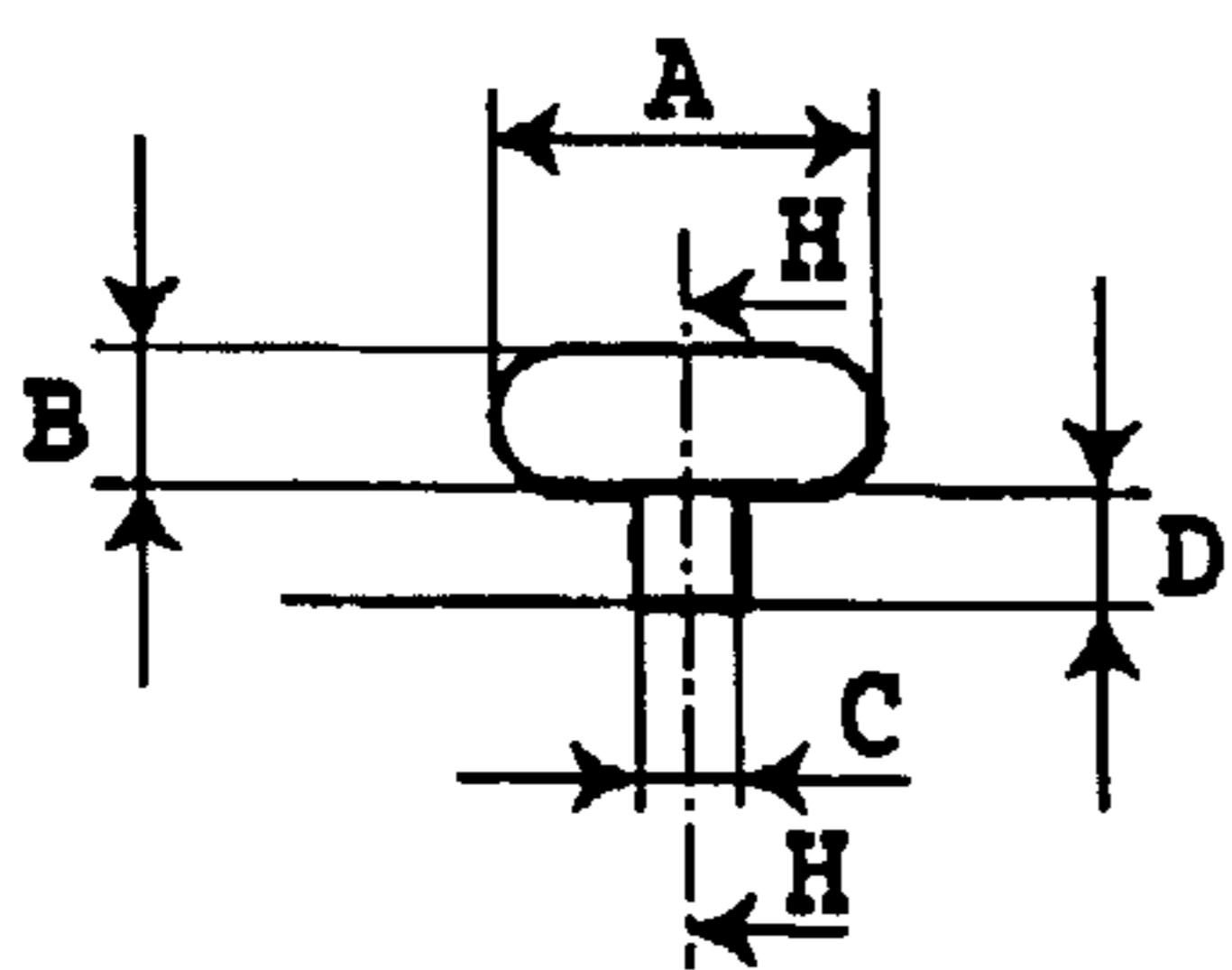
G DETAILED VIEW
