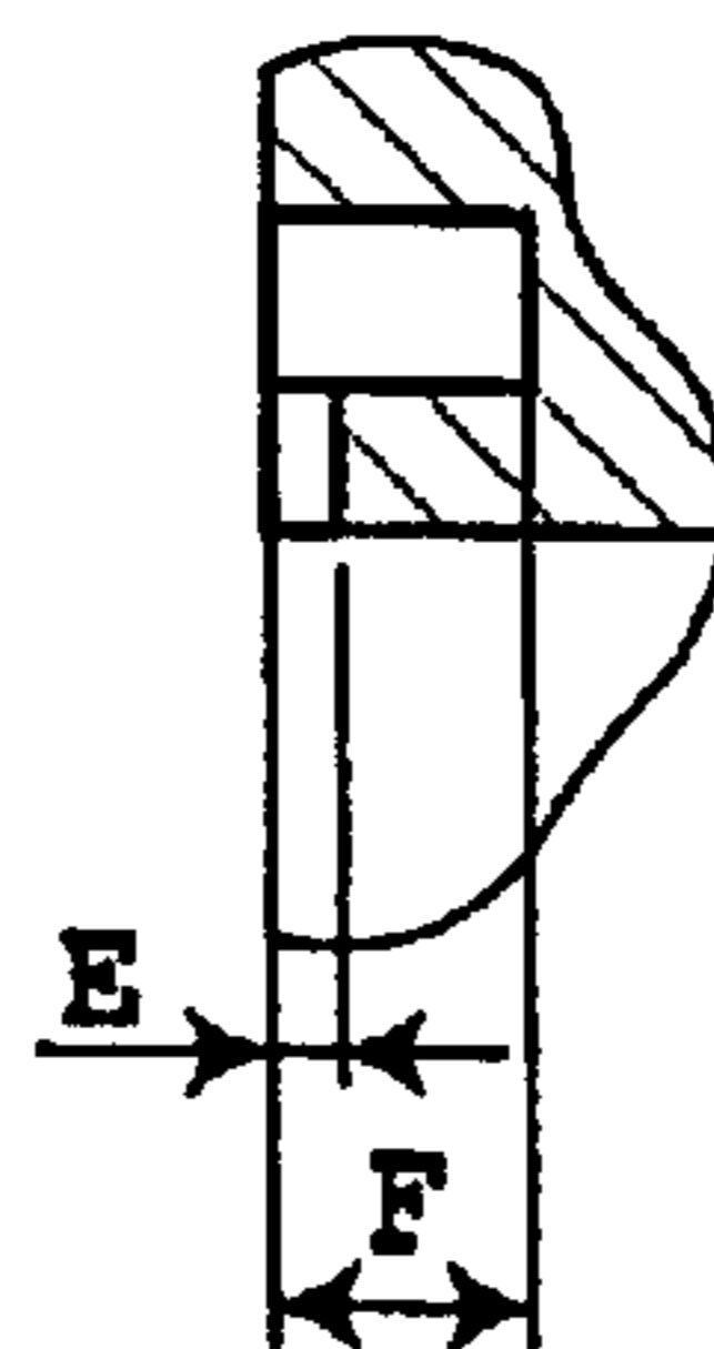
H-H SECTIONAL VIEW
