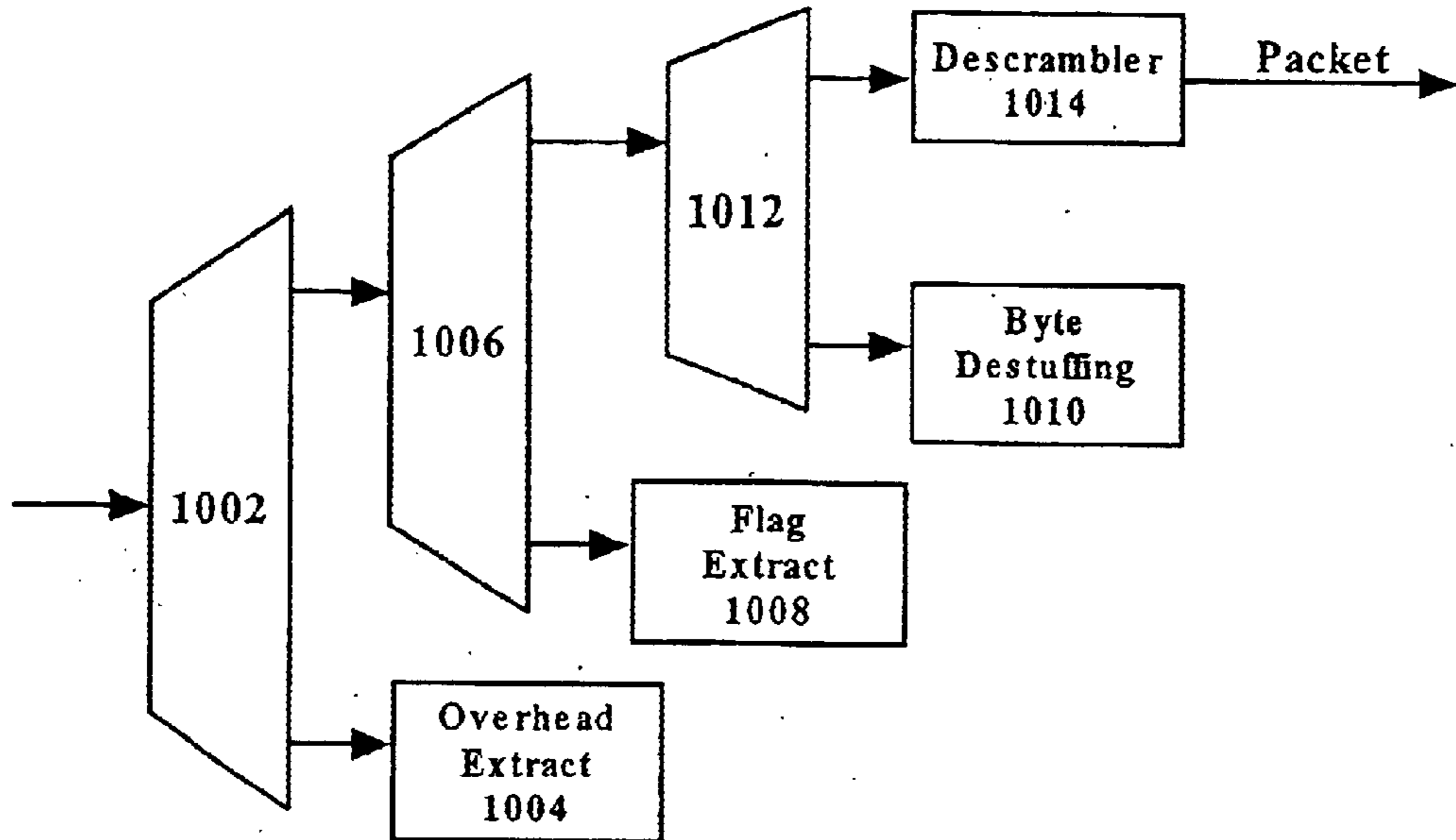
FIG. 10 (PRIOR ART)
