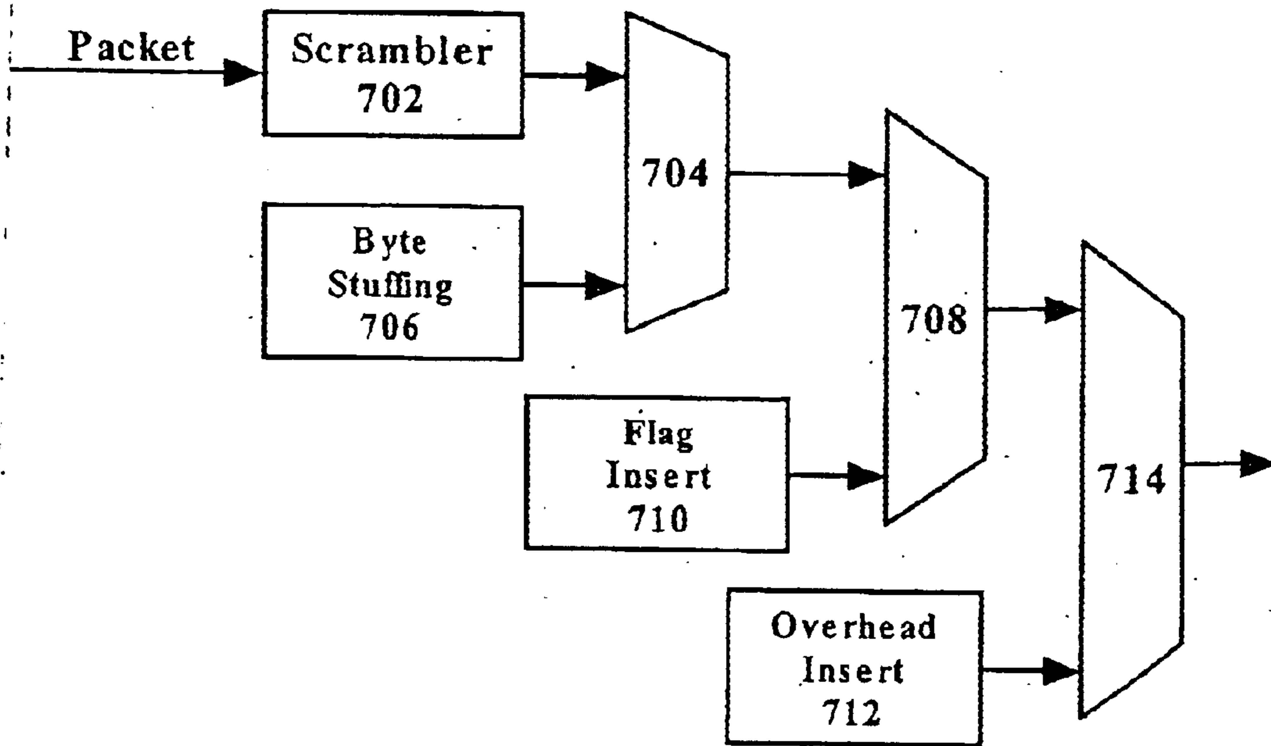
FIG. 7 (PRIOR ART)
