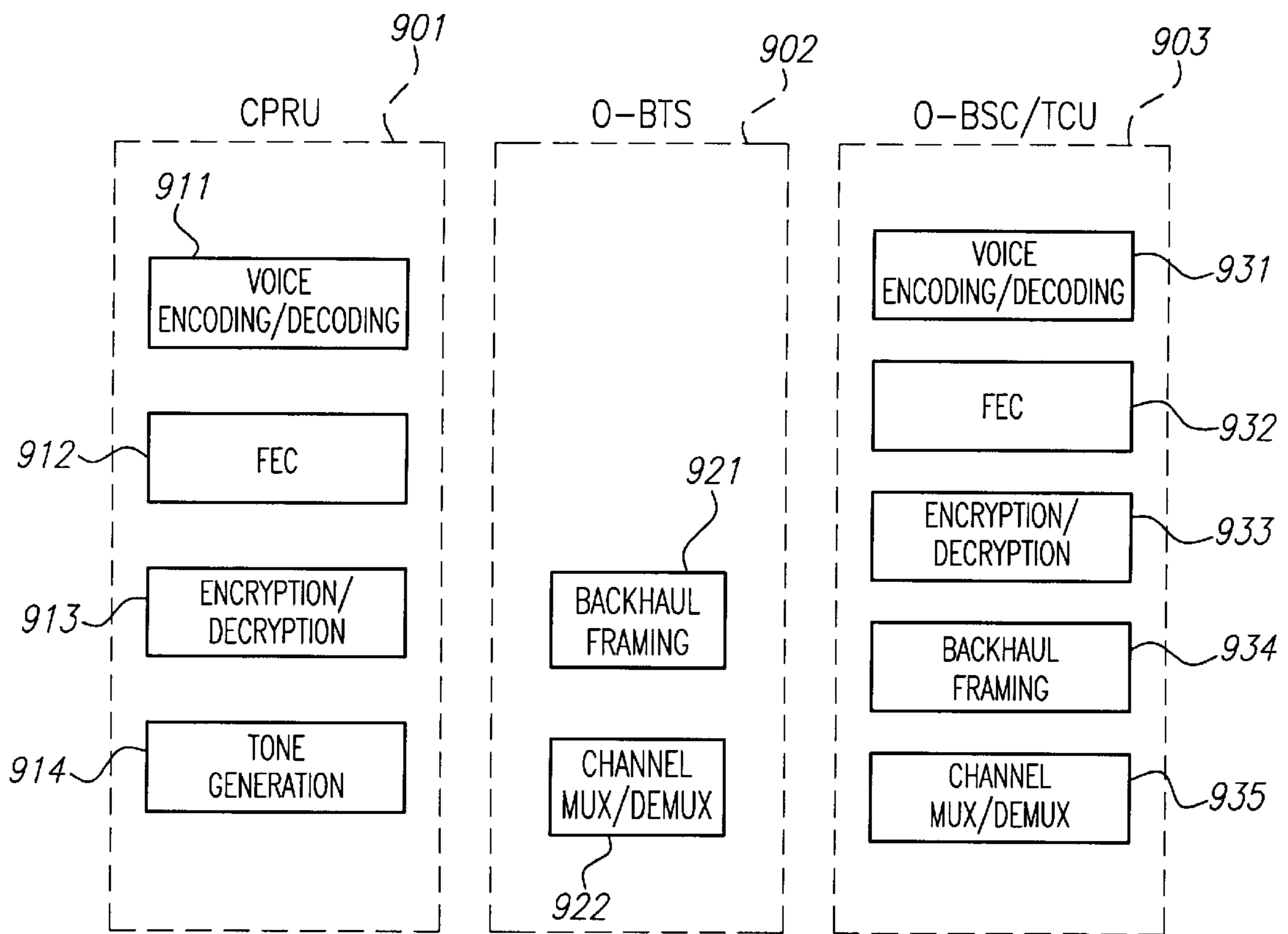
BEARER PATH FUNCTIONS
