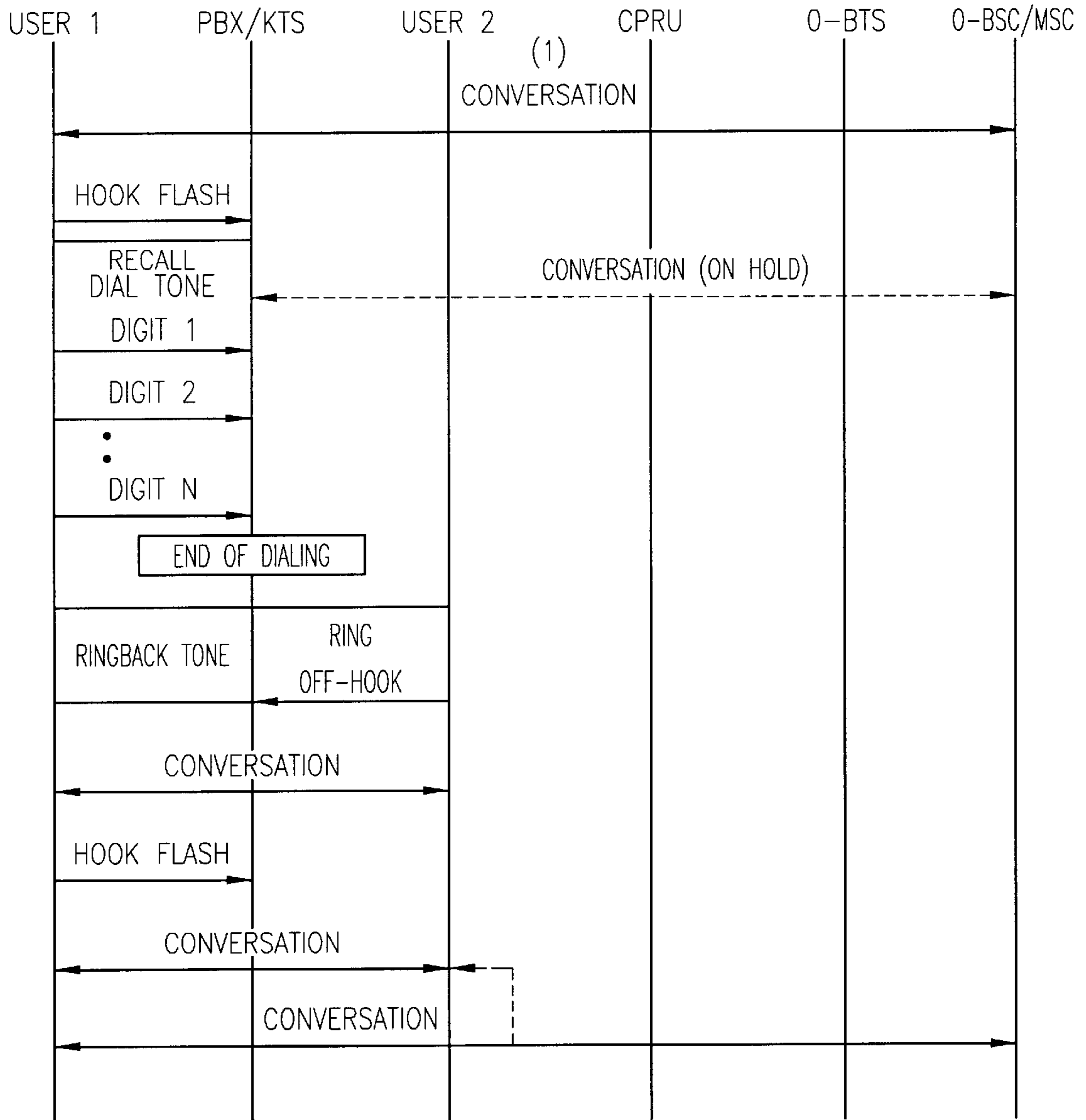
THREE-WAY CALL SETUP SCENARIO
