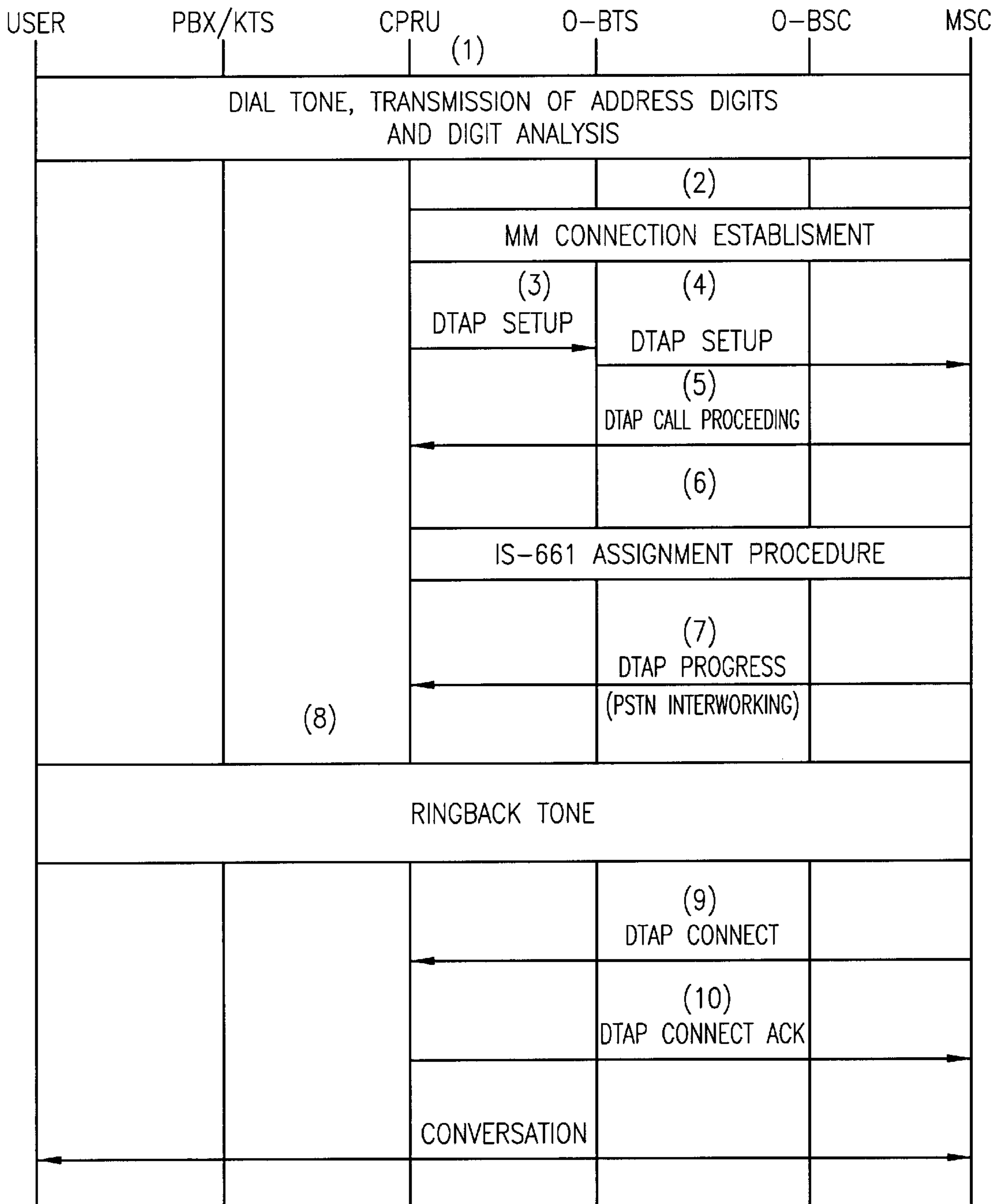
SUCCESSFUL OUTGOING CALL SETUP (PSTN INTERWORKING)
