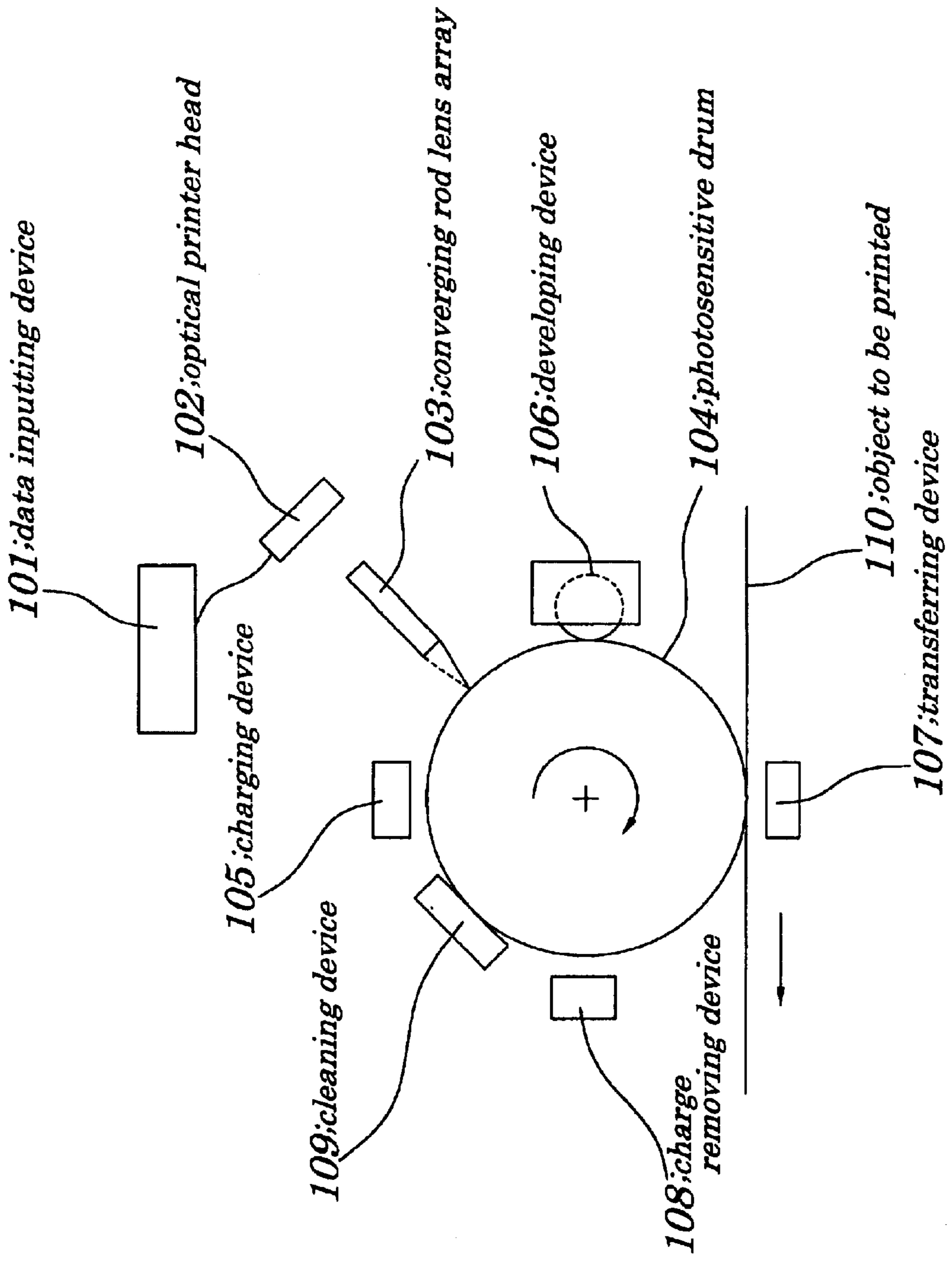
FIG. 13 (PRIOR ART)
