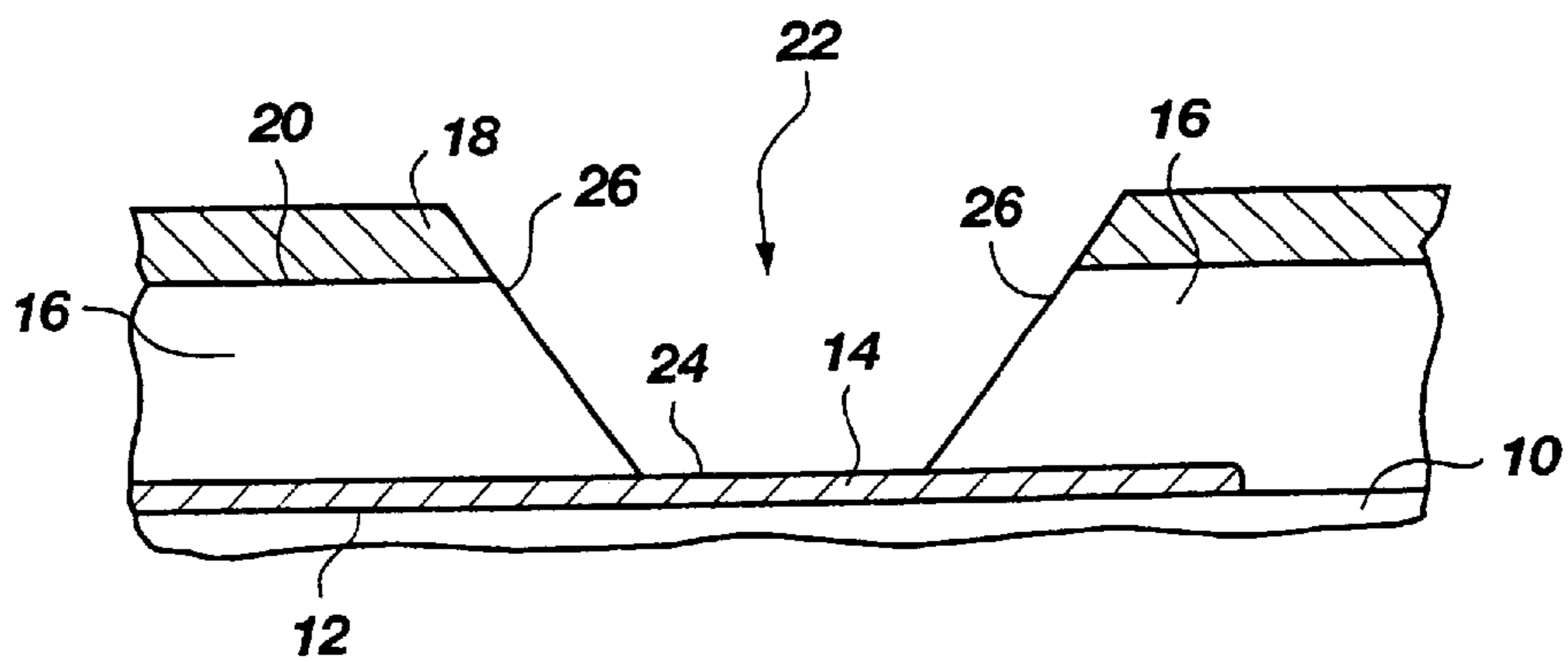
Fig. 1c (PRIOR ART)
