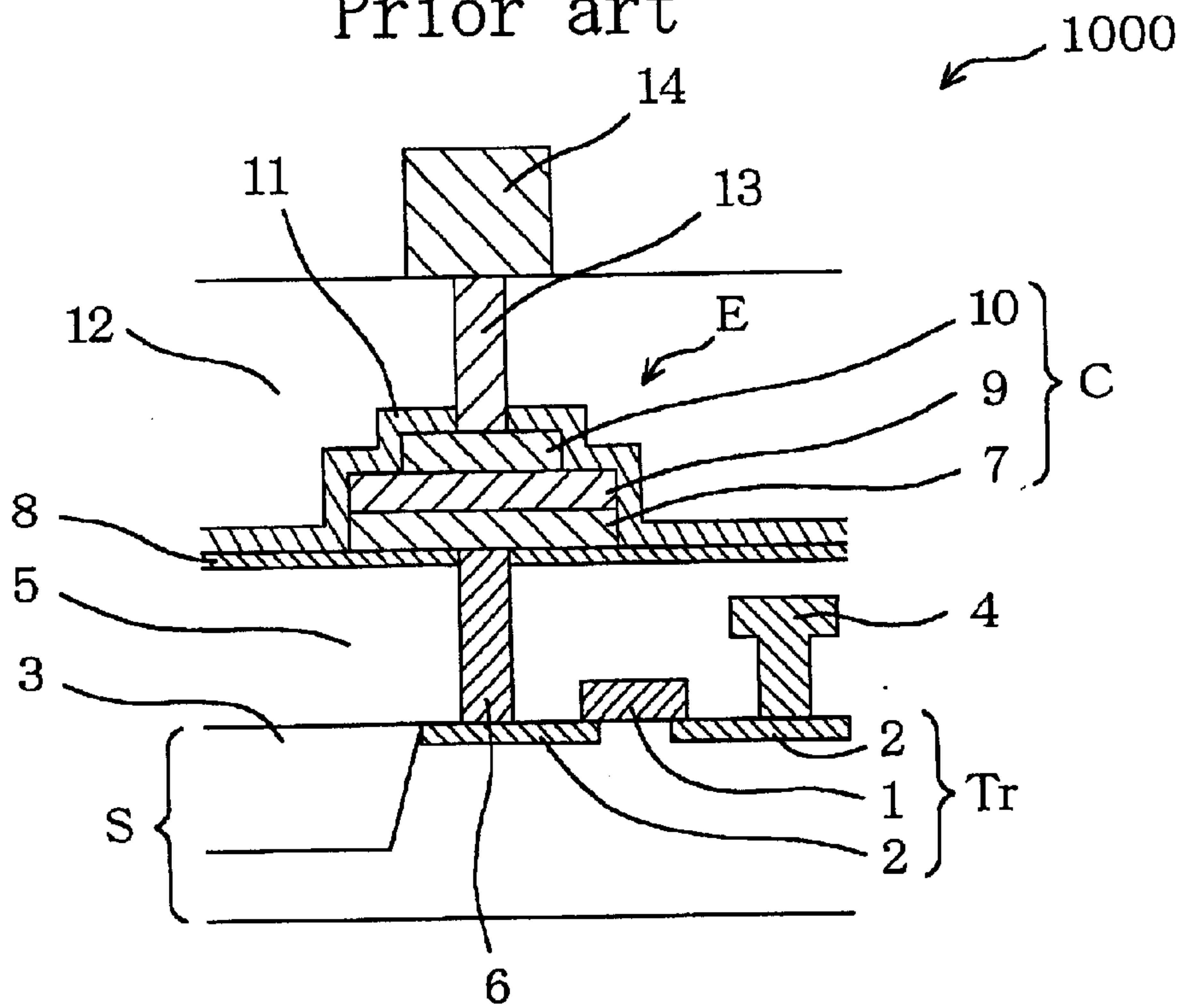
Fig. 17 Prior art
