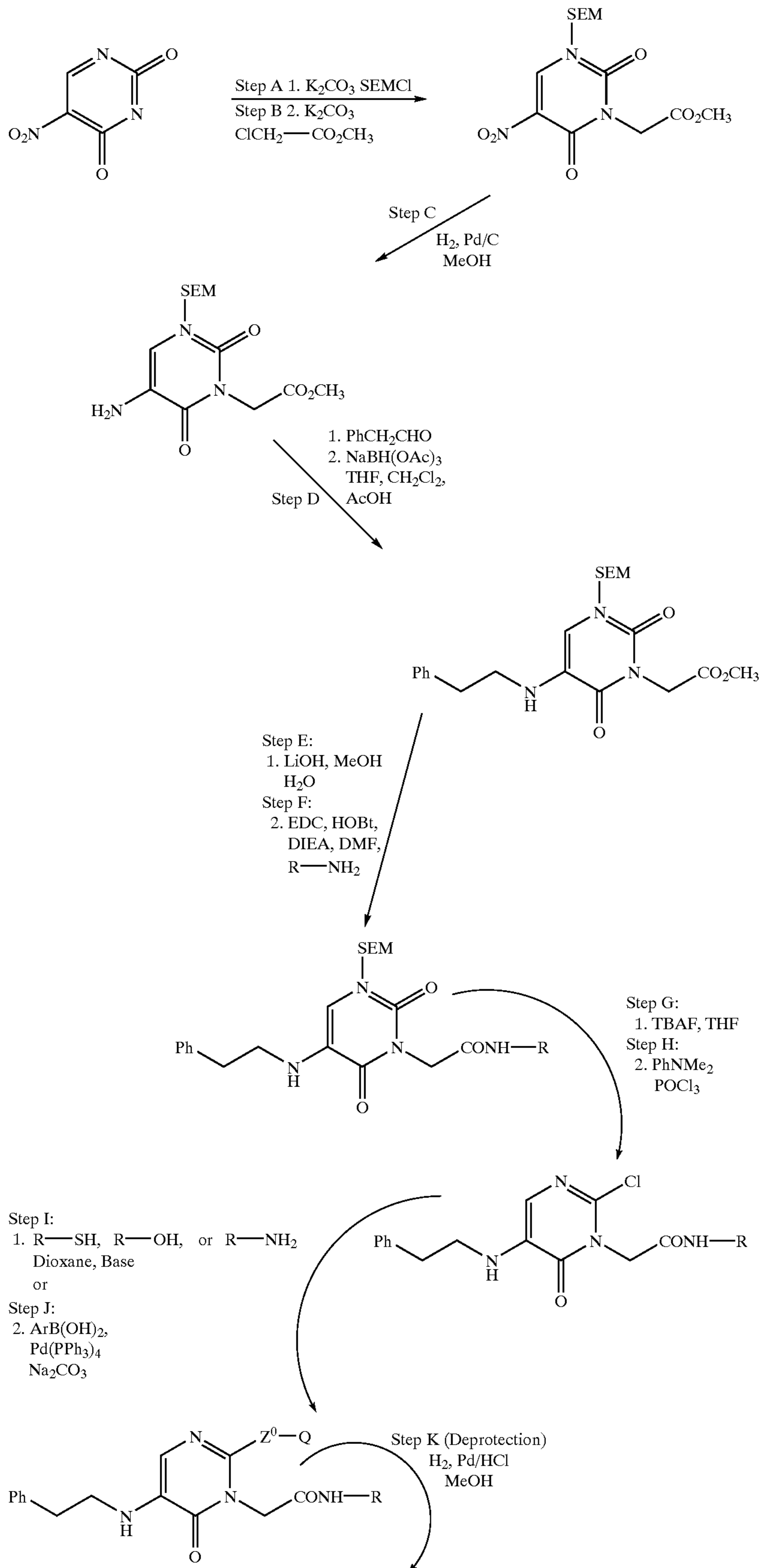
Scheme 6. Preparation of 2-Substituted Pyrimidinones
