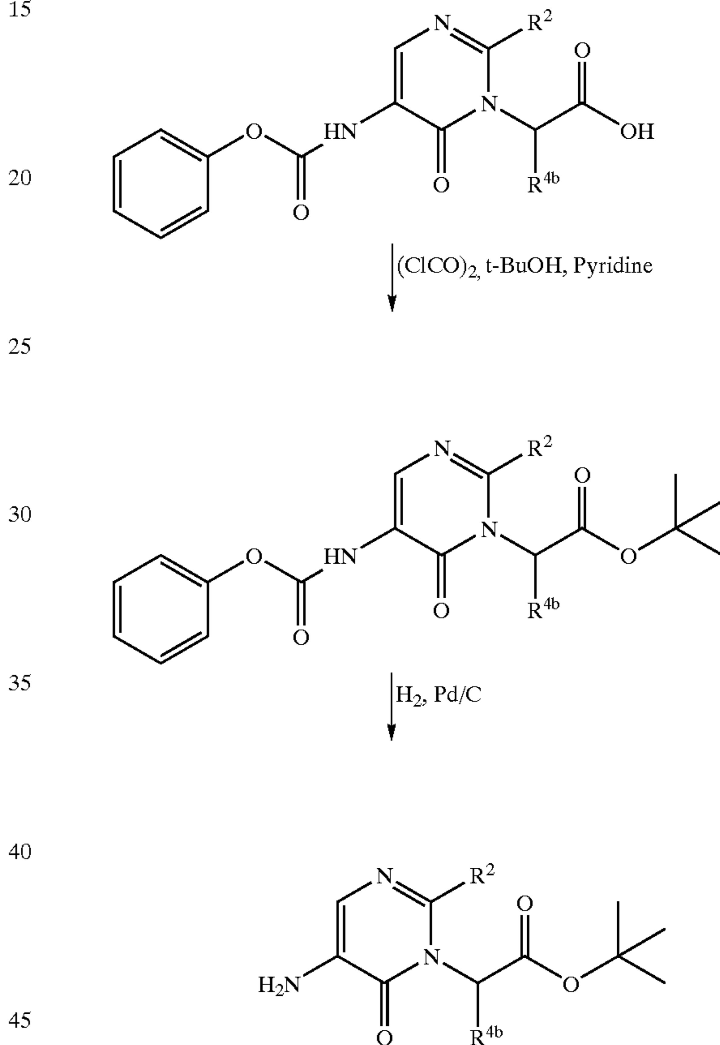
Scheme 2: General Pyrimidinone Synthesis-I (Continued)
