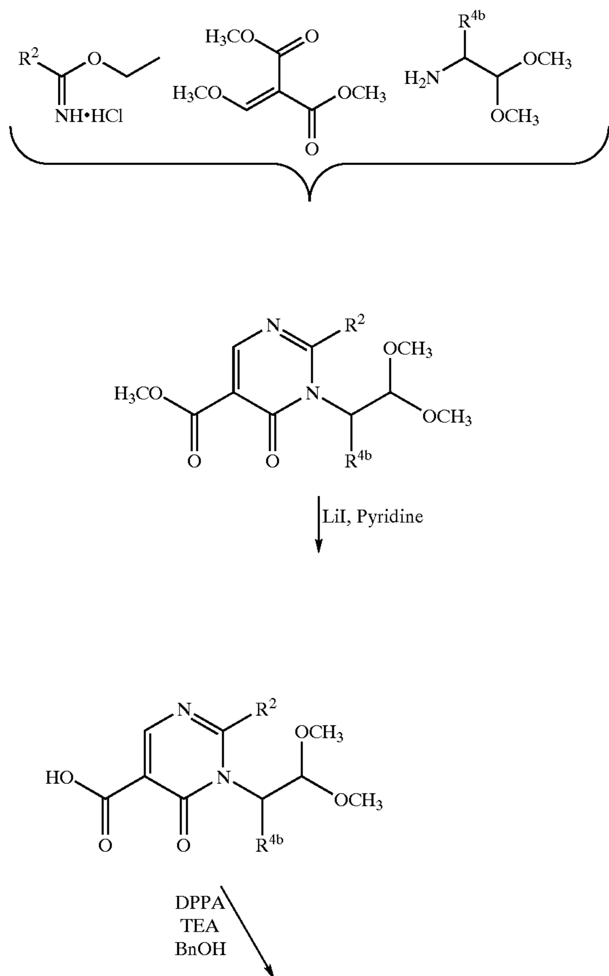
Scheme 1: General Pyrimidinone Synthesis-I
