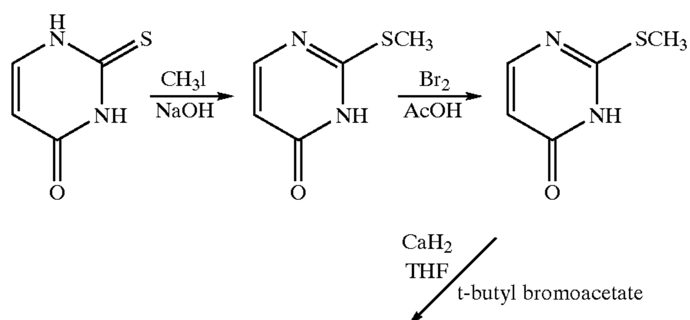
Scheme 7: Alternate Pyrimidinone Synthesis
