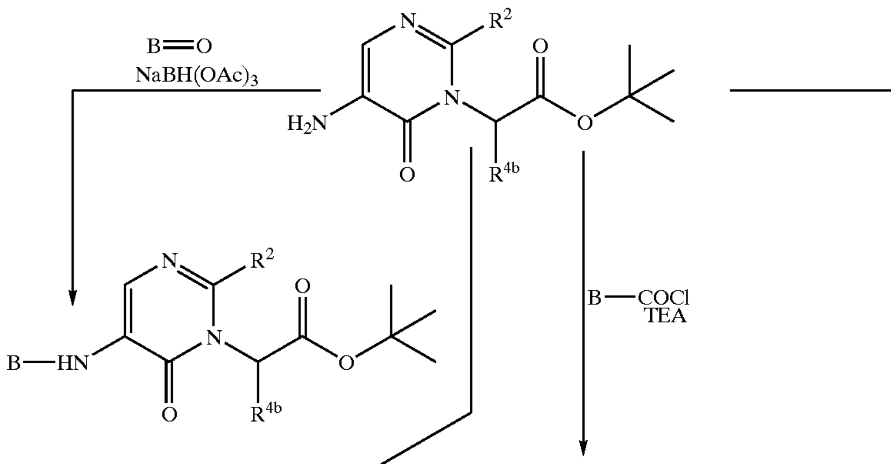
Scheme 3: General Pyrimidinone Synthesis-I (Continued)
