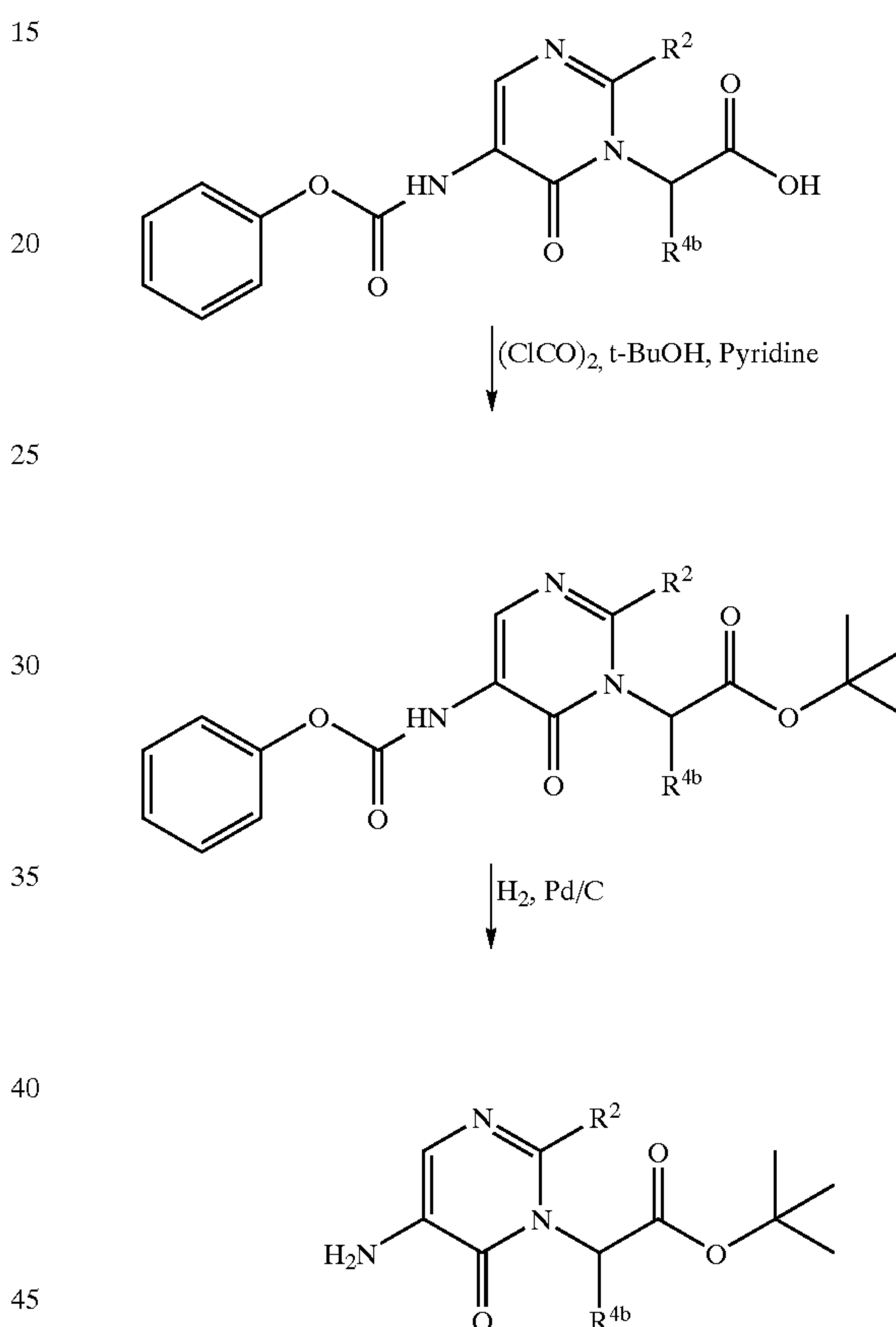
Scheme 2: General Pyrimidinone Synthesis-I (Continued)
