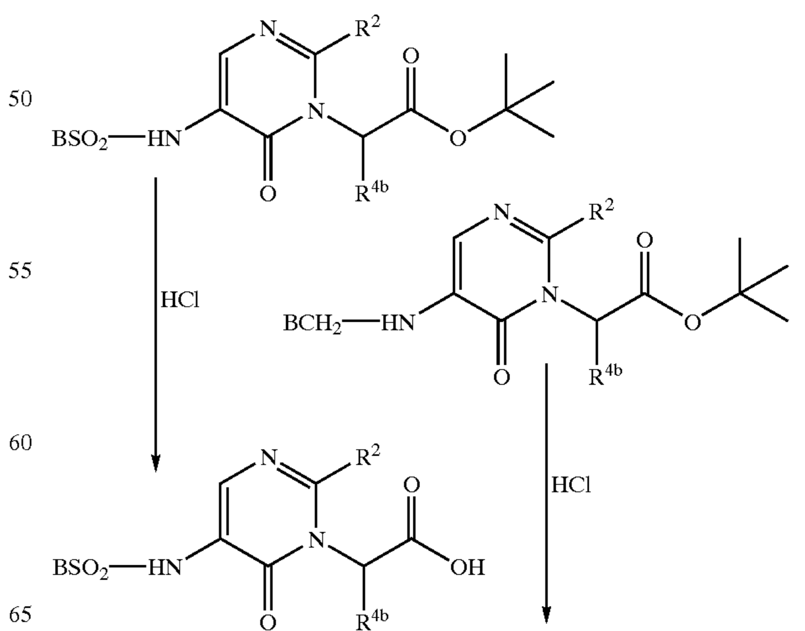
Scheme 5: General Pyrimidinone Synthesis-I (Concluded)
