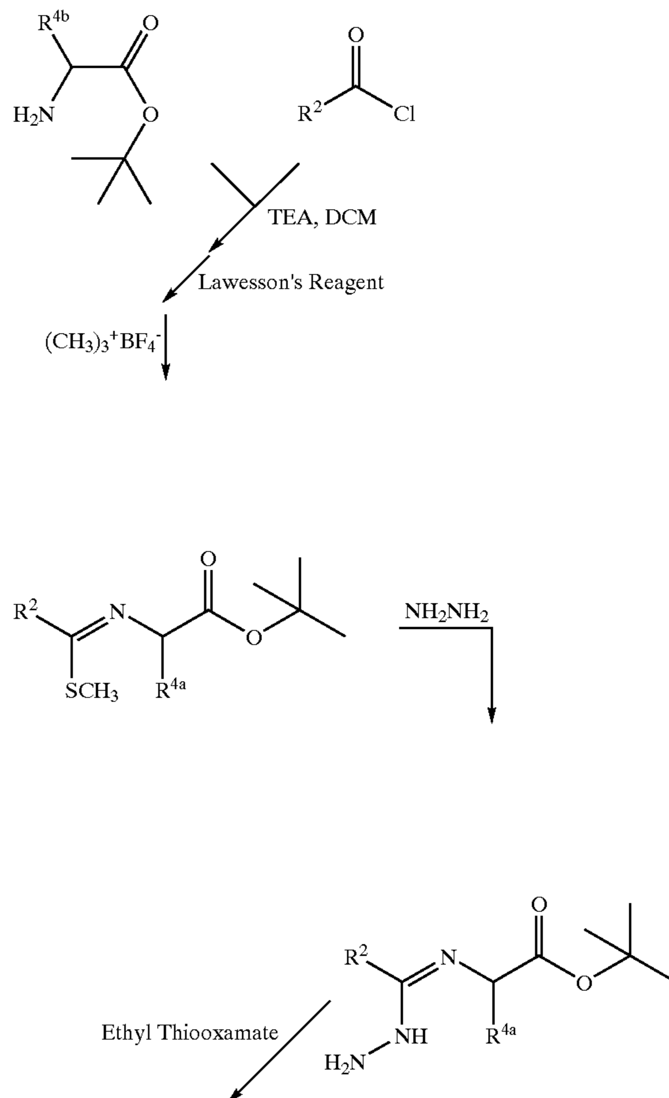
Scheme 9: General 4-AzaPyrimidinone Synthesis
