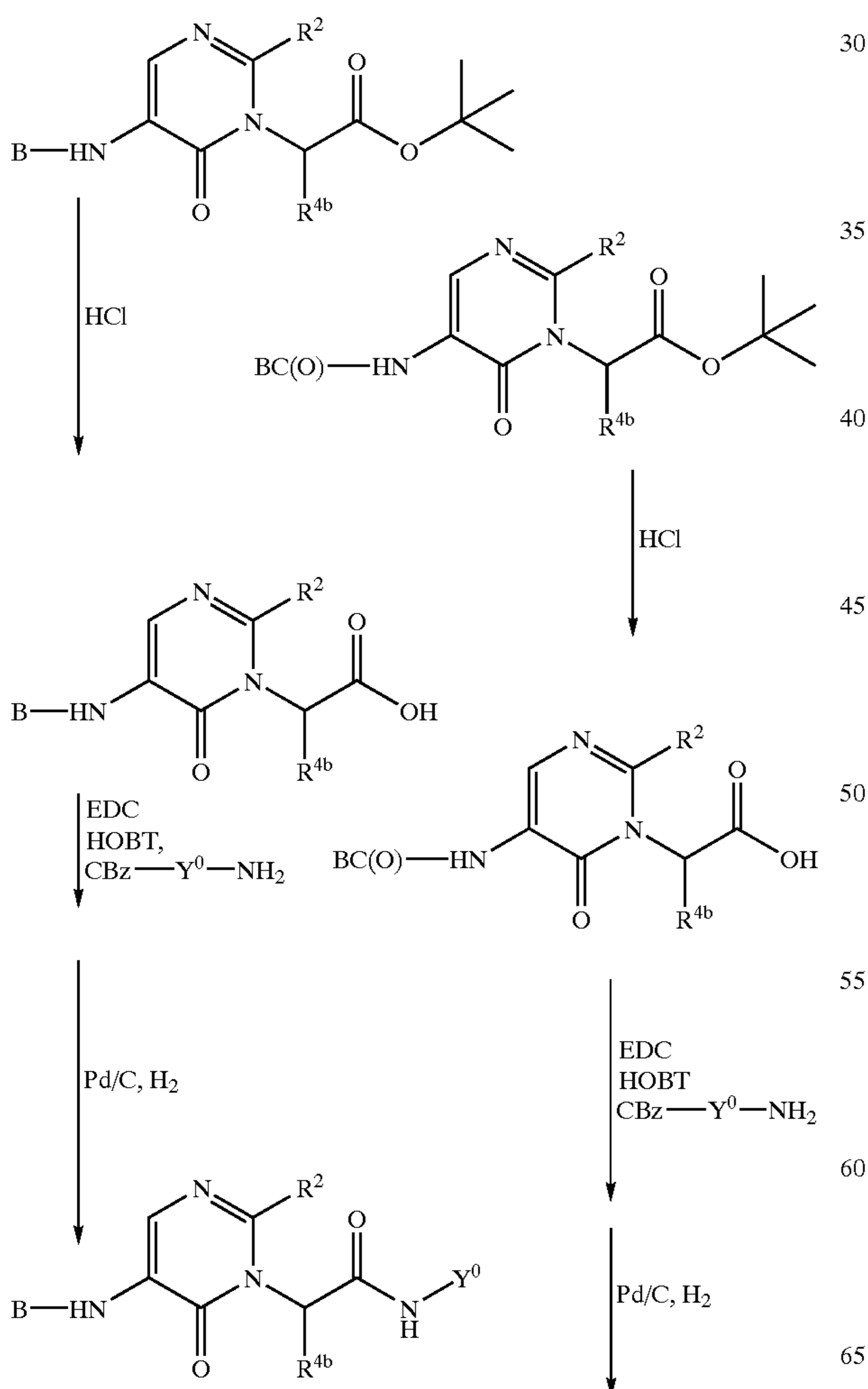
Scheme 4: General Pyrimidinone Synthesis-I (Concluded)
