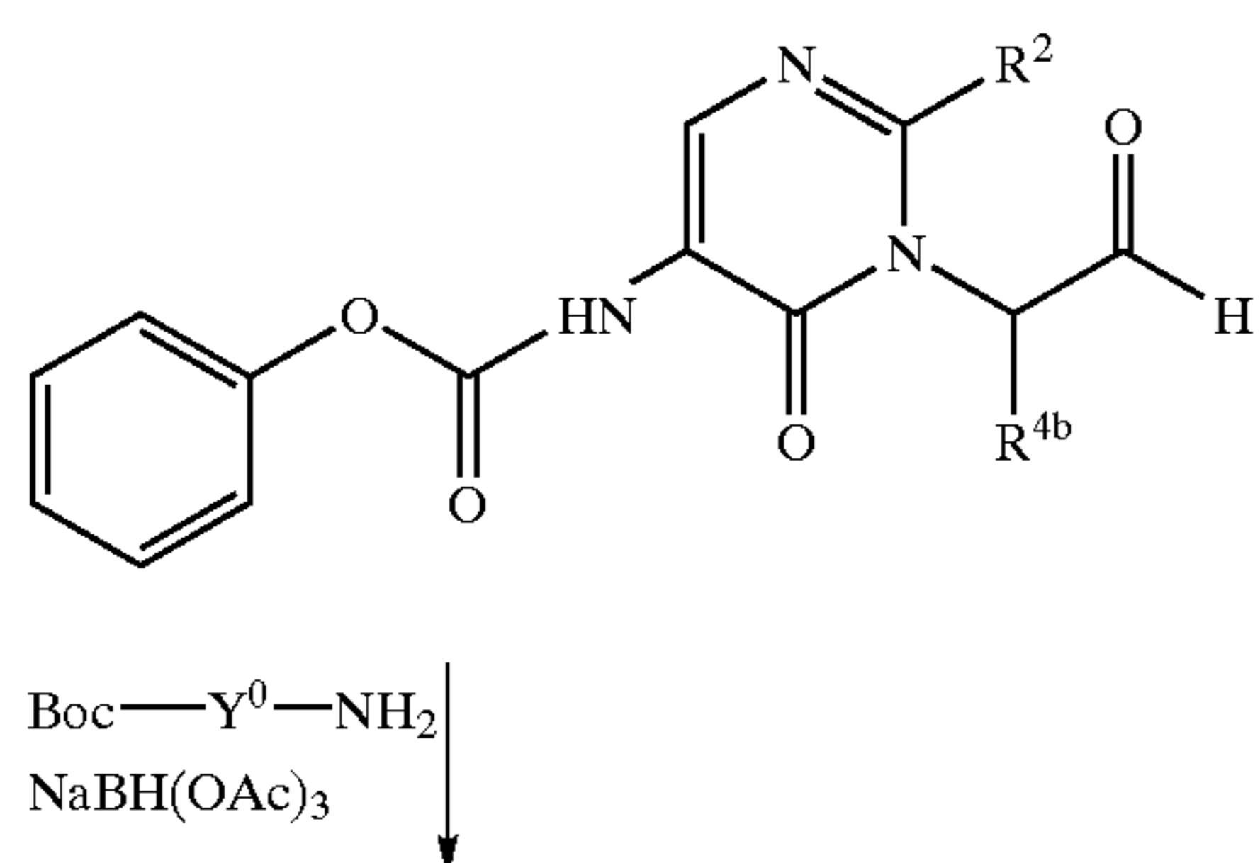
Scheme 8: General Methylene Pyrimidinone Synthesis
