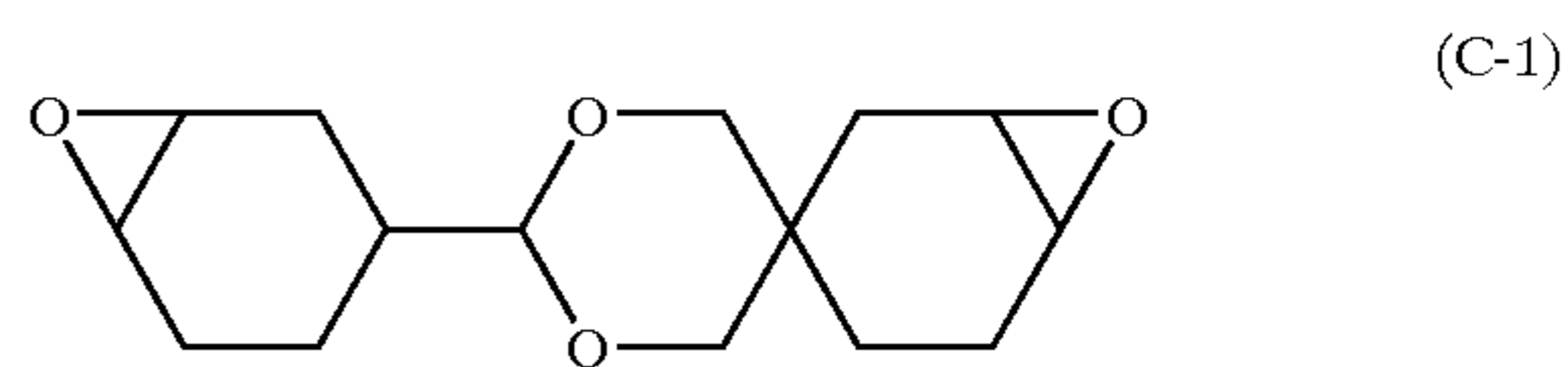
2(3,4-Epoxy)cyclohexyl-5,5-spiro-3,4-epoxycyclohexane-meta-dioxane (ERL-4234)
