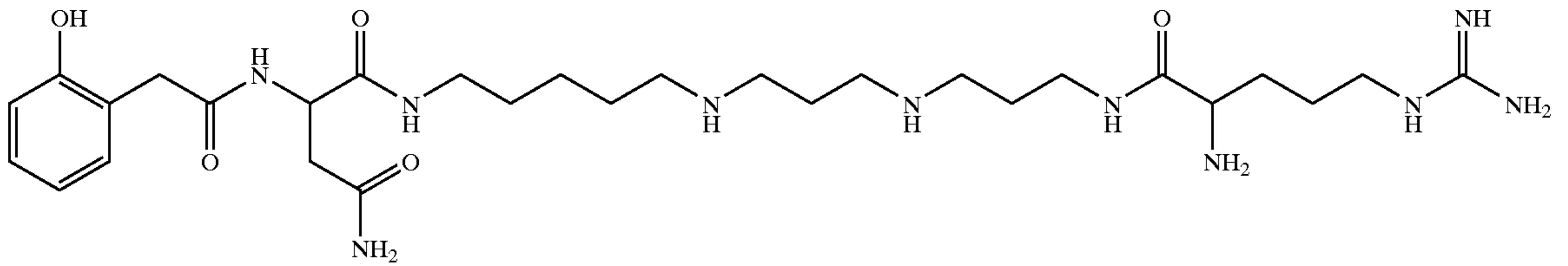
Compound 11
