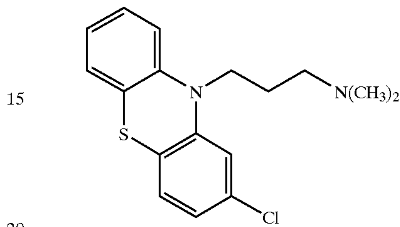
Chlorpromazine
