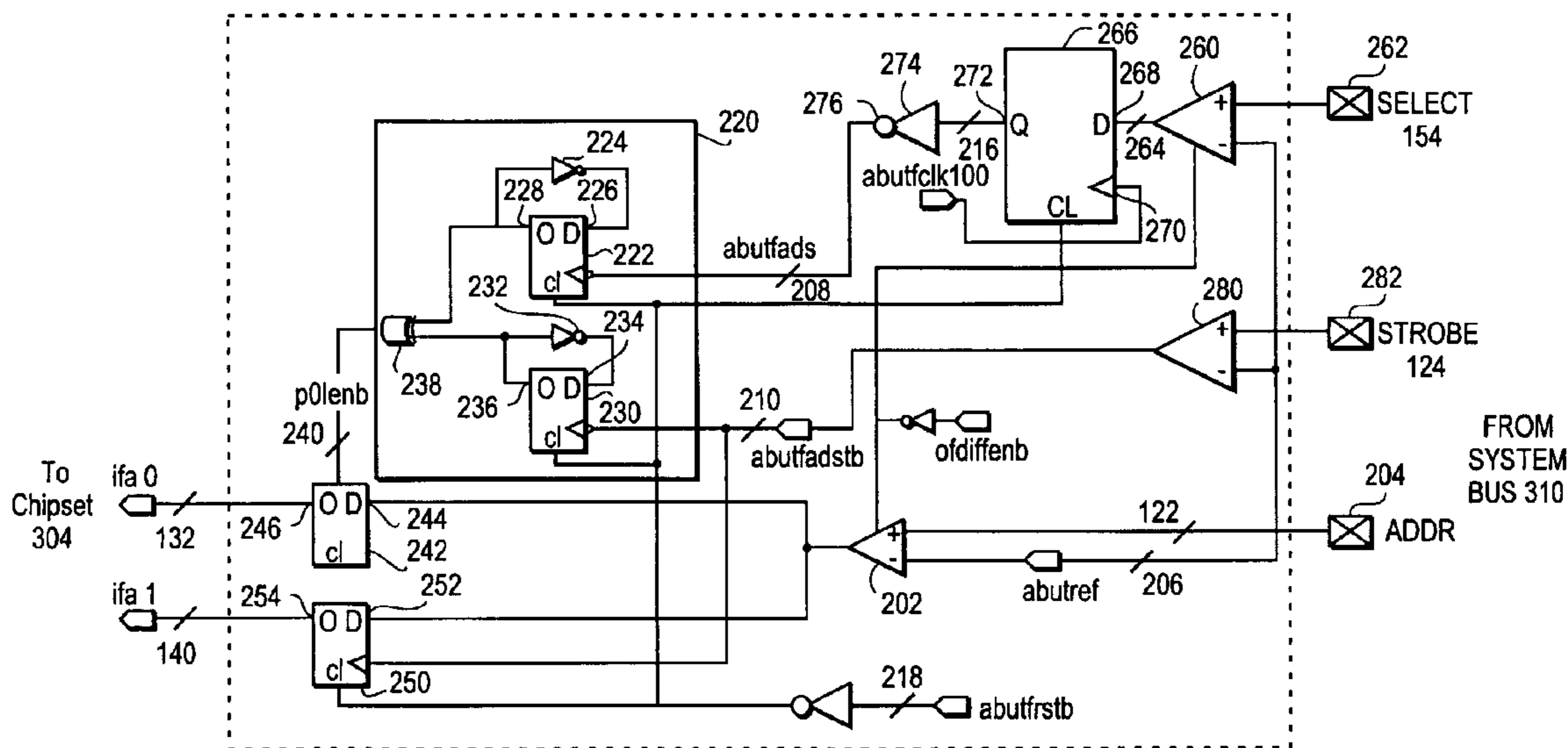
Source Synchronous Address Receiver 200
