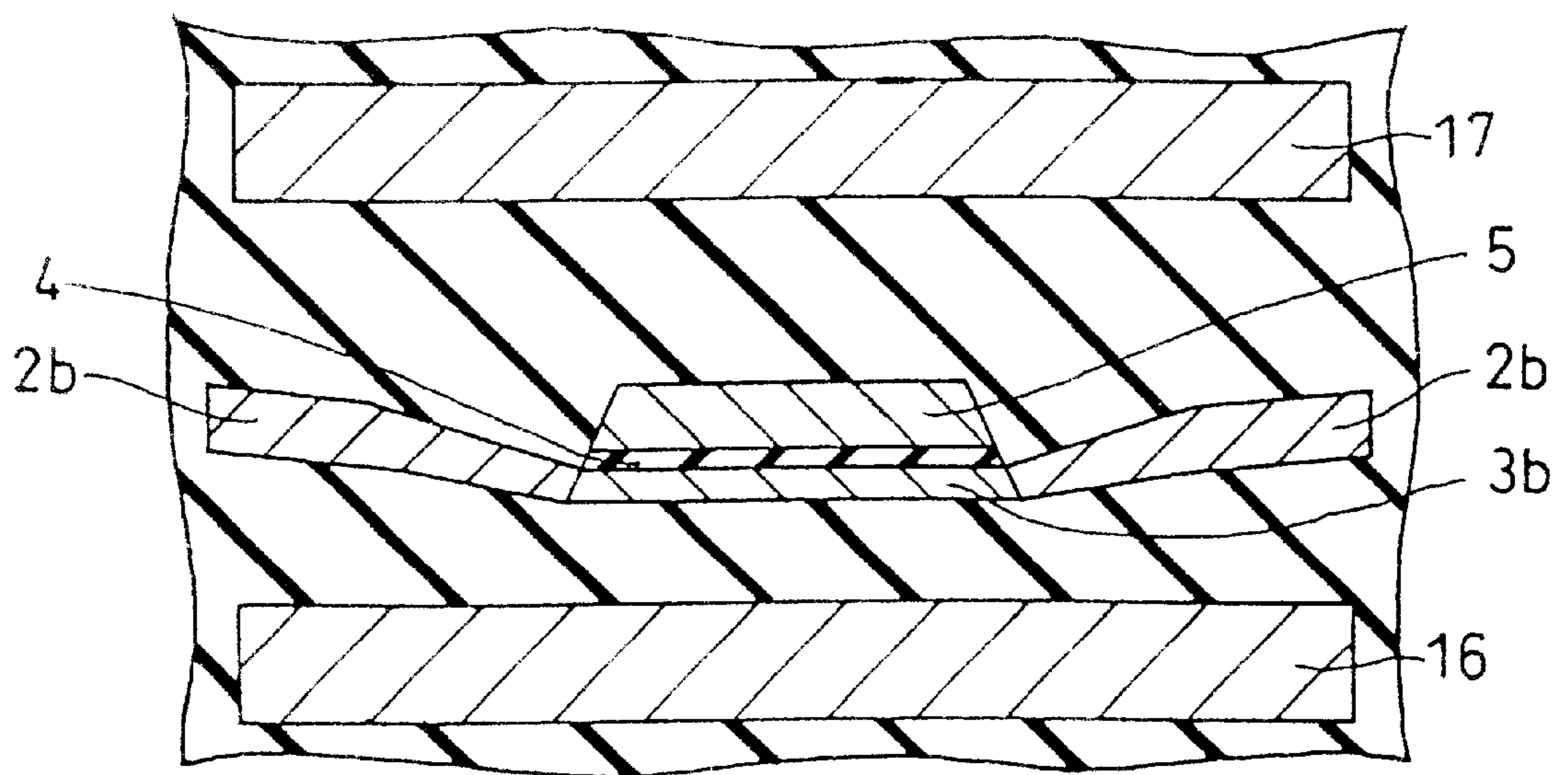
FIG. 3 (PRIOR ART)
