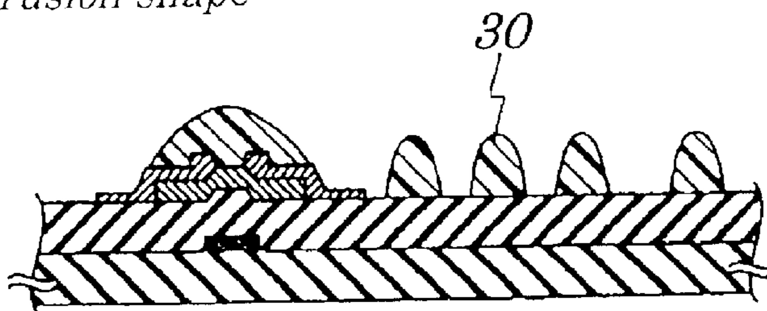
FIG.21G (PRIOR ART) smooth protrusion shape
