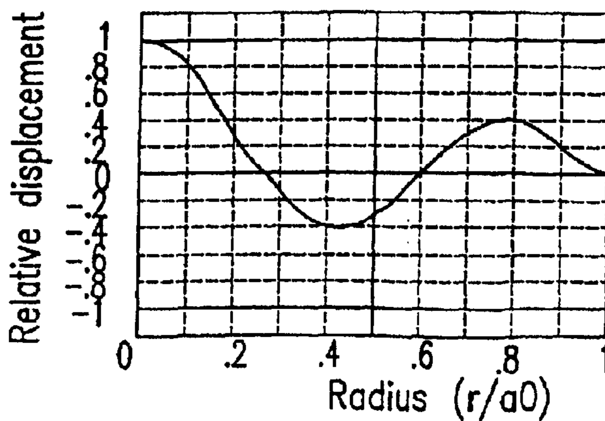
3rd resonance mode
