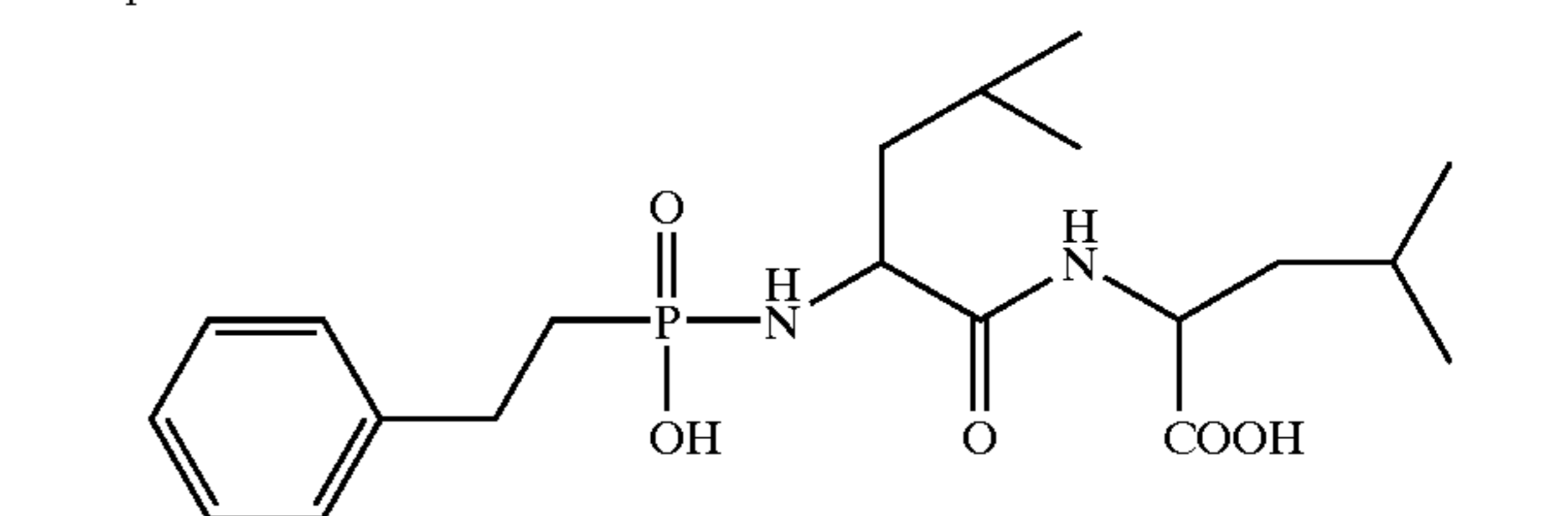
Compound 3:
