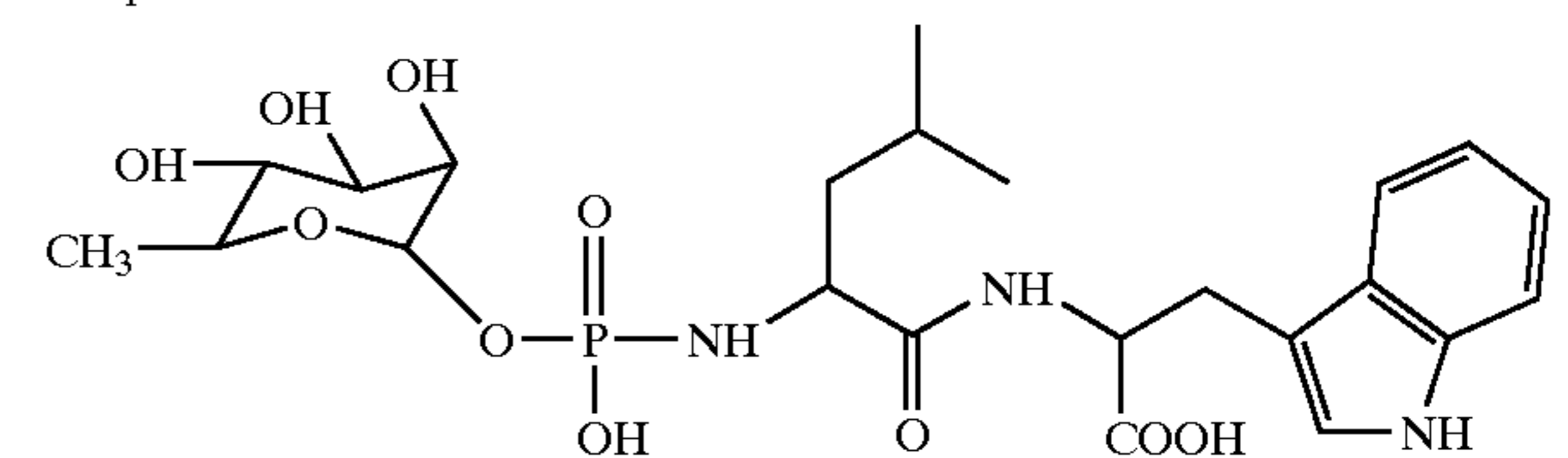
Compound 1:
