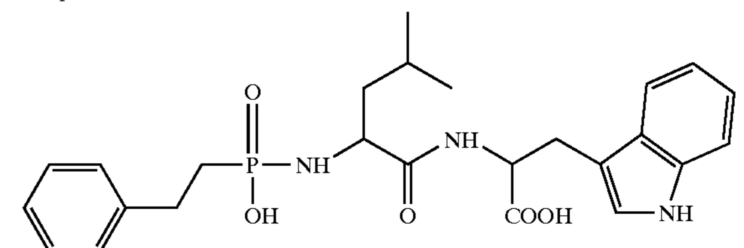
Compound 2:
