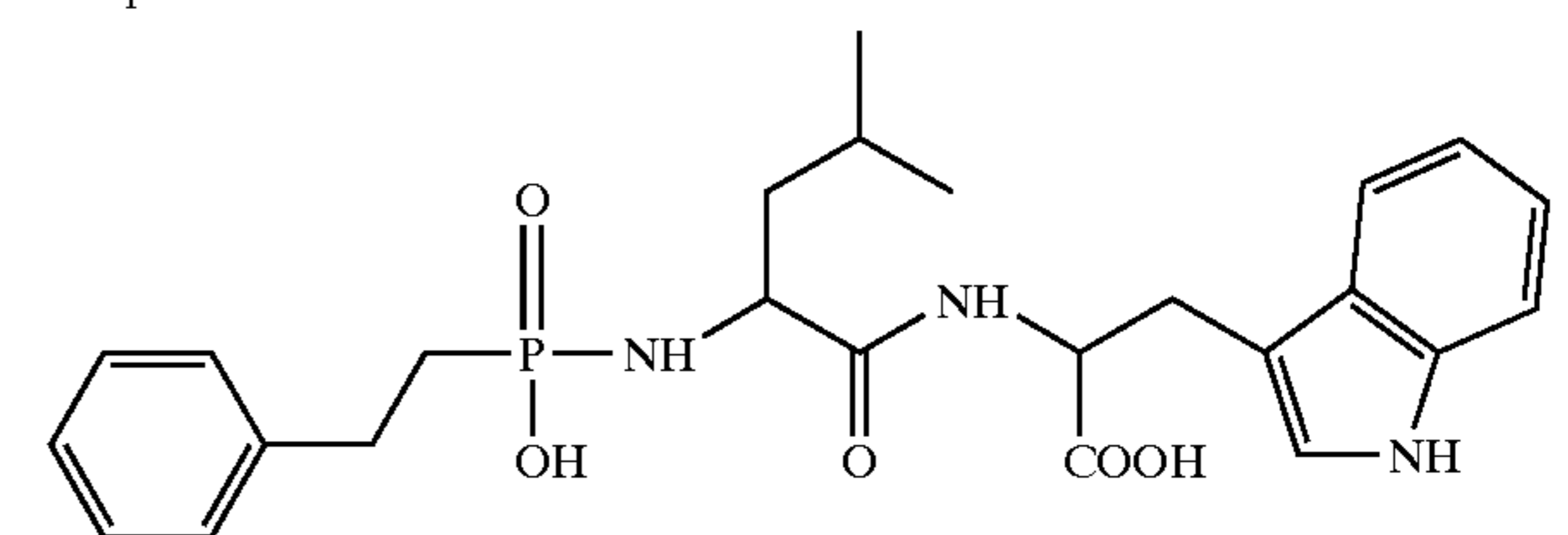
Compound 2:
