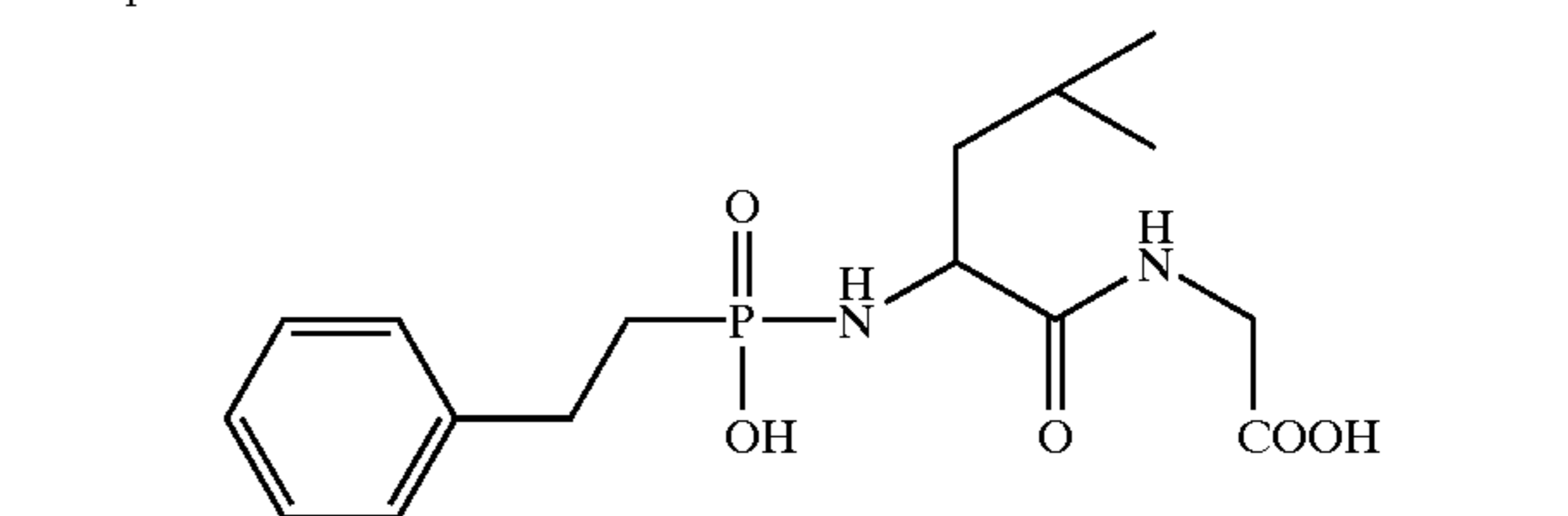
Compound 4:
