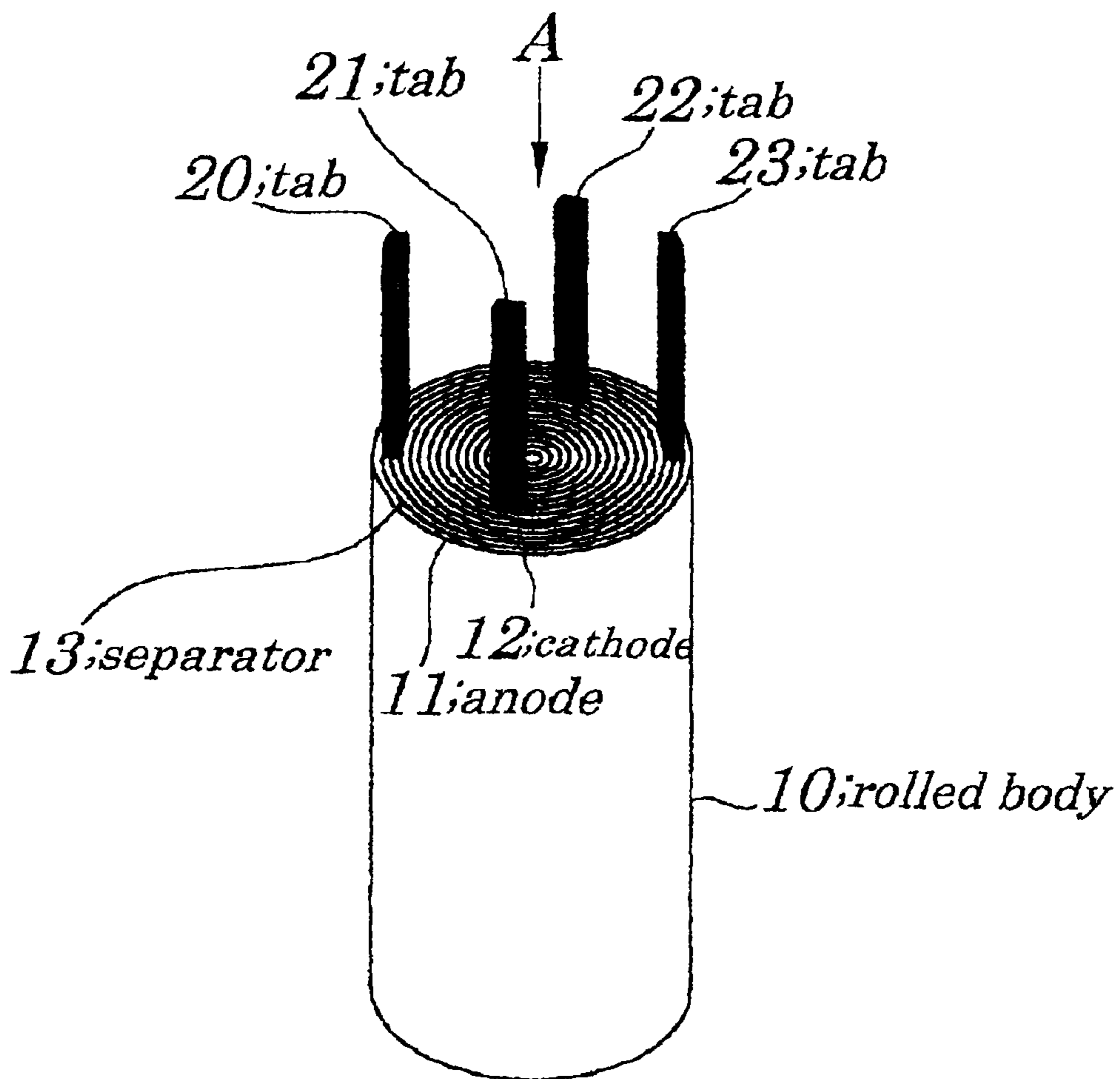
FIG. 12 (PRIOR ART)
