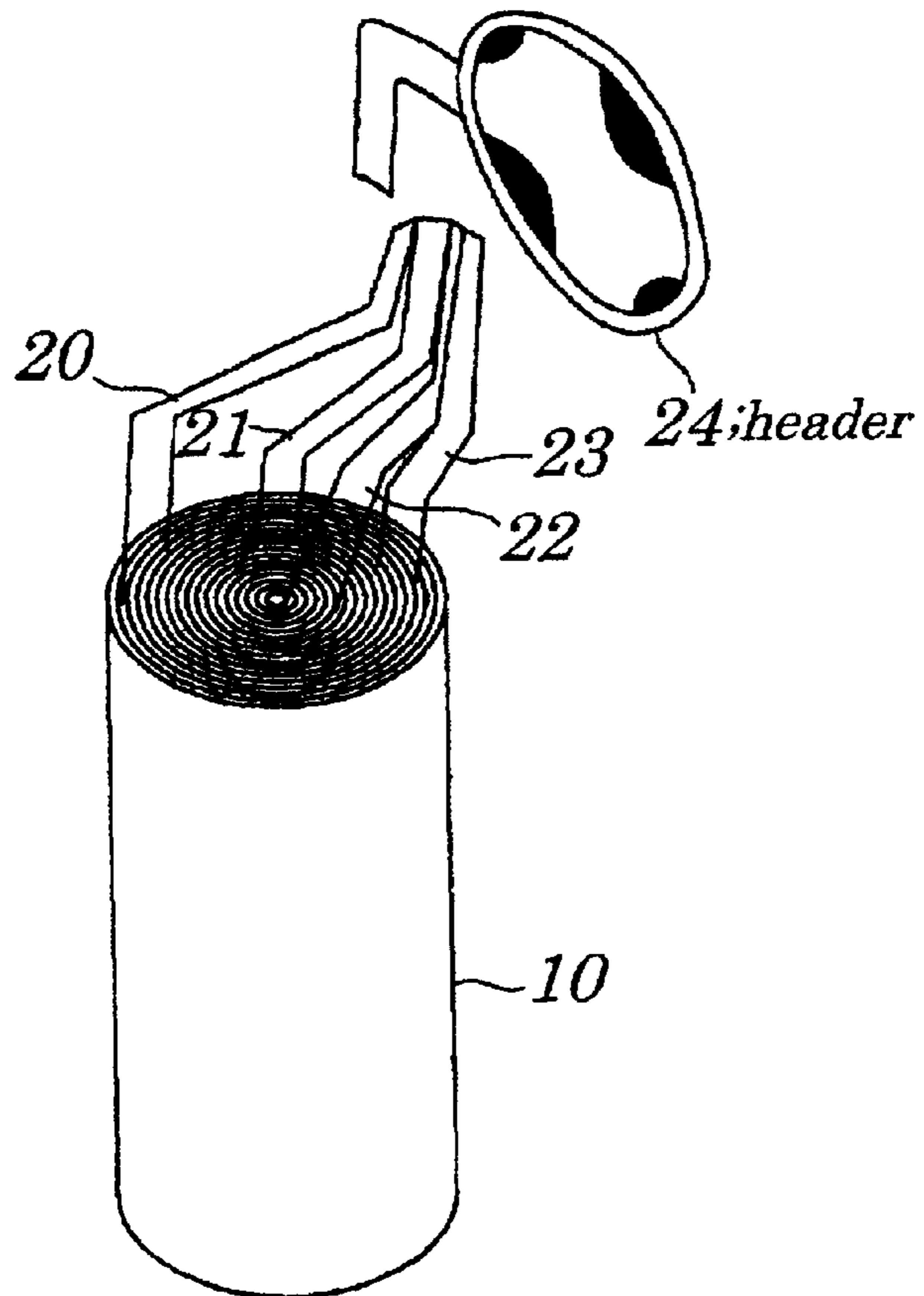
FIG. 22 (PRIOR ART)
