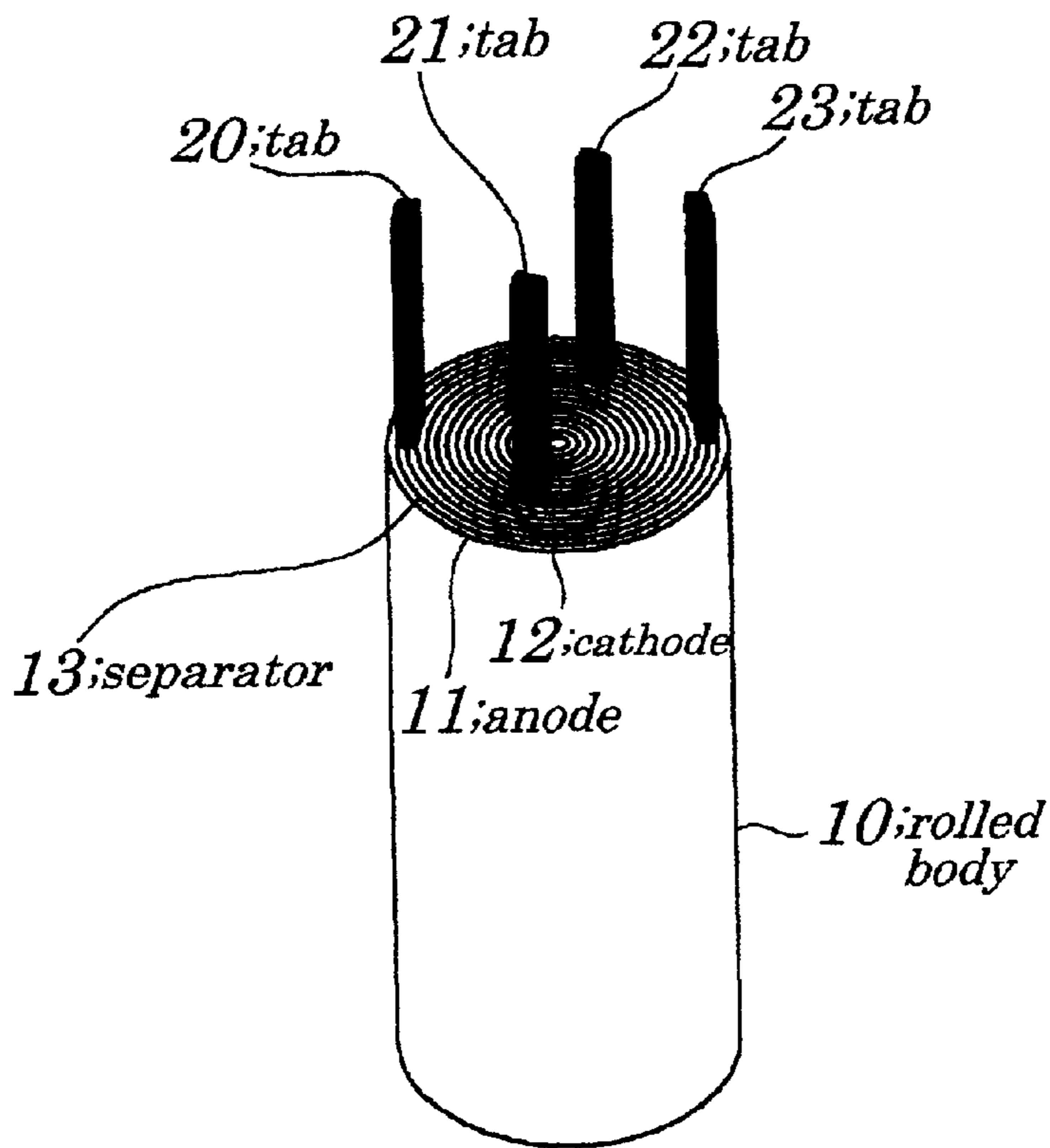
FIG. 20 (PRIOR ART)
