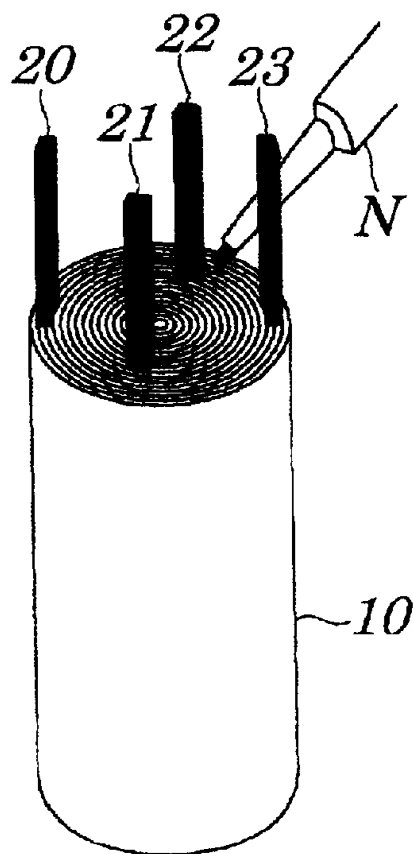
FIG. 22 (PRIOR ART)
